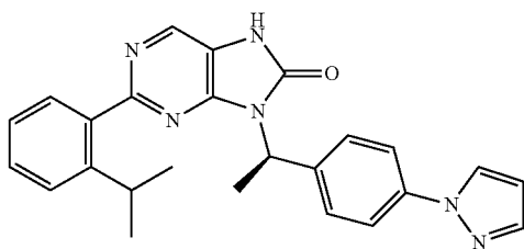
(R)-9-(1-(4-(1H-pyrazol-1-yl)phenylethyl)-2-(2-isopropylphenyl))-7,9-dihydro-8H-purin-8-one
