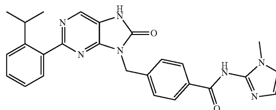
4-((2-(2-isopropylphenyl)-8-oxo-7,8-dihydro 8H-purin-8-yl)methyl)-N-(1-methyl-1H-imidazol-2-yl)benzamide
