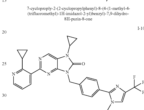
7-cyclopropyl-2-(2-cyclopropylpyridin-3-yl)-9-(4-(1-methyl-4-(trifluoromethyl)-1H-imidazol-2-yl)benzyl)-7,9-dihydro-8H-purin-8-one
