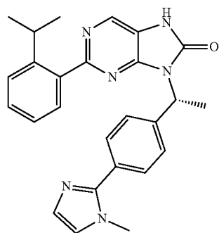
(R)-2-(2-isopropylphenyl)-8-(1-(4-(1-methyl-1H-imidazol-2-yl)phenyl)ethyl)-7,9-dihydro-8H-purin-8-one
