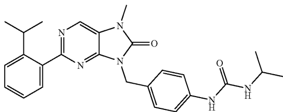
1-isopropyl-3-(4-((2-(2-isopropylphenyl)-7-methyl-8-oxo-7,8-dihydro-8H-purin-8-yl)methyl)phenyl)urea
