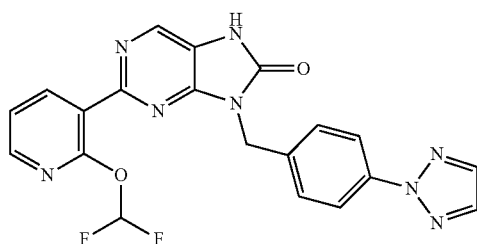
9-(4-(2H-1,2,3-triazol-2-yl)benzyl)-2-(2-(dihydromethoxy)pyridin-3-yl)-7,9-dihydro-8H-purin-8-one
