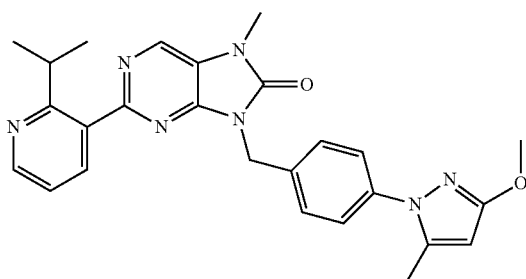
2-(2-isopropylpyridin-3-yl)-8-(4-(2-methoxy-5-methyl-1H-pyrazol-1-yl)benzyl)-7-methyl-7,8-dihydro-8H-purin-8-one
