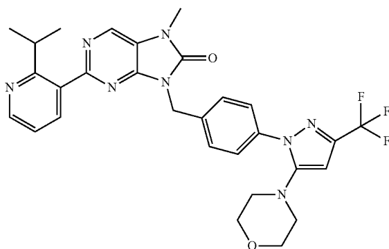
2-(2-isopropylpyridin-3-yl)-7-methyl-9-(4-(5-morpholine-3-(trifluoromethyl)-1H-pyrazol-1-yl)benzyl)-7,9-dihydro-8H-purin-8-one
