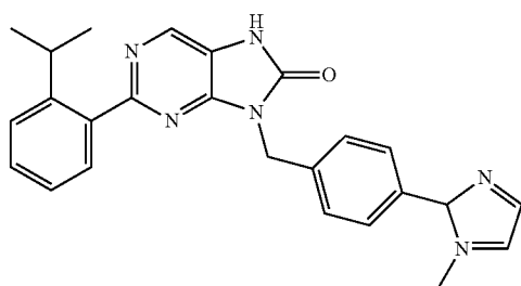
2-(2-isopropylphenyl)-9-(4-(5-methyl-1H-pyrazol-1-yl)benzyl)-7,9-dihydro-8H-purin-8-one
