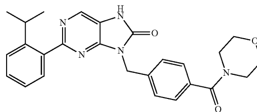
2-(2-isopropylphenyl)-8-(4-(morpholine-4-carbonyl)benzyl)-7,9-dihydro-8H-purin-8-one
