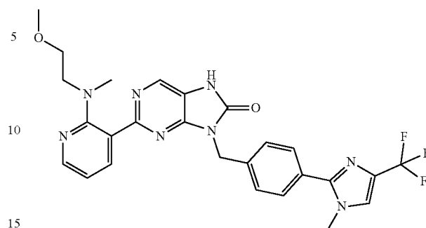
2-((2-methoxyethyl)(methylamino)pyridin-3-yl)-9-(4-(1-methyl-4-(trifluoromethyl)-1H-imidazol-2-yl)benzyl)-7,9-dihydro-8H-purin-8-one
