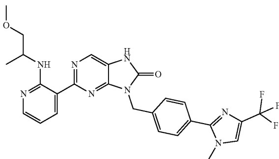
2-((1-methoxypropan-2-yl)amino)pyridin-3-yl)-8-(4-(1-methyl-4-(trifluoromethyl)-1H-imidazol-2-yl)benzyl)-7,9-dihydro-8H-purin-8-one
