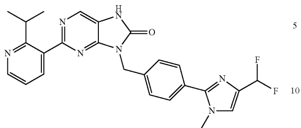
9-(4-(4-difluoromethyl-1-methyl-1H-imidazol-2-yl)benzyl)-2-(2-isopropylpyridin-3-yl)-7,9-dihydro-8H-purin-8-one
