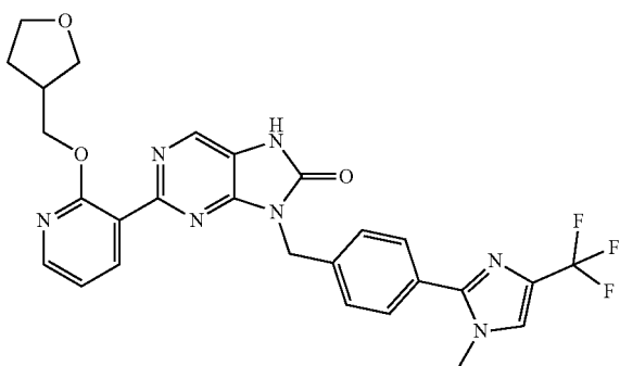
8-(4-(1-methyl-4-(trifluoromethyl)-1H-imidazol-2-yl)benzyl)-2-(2-((tetrahydrofuran-3-yl)methoxy)pyridin-3-yl)-7,9-dihydro-8H-purin-8-one
