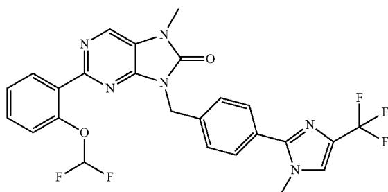
7-methyl-8-(4-(1-methyl-4-(trifluoromethyl)-1H-imidazol-2-yl)-2-benzyl)-2-(2-(trifluoromethoxy)phenyl)-7,9-dihydro-8H-purin-8-one
