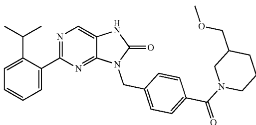
2-(2-isopropylphenyl)-8-((4-(3-(methoxymethyl)piperidine-1-carbonyl)benzyl)-7,9-dihydro 8H-purin-8-one
