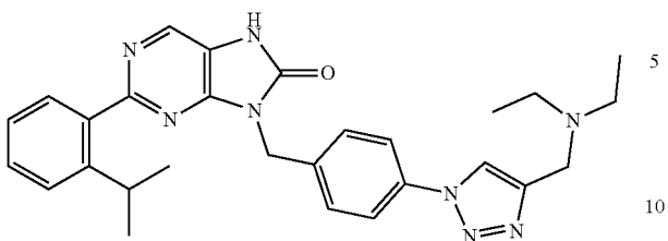
9-(4-(((diethylamino)methyl)-1H-1,2,3-triazol-1-yl)benzyl)-2-(2-isopropylphenyl)-7,8-dihydro-8H-purin-8-one
