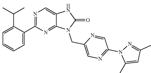
9-((5-(3,5-dimethyl-1H-pyrazol-1-yl)pyrazin-2-yl)methyl)-2-(2-isopropylphenyl)-7,9-dihydro-8H-purin-8-one
