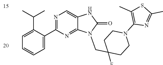
9-((1-(2,5-dimethylthiazol-4-yl)-4-fluoropiperidin-4-yl)methyl)-2-(2-isopropylphenyl)-7,9-dihydro-8H-purin-8-one
