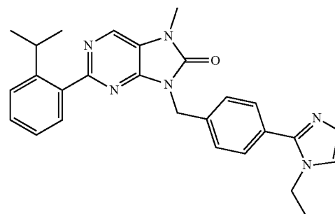
9-(4-(1-ethyl-1H-imidazol-2-yl(benzyl)-2-yl(benzyl)-2-(2-isopropylphenyl))-7-methyl-1,9-dihydro-8H-purin-8-one
