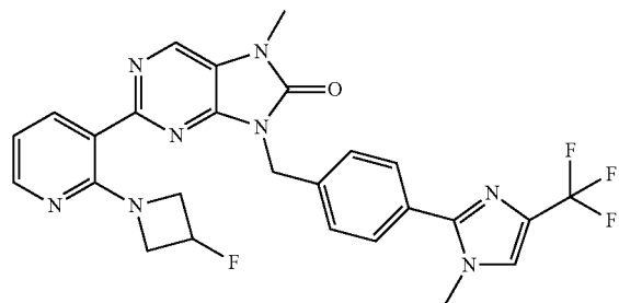
2-(2-(3-fluoroazetidin-1-yl)pyridin-3-yl)-7-methyl-9-(4-(1-methyl-4-(trifluoromethyl)-1H-imidazol-2-yl)benzyl)-7,9-dihydro-8H-purin-8-one
