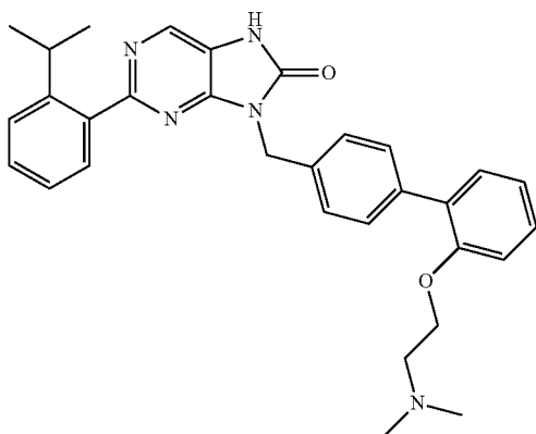
5-((2'-(2-(dimethylamino)ethoxy)-[1,1'-biphenyl]-4-yl)methyl)-2-(2-isopropylphenyl)-7-methyl-7,9-dihydro-8H-purin-8-one
