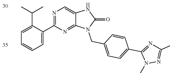
9-(4-(1,3-dimethyl-1H-1,2,4-triazol-5-yl)benzyl)-2-(2-isopropylphenyl)-7,9-dihydro-8H-purin-8-one
