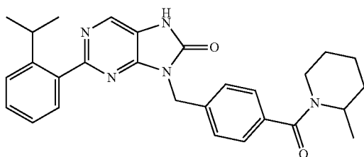
2-(2-isopropylphenyl)-9-(4-(2-methylpiperidine-1-carbonyl)benzyl)-7,9-dihydro-8H-purin-8-one
