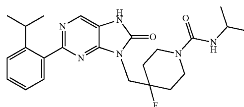
4-fluoro-N-isopropyl-4-((2-(2-isopropylphenyl)-8-oxo-7,8-dihydro-8H-purin-8-yl)methyl)piperidine-1-carboxamide
