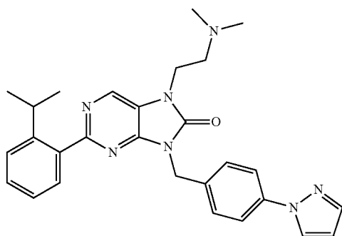
9-(4-(1H-pyrazol-2-yl)benzyl)-7-(2-(dimethylaminoethyl)-2-(2-isopropylphenyl)-7,9-dihydro-8H-purin-8-one
