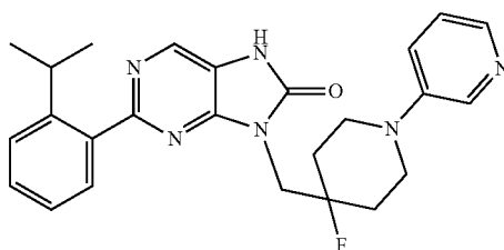
9-((4-fluoro-1-(pyridin-3-yl)piperidin-4-yl)methyl)-2-(2-isopropylphenyl)-7,8-dihydro-8H-purin-8-one
