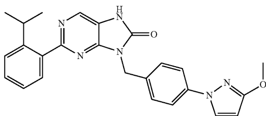
2-(2-isopropylphenyl)-9-(4-(3-methoxy-1H-pyrazol-1-yl)benzyl)-7,9-dihydro-8H-purin-8-one
