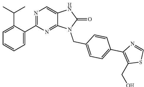
9-(4-(5-(hydroxymethyl)thiazol-4-yl)benzyl)-2-(2-isopropylphenyl)-7,9-dihydro-8H-purin-8-one
