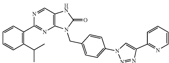
2-(2-isopropylphenyl)-9-(4-(4-(pyridin-2-yl)-1H-1,2,3-triazol-1-yl)benzyl)-7,9-dihydro-8H-purin-8-one
