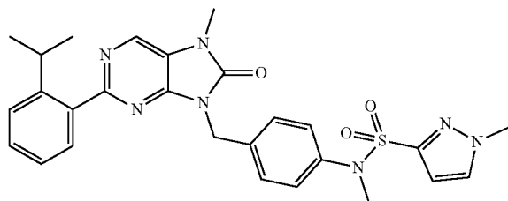
N-((4-((2-(2-isopropylphenyl)-7-methyl-8-oxo-7,8-dihydro-8H-purin-8-yl)methyl)phenyl)-N-1-dimethyl-1H-pyrazole-3-sulfonamide
