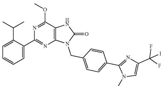
2-(2-isopropylphenyl)-6-methoxy-9-(4-(1-methyl-4-(trifluoromethyl)-1H-imidazol-2-yl)benzyl)-7,9-dihydro-8H-purin-8-one
