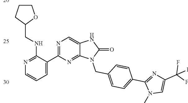
8-(4-(1-methyl-4-(trifluoromethyl)-1H-imidazol-2-yl)benzyl)-2-((2-(tetrahydrofuran-2-yl)methyl)amino)pyridin-3-yl)-7,9-dihydro-8H-purin-8-one
