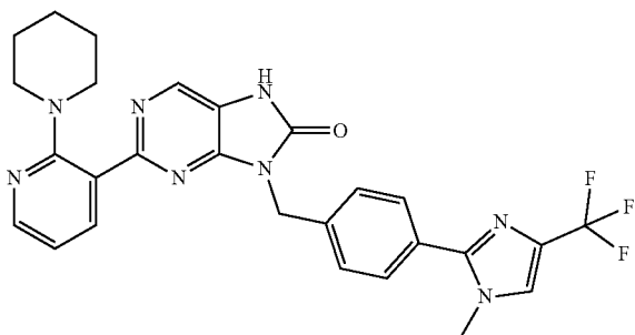
9-(4-(1-methyl-4-(trifluoromethyl)-1H-imidazol-2-yl)benzyl)-2-(2-(piperidin-1-yl)pyridin-3-yl)-7,9-dihydro-8H-purin-8-one
