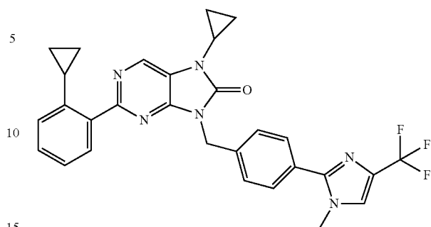
7-cyclopropyl-2-(2-cyclopropylphenyl)-8-(4-(1-methyl-4-(trifluoromethyl)-1H-imidazol-2-yl)benzyl)-7,9-dihydro-8H-purin-8-one
