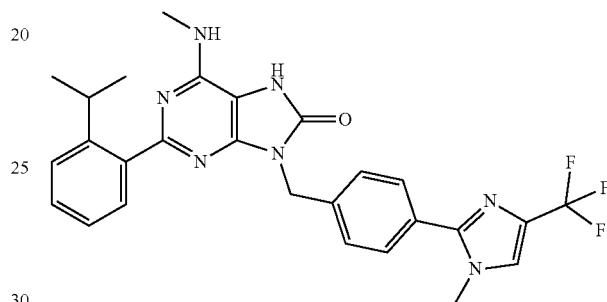
2-(2-(isopropylphenyl)-9-(4-(1-methyl-4-(trifluoromethyl)-1H-imidazol-2-yl)benzyl)-8-(methylamino)-7,9-dihydro-8H-purin-8-one
