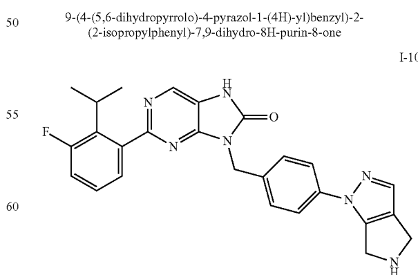
9-(4-(5,6-dihydropyrrolo)-[3,4-o]pyrazol-(4H-yl)benzyl)-2-(3-fluoro-2-isopropylphenyl)-7,9-dihydro-8H-purin-8-one
