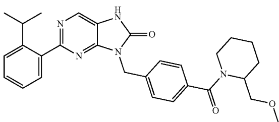
2-(2-isopropylphenyl)-9-(4-(2-methoxymethyl)piperidine-1-carbonyl)benzyl)-7,8-dihydro-8H-purin-8-one
