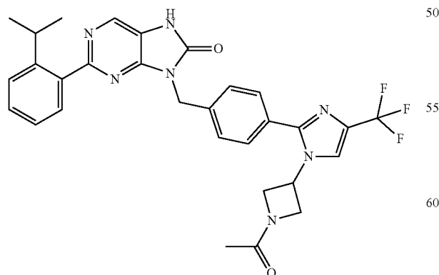
9-(4-(1-(1-acetylazetidin-3-yl)-4-(trifluoromethyl)-1H-imidazol- 2-yl)benzyl)-2-(2-isopropylphenyl)-7,9-dihydro-8H-purin-8-one
