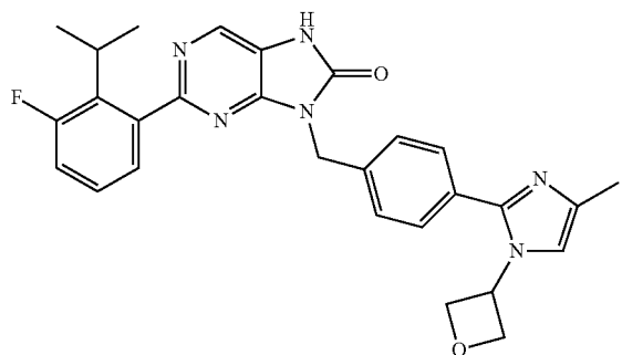
2-(3-fluoro-2-isopropylphenyl)-8-(4-(4-methyl-1-(oxetan-3-yl)-1H-imidazol-2-yl)benzyl)-7,9-dihydro-8H-purin-8-one
