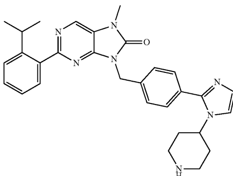
2-(2-isopropylphenyl)-7-methyl-8-(4-(1-(piperidin-4-yl)-1H-imidazol-2-yl(benzyl))-7,9-dihydro-8H-purin-8-one
