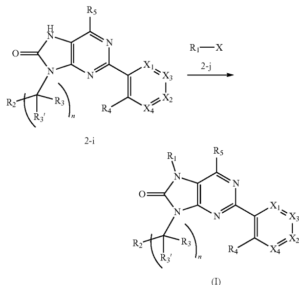
General Scheme 3
