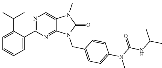
3-isopropyl-1-(4-((2-(2-isopropylphenyl)-7-methyl-8-oxo-7,8-dihydro-8H-purin-8-yl)methyl)phenyl)-1-methylurea
