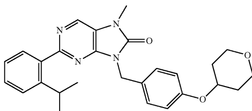
2-(2-isopropylphenyl)-7-methyl-8-(4-((tetrahydro-2H-pyran-4-yl)oxy)benzyl)-7,9-dihydro-8H-purin-8-one
