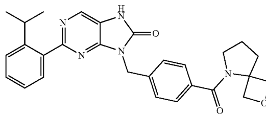
8-(4-(2-oxa-5-azaspiro[3,4]octane-5-carbonyl)benzyl)-2-(2-isopropylphenyl)-7,8-dihydro-8H-purin-8-one
