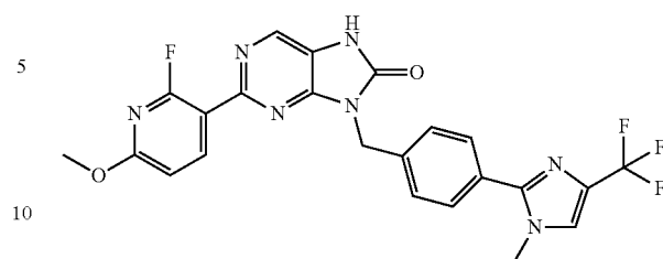
2-(2-fluoro-8-methoxypyridin-3-yl)-8-(4-(t-methyl-4-(trifluoromethyl)-1H-imidazol-2-yl)benzyl)-7,9-dihydro-8H-purin-8-one
