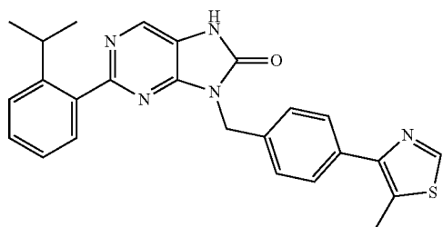
2-(2-isopropylphenyl)-9-(4-(5-methylthiazol-4-yl)benzyl)-7,9-dihydro-8H-purin-8-one
