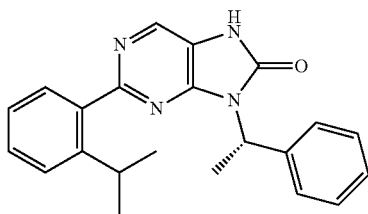
(S)-2-(2-isopropylphenyl)-8-(1-phenylethyl)-7,9-dihydro-8H-purin-8-one
