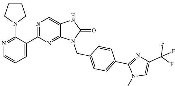
9-(4-(1-methyl-4-(trifluoromethyl)-1H-imidazol-2-yl)benzyl)-2-(2-(pyrrolidin-1-yl)pyridin-3-yl)-7,9-dihydro-8H-purin-8-one
