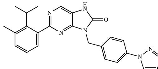
9-(4-(1H-pyrazol-1-yl)benzyl)-2-(2-isopropyl-3-methylphenyl)-7,9-dihydro-8H-purin-8-one
