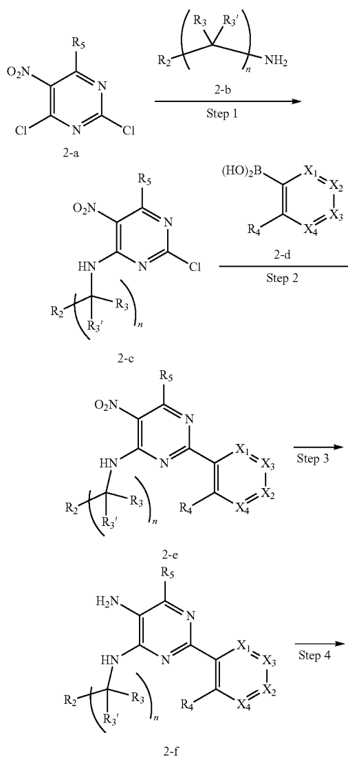
General Scheme 1
