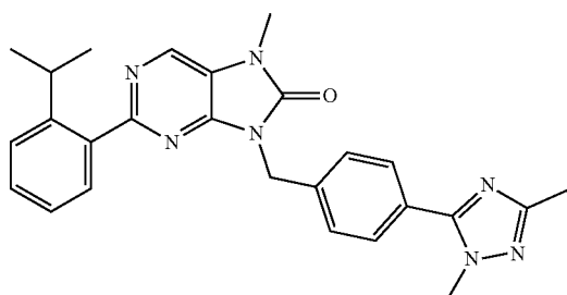
9-(4-(1,3-dimethyl-1H-1,2,4-triazol-5-yl)benzyl)-2-(2-isopropylphenyl)-7-methyl-7,9-dihydro-8H-purin-8-one
