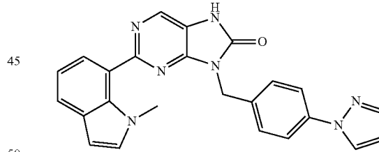
9-(4-(1H-pyrazol-1-yl)benzyl)-2-(1-methyl-1H-imidazol-7-yl)-7,8-dihydro-8H-purin-8-one
