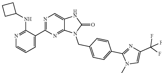
2-(2-cyclobutylamino)pyridin-3-yl)-8-(4-(1-methyl-4-(trifluoromethyl)-1H-imidazol-2-yl)benzyl)-7,9-dihydro-8H-purin-8-one
