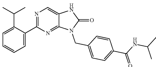
N-isopropyl-4-((2-(2-isopropylphenyl)-8-oxo-7,8-dihydro-8H-purin-8-yl)methyl)benzamide
