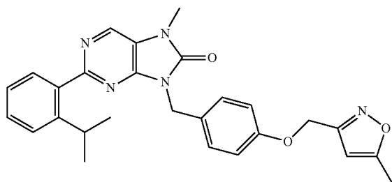
2-(2-isopropylphenyl)-7-methyl-8-(4-((5-methylisoxazi-3-yl)methoxy)benzyl)-7,9-dihydro-8H-purin-8-one
