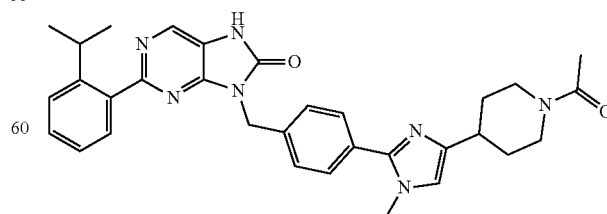
9-(4-(4-(1-acetylpiperidin-4-yl)-1-methyl-1H-imidazol-2-yl)benzyl)-2-(2-isopropylphenyl)-7,9-dihydro-8H-purin-8-one
