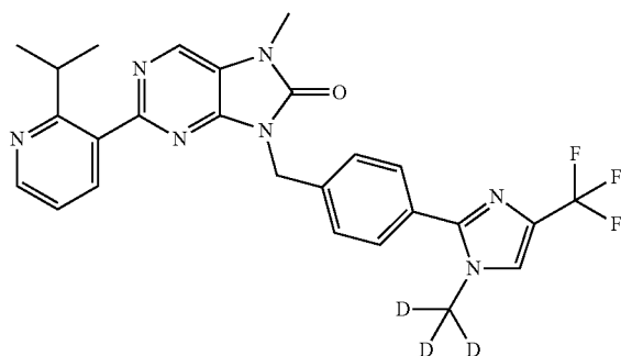
2-(2-isopropylpyridin-3-yl)-7-methyl-9-(4-(1-(methyl-d 3 )-4-(trifluoromethyl)-1H-imidazol-2-yl)benzyl)-7,9-dihydro-8H-purin-8-one
