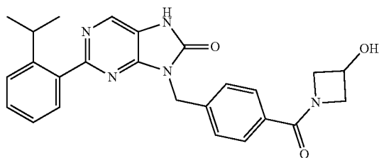
9-4-(3-hydroxyazetidine-1-carbonylbenzyl)-2-(2-isopropylphenyl)-7,8-dihydro-8H-purin-8-one
