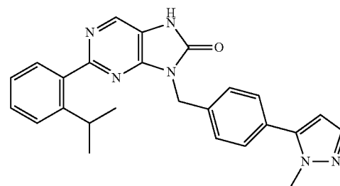
2-(2-isopropylphenyl)-9-(4-(1-methyl-1H-pyrazol-5-yl)benzyl)-7,9-dihydro-8H-purin-8-one
