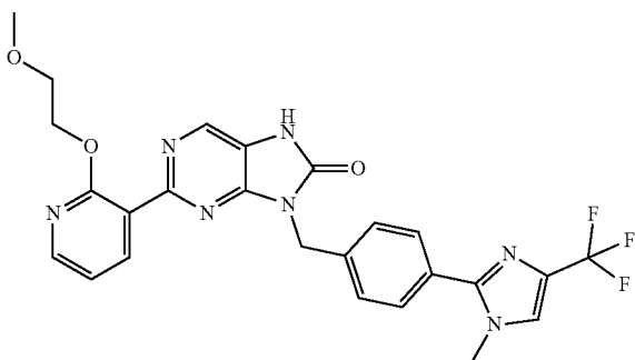
2-(2-(2-methoxyethoxy)pyridin-3-yl)-9-(4-(1-methyl-4-(trifluoromethyl)-1H-imidazol-2-yl)benzyl)-7,9-dihydro-8H-purin-8-one
