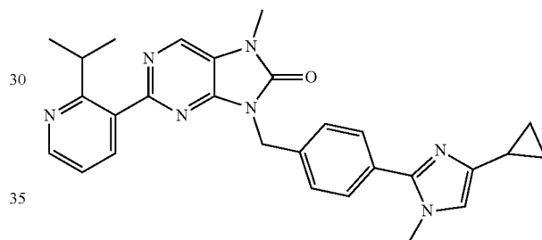
9-(4-(4-cyclopropyl-1-methyl-1H-imidazol-2-yl)benzyl)-2-(2-isopropylpyridin-3-yl)-7-methyl-7,9-dihydro-8H-purin-8-one
