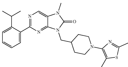
9-((1-(2,5-dimethylthiazol-4-yl)piperidin-4-yl)methyl)-2-(2-isopropylphenyl)-7-methyl-7,9-dihydro-8H-purin-8-one
