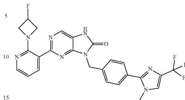
2-(2-(3-fluoroazetidin-1-yl)pyridin-3-yl)-9-(4-(1-methyl-4-(trifluoromethyl)-1H-imidazol-2-yl)benzyl)-7,9-dihydro-8H-purin-8-one
