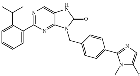
9-(4-(5-fluoro-1-methyl-1H-imidazol-2-yl)benzyl)-2-(2-isopropylphenyl)-7,8-dihydro-8H-purin-8-one
