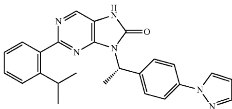
(S)-8-(1-(4-(1H-pyrazol-1-yl)phenylethyl)-2-(2-isopropylphenyl))-7,9-dihydro-8H-purin-8-one
