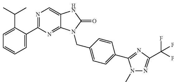
2-(2-isopropylphenyl)-9-(4-(1-methyl-3-(trifluoromethyl)-1H-1,2,4-triazol-5-yl)-benzyl)-7,9-dihydro-8H-purin-8-one
