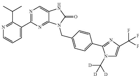
2-(2-isopropylpyridin-3-yl)-9-(4-(1-methyl-d3)-4-(trifluoromethyl)-1H-imidazol-2-yl)benzyl)-7,9-dihydro-8H-purin-8-one
