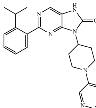
2-(2-isopropylphenyl)-8-(4-(pyridin-3-yl)piperidin-4-yl)-7,9-dihydro-8H-purin-8-one
