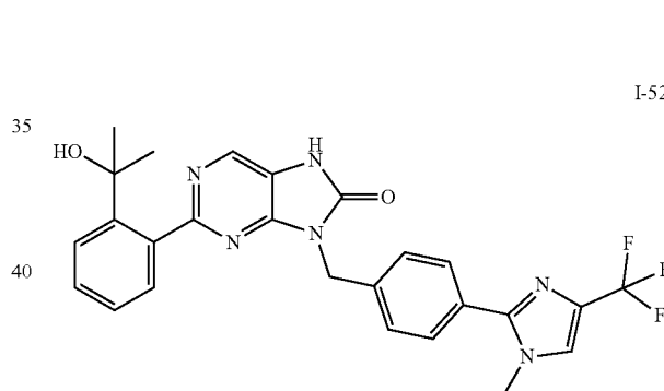
2-(2-(hydroxypropan-2-yl)phenyl)-9-(4-(1-benzyl-4-trifluoromethyl)-1H-imidazol-2-yl)benzyl)-7,9-dihydro-8H-purin-8-one
