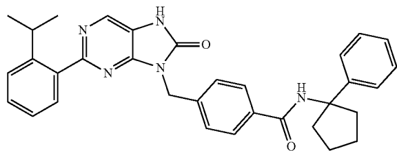
4-((2-(2-isopropylphenyl)-8-oxo-7,8-dihydro-9H-purin-8-yl)methyl)-N-(1-phenylcyclopentyl)benzamide
