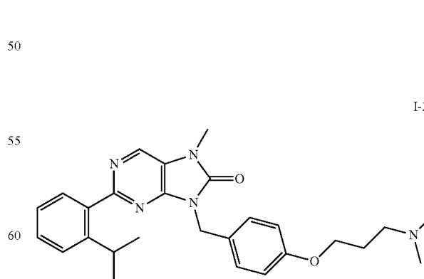
9-(4-(3-(dimethylamino)propyl)methoxy)benzyl)-2-(2- isopropylphenyl)-7-methyl-7,9-dihydro-8H-purin-8-one
