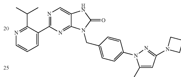
8-(4-(3-(azetidin-1-yl)-5-methyl-1H-pyrazol-1-yl)benzyl)-2-(2-isopropylpyridin-2-yl)-7,9-dihydro-8H-purine-8-one
