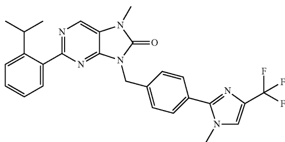
2-(2-isopropylphenyl)-7-methyl-5-(4-(1-methyl-4-(trifluoromethyl)-1H-imidazol-2-yl)benzyl)-7,9-dihydro-8H-purin-8-one
