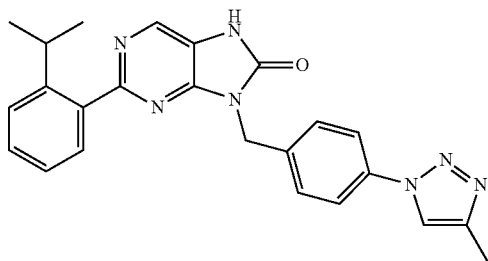
2-(2-isopropylphenyl)-9-(4-(4-methyl-1H-1,2,3-triazol-1-yl)benzyl)-7,9-dihydro-8H-purin-8-one
