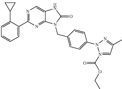
ethyl 1-(4-((2-(2-cyclopropylphenyl)-8-oxo-7,9-dihydro-9H-purin-9-yl)methyl)phenyl)-3-methyl-1H-pyrazol-5-oate
