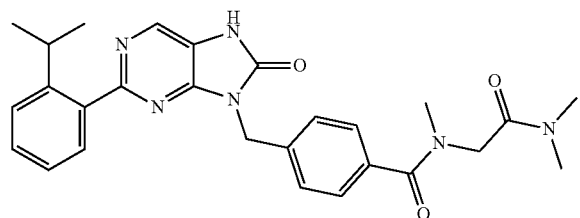
N-(2-(dimethylamino)-2-oxoethyl)-4-((2-(2-isopropylphenyl)-8-oxo-7,8-dihydro-8H-purin-8-yl)methyl)-N-methylbenzamide
