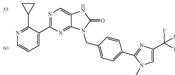
2-(2-cyclopropylpyridin-3-yl)-3-(4-(1-methyl-4-trifluoromethyl)-1H-imidazol-2-yl)benzyl-7,5-dihydro-3H-purin-8-one
