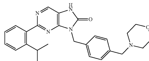
2-(2-isopropylphenyl)-8-(4-(morpholinomethyl)benzyl)-7,8-dihydro-8H-purin-8-one
