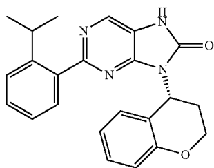
(R)-8-(chroman-4-yl)-2-(2-isopropylphenyl)-7,9-dihydro-8H-purin-8-one
