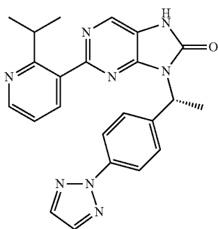
(R)-8-(1-(4-(2H-1,2,3-triazol-2-yl)phenyl)ethyl)-2-(2-isopropylphenyl)-7,9-dihydro-8H-purin-8-one
