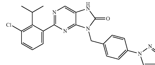
9-(4-(1H-pyrazol-1-yl)benzyl)-2-(3-chloro-2-isopropylphenyl)-7,9-dihydro-8H-purin-8-one
