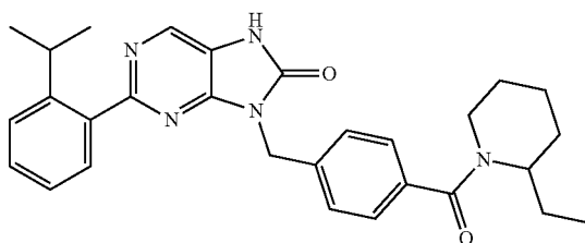
9-(4-(2-ethylpiperidine-1-carbonyl)benzyl)-2-(2-isopropylphenyl)-7,9-dihydro-8H-purin-8-one
