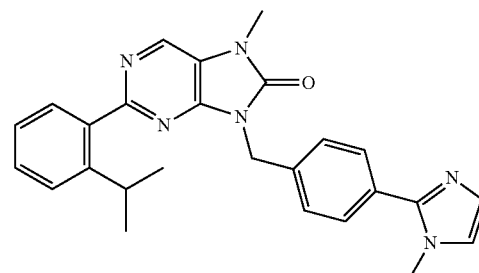
2-(2-isopropylphenyl)-7-methyl-8-(4-(1-methyl-1H-imidazol-2-yl)benzyl)-7,9-dihydro-8H-purin-8-one
