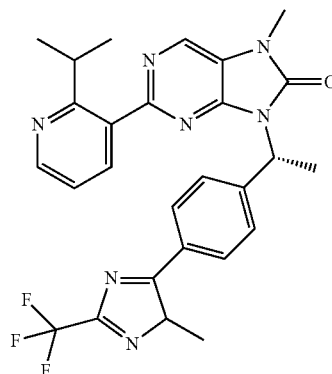
(R)-2-(2-isopropylpyridin-3-yl)-7-methyl-9-(1-(4-(1-methyl-4-(trifluoromethyl)-1H-imidazol-2-yl)phenyl)ethyl)-7,9-dihydro-8H-purin-8-one
