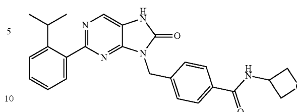
4-((2-(2-isopropylphenyl)-8-oxo-7,8-dihydro-8H-purin-8-yl)methyl)-N-(oxetan-3-yl)benzamide
