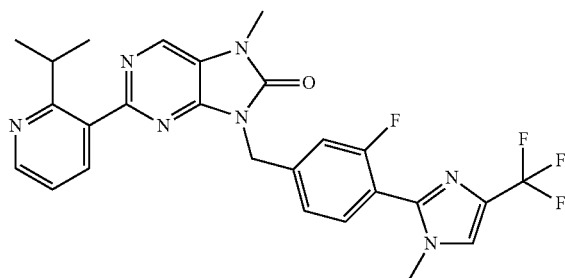
9-(3-fluoro-4-(1-methyl-4-(trifluoromethyl)-1H-imidazol-2-yl)-benzyl)-2-(2-isopropylpyridin-3-yl)-7-methyl-7,9-dihydro-8H-purin-8-one
