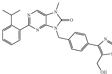
8-(4-(5-(hydroxymethyl)thiazol-4-yl)benzyl)-2-(2-isopropylphenyl)-7-methyl-7,9-dihydro-8H-purin-8-one
