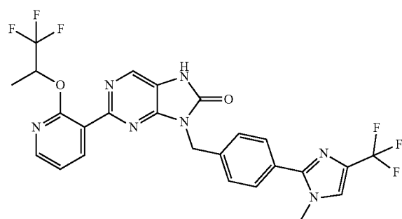
9-(4-(1-methyl-4-(trifluoromethyl)-1H-imidazol-2-yl)benzyl)-2-(2-((1,1,1-trifluoropropan-2-yl)oxy)pyridin-3-yl)-7,8-dihydro-8H-purin-8-one
