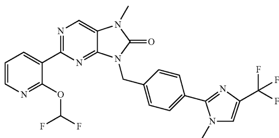
2-(2-(difluoromethoxy)pyridin-3-yl)-7-methyl-9-(4-(trifluoromethyl)-1H-imidazol-2-yl)benzyl)-7,3-dihydro-8H-purin-8-one
