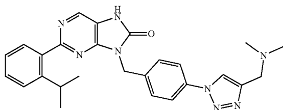
9-(4-(4-((dimethylamino)methyl)-1H-1,2,3-triazol-1-yl)benzyl)-2-(2-isopropylphenyl)-7,9-dihydro-8H-purin-8-one
