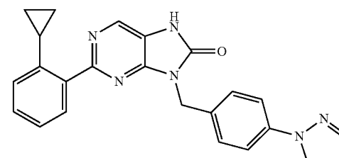
9-(4-(1H-pyrazol-1-yl)benzyl)-2-(2-cyclopropylphenyl)-7,9-dihydro-8H-purin-8-one
