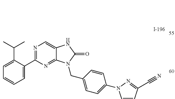
1-(4-((2-(2-isopropylphenyl)-8-oxo-7,9-dihydro-9H-purin-9-yl)methyl)phenyl)-1H-pyrazole-3-carbonitrile
