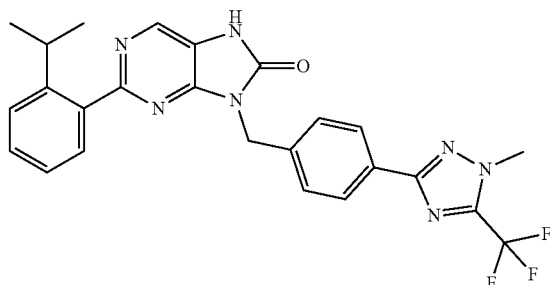
2-(2-isopropylphenyl)-8-(4-(1-methyl-5-(trifluoromethyl)-1H-1,2,4-triazol-3-yl)benzyl)-7,9-dihydro-8H-purin-8-one
