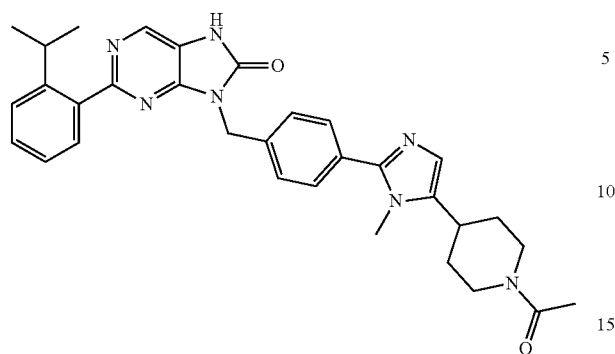
9-(4-(5-(1-acetylpiperidin-4-yl)-1-methyl-1H-imidazol-2-yl)benzyl)- 2-(2-isopropylphenyl)-7,9-dihydro-8H-purin-8-one
