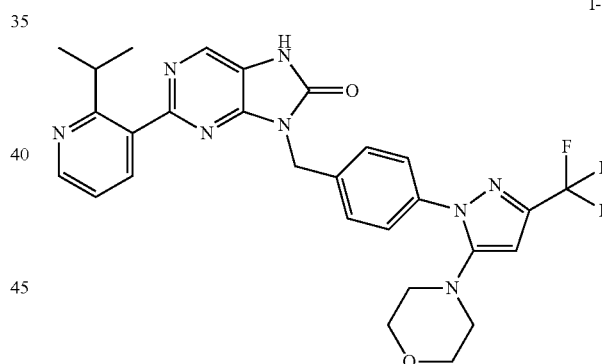
2-(2-isopropylpyridin-3-yl)-8-(4-(5-morpholino-3-(trifluoromethyl)-1H-pyrazol-1-yl)benzyl)-7,9-dihydro-8H-purin-8-one
