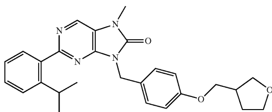
2-(2-isopropylphenyl)-7-methyl-9-(4-((tetrahydrofuran-3-yl) methoxy)benzyl)-7,9-dihydro-8H-purin-8-one
