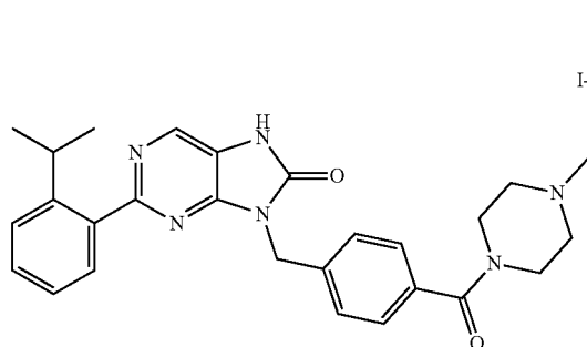
2-(2-isopropylphenyl)-8-(4-(4-methylpiperazine-1-carbonyl)benzyl)-7,8-dihydro-8H-purin-8-one
