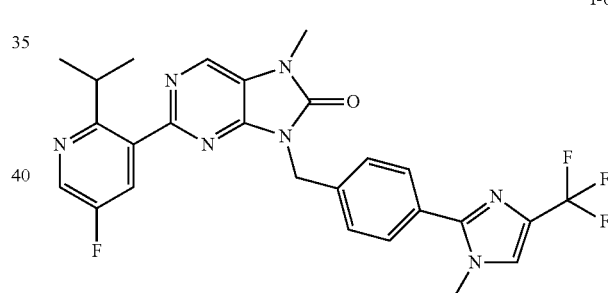
2-(5-fluoro-2-isopropylpyridin-3-yl)-7-methyl-9-(4-(1-methyl-4-(trifluoromethyl)-1H-imidazol-2-yl)benzyl)-7,9-dihydro-8H-purin-8-one
