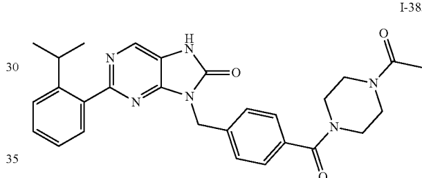
8-(4-(4-acetypiperazine-1-carbonylbenzyl)-2-(2-isopropylphenyl)-7,8-dihydro-8H-purin-8-one
