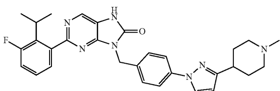
2-(3-fluoro-2-isopropylphenyl)-8-(4-(3-(1-methylpiperidin-4-yl)-1H-pyrazol-1-yl)benzyl)-7,8-dihydro-8H-purin-8-one
