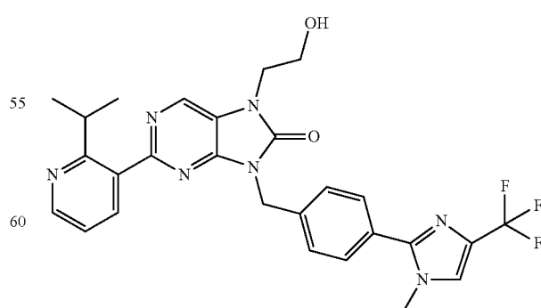
7-(2-hydroxyethyl)-2-(2-isopropylpyridin-3-yl)-3-(4-(1-methyl-4-(trifluoromethyl)-1H-imidazol-2-yl)benzyl)-7,8-dihydro-8H-purin-8-one
