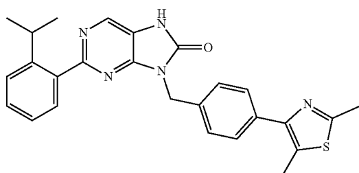
9-(4-(2,5-dimethylthiazol-4-yl)benzyl)-2-(2-isopropylphenyl)-7,9-dihydro-8H-purin-8-one
