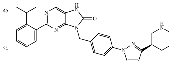
(R)-2-(2-isopropylphenyl)-9-(4-(3-(piperidin-3-yl)-1H-pyrazol-1-yl)-benzyl)-7,9-dihydro-9H-purin-8-one
