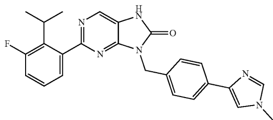
2-(3-fluoro-2-isopropylphenyl)-9-(4-(1-methyl-1H-imidazol-4-yl)benzyl)-7,9-dihydro-8H-purin-8-one
