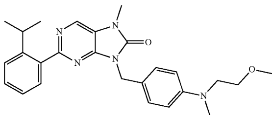
2-(2-isopropylphenyl)-8-((2-methoxyethyl(methyl)amino)benzyl)-7-methyl-7,9-dihydro-8H-purin-8-one
