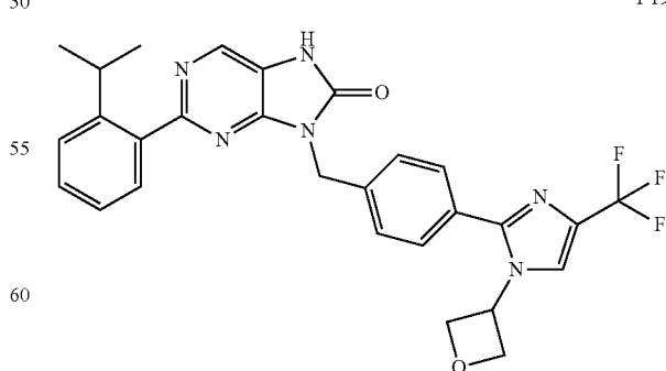
2-(2-isopropylphenyl)-8-(4-(1-(oxetan-3-yl)-4-(trifluoromethyl)-1H-imidazol-2-yl)benzyl)-7,9-dihydro-8H-purin-8-one
