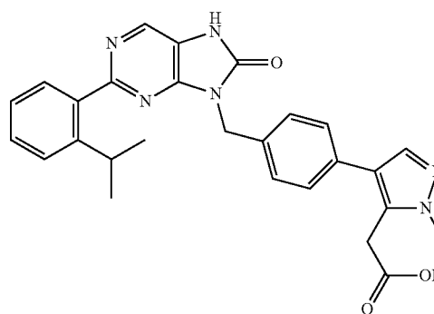
2-(4-(4-((2-(2-isopropoxy(methyl)-6-oxo-7,6-dihydro-9H-purin-9-yl)methyl)phenyl)-1-methyl-1H-pyrazol-5-yl)acetic acid
