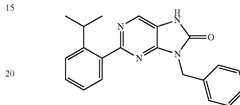
5-benzyl-2-(2-isopropylphenyl)-7,9-dihydro-8H-purin-8-one
