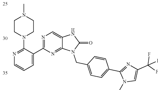
9-(4-(1-methyl-4-(trifluoromethyl)-1H-imidazol-2-yl)benzyl)-2-(2-(4-methylpiperazin-1-yl)pyridin-3-yl)-7,8-dihydro-8H-purin-8-one
