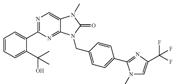
2-(2-(2-methyl)propan-2-yl)phenyl)-7-methyl-9-(4-(1-methyl-4-(trifluoromethyl)-1H-imidazol-2-yl)benzyl)-7,9-dihydro-8H-purin-8-one
