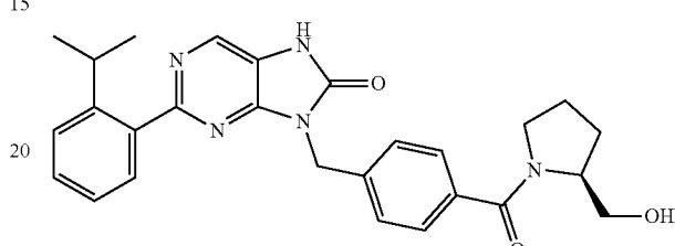
(S)-8-(4-(2-hydroxymethyl)pyrrolidine-1-carbonylbenzyl)-2-(2-isopropylphenyl)-7,8-dihydro-8H-purin-8-one
