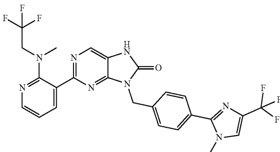
2-(2-(methyl(2,2,2-trifluoroethyl)amino)pyridin-3-yl)-9-(4-(1-methyl-4-(trifluoromethyl)-1H-imidazol-2-yl)benzyl)-7,9-dihydro-8H-purin-8-one
