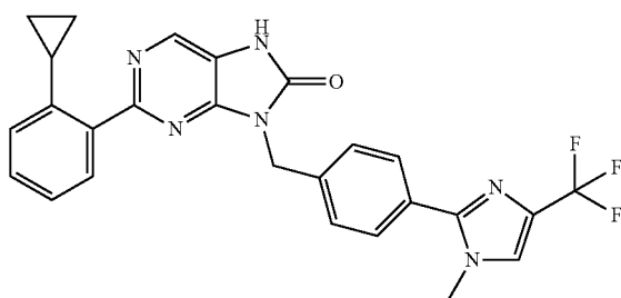
2-(2-cyclopropyl(phenyl)-3-(4-(1-methyl-4-(trifluoromethyl)-1H-imidazol-2-yl)benzyl)-7,9-dihydro-8H-purin-8-one
