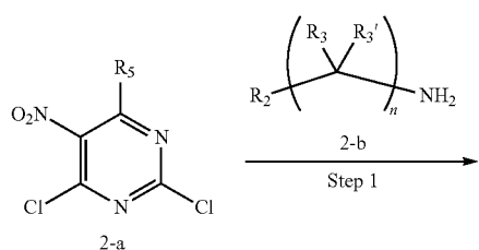
General Scheme 2
