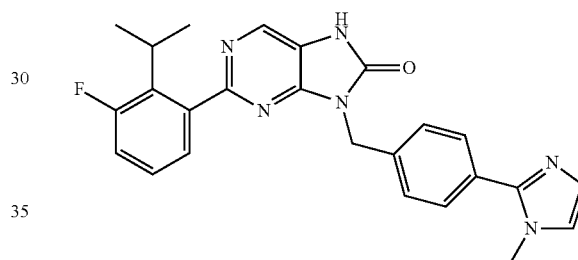
2-(3-fluoro-2-isopropylphenyl)-3-(4-(1-methyl-1H-imidazol-2-yl)benzyl)-7,9-dihydro-8H-purin-8-one
