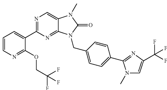
7-methyl-9-(4-(1-methyl-4-(trifluoromethyl)-1H-imidazol-2-yl)benzyl)-2-(2-(2,2,2-trifluoromethoxy)pyridin-3-yl)-7,8-dihydro-8H-purin-8-one
