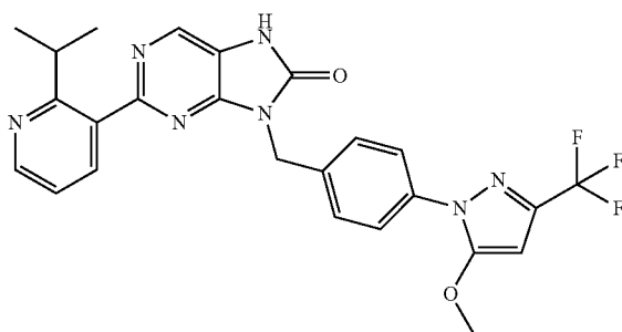
2-(2-isopropylpyridin-3-yl)-9-(4-(5-methoxy-3-(trifluoromethyl)-1H-pyrazol-1-yl)benzyl)-7,9-dihydro-8H-purin-8-one
