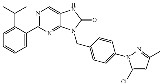
9-(4-(5-chloro-3-methyl-1H-pyrazol-1-yl)benzyl)-2-(2-isopropylphenyl)-7,9-dihydro-8H-purin-8-one
