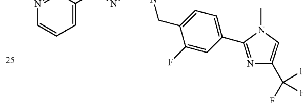
9-(2-fluoro-4-(1-methyl-4-(trifluoromethyl)-1H-imidazol-2-yl)benzyl)-2-(2-isopropylpyridin-3-yl)-7,9-dihydro-8H-purin-8-one
