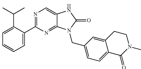
5-((2-(2-isopropylphenyl)-8-oxo-7,8-dihydro-8H-purin-8-yl)methyl)-2-methyl-3,4-dihydroquinolin-1(2H)-one
