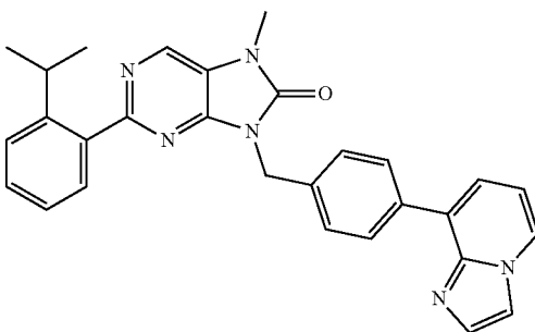
8-(4-(1H-imidazol-1,2-a)pyridin-8-yl)benzyl)-2-(2-isopropylphenyl)-7-methyl-7,8-dihydro-8H-purin-8-one
