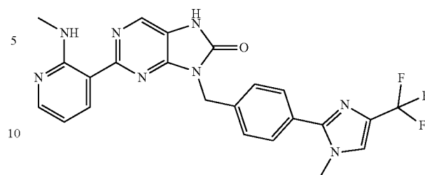
8-(4-(1-methyl-4-(trifluoromethyl)-1H-imidazol-2-yl)benzyl)-2-(2-methylamino)pyridin-3-yl)-7,9-dihydro-8H-purin-8-one
