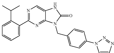
9-(4-(1H-1,2,3-triazol-1-yl)benzyl)-2-(2-isopropylphenyl)-7,9-dihydro-8H-purin-8-one
