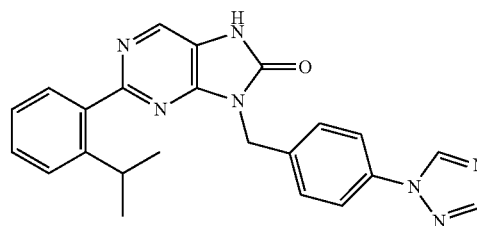
8-(4-(1H-1,2,4-triazol-1-yl)benzyl)-2-(2-isopropylphenyl)-7,9-dihydro-8H-purin-8-one
