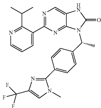
(R)-2-(2-isopropylpyridin-3-yl)-9-(1-(4-(1-methyl-4-(trifluoromethyl)-1H-imidazol-2-yl)phenyl)ethyl)-7,9-dihydro-8H-purin-8-one
