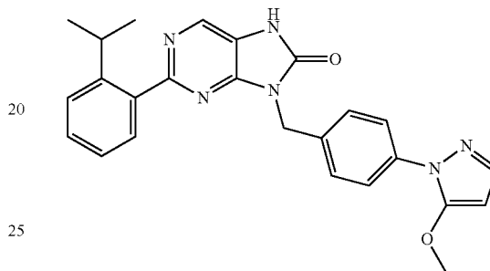
2-(2-isopropylphenyl)-9-(4-(5-methoxy-1H-pyrazol-1-yl)benzyl)-7,9-dihydro-8H-purin-8-one
