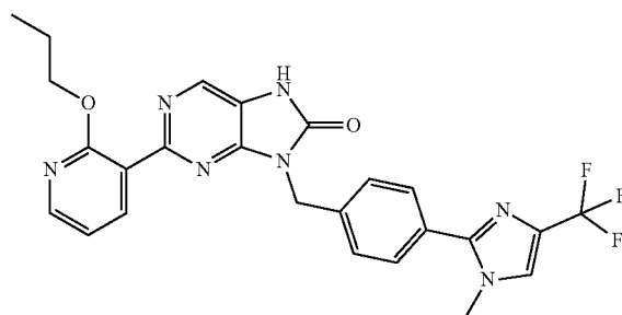
9-(4-(1-methyl-4-(trifluoromethyl)-1H-imidazol-2-yl)benzyl)-2-(2-propoxypyridin-3-yl)-7,8-dihydro-8H-purin-8-one
