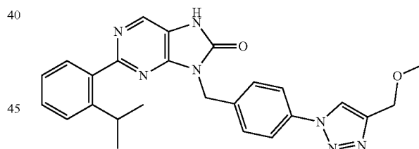
2-(2-isopropylphenyl)-8-(4-(4-(methoxymethyl)-1H-1,2,3-triazol-1-yl)benzyl)-7,8-dihydro-8H-purin-8-one
