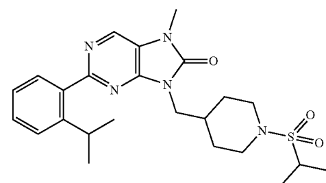
2-(2-isopropylphenyl)-8-((1-(isopropylsulfonyl)piperidin-4-yl)methyl)-7-methyl-7,9-dihydro-8H-purin-8-one
