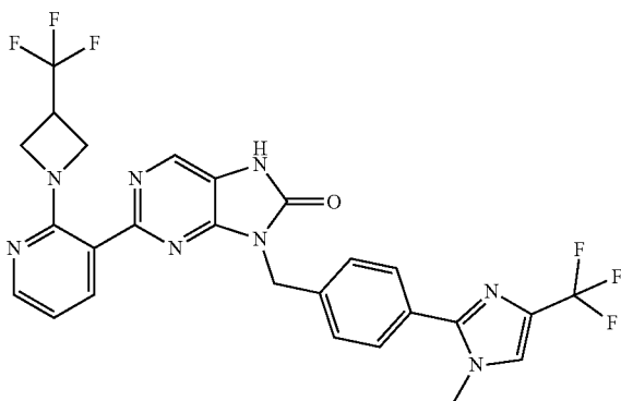
9-(4-(1-methyl-4-(trifluoromethyl)-1H-imidazol-2-yl)benzyl)-2-(2-(3-(trifluoromethyl)azetidin-1-yl)pyridin-3-yl)-7,9-dihydro-8H-purin-8-one
