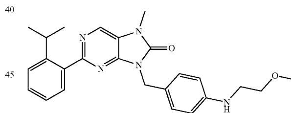
2-(2-isopropylphenyl)-8-(4-((2-methoxyethyl)amino)benzyl)-7-methyl-7,9-dihydro-8H-purin-8-one
