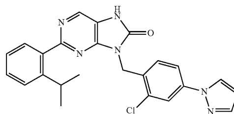
9-(2-chloro-4-(1H-pyrazol-1-yl)benzyl)-2-(2-isopropylphenyl)-7,8-dihydro-8H-purin-8-one
