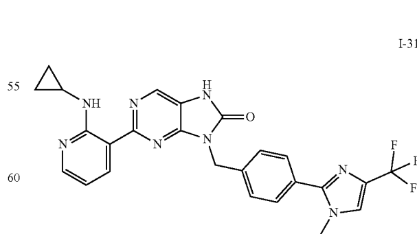
2-(2-cyclopropylamino)pyridin-3-yl)-8-(4-(1-methyl-4-(trifluoromethyl)-1H-imidazol-2-yl)benzyl)-7,9-dihydro-8H-purin-8-one
