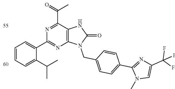
6-acetyl-2-(2-isopropylphenyl)-8-(4-(1-methyl-4-(trifluoromethyl)-1H-imidazol-2-yl)benzyl)-7,9-dihydro-8H-purin-8-one
