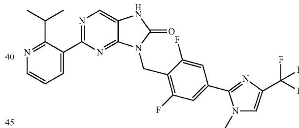
9-(2,8-difluoro-4-(1-methyl-4-(trifluoromethyl)-1H-imidazol-2-yl)benzyl)-2-(2-isopropylpyridin-3-yl)-7,9-dihydro-8H-purin-8-one
