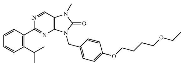
9-(4-(2-ethoxyethoxy)benzyl)-2-(2-isopropylphenethyl)-7-methyl-7,9-dihydro-8H-purin-8-one
