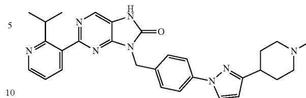
2-(2-isopropylpyridin-3-yl)-9-(4-(3-(1-methylpiperidin-4-yl)-1H-pyrazol-1-yl)benzyl)-7,8-dihydro-8H-purin-8-one
