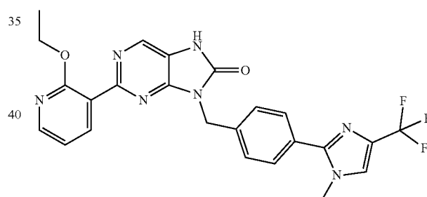
2-(2-(2-ethoxy)pyridin-3-yl)-9-(4-(1-methyl-4-(trifluoromethyl)-1H-imidazol-2-yl)benzyl)-7,9-dihydro-8H-purin-8-one
