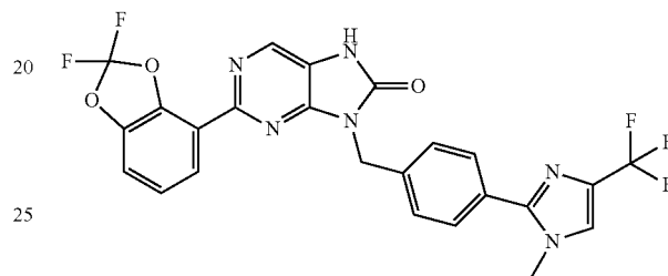
2-(2,2-difluorobenzo[d(1,3)dioxol-4-yl)-8-(4-yl-methyl-4-trifluoromethyl)-1H-imidazol-2-yl)benzyl)-7,2-dihydro-8H-purin-8-one
