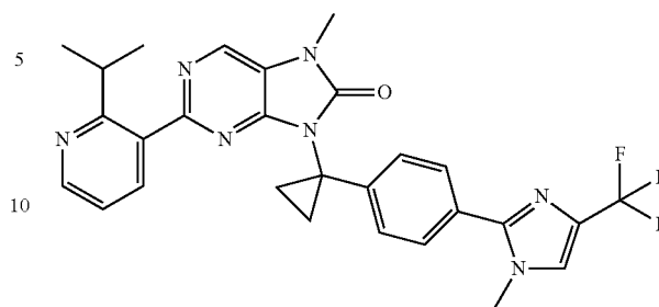
2-(2-isopropylpyridin-3-yl)-7-methyl-6-(1-(4-(t-methyl-4-(trifluoromethyl)-1H-imidazol-2-yl)phenyl)-cyclopropyl)-7,8-dihydro-8H-purin-8-one
