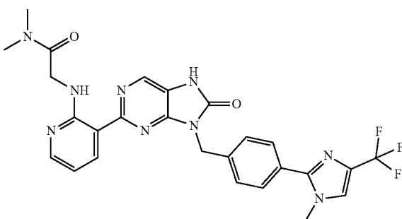
N,N-dimethyl-2-((3-(9-(4-(1-methyl-4-(trifluoromethyl)-1H-imidazol-2-yl)benzyl)-8-oxo-8,9-dihydro-7H-purin-2-yl)pyridin-2-yl)amino)acetamide
