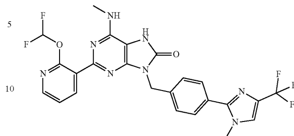
2-(2-(difluoromethoxy)pyridin-3-yl)-8-(4-(1-methyl-4-(trifluoromethyl)-1H-imidazol-2-yl)benzyl)-8-(methylamino)-7,9-dihydro-8H-purin-8-one
