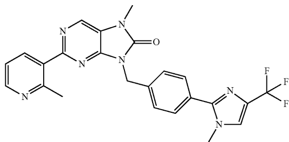
7-methyl-8-(4-(1-methyl-4-(trifluoromethyl)-1H-imidazol-2-yl)benzyl)-2-(2-methylpyridin-3-yl)-7,8-dihydro-8H-purin-8-one
