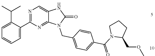
(S)-2-(2-isopropylphenyl)-8-(4-(2-methylpyrrolidine-1-carbonyl)benzyl)-7,9-dihydro-8H-purin-8-one
