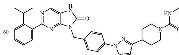
4-(1-(4-((2-(2-isopropylphenyl)-8-oxo-7,8-dihydro-8H-purin-9- yl)methyl)phenyl)-1H-pyrazol-3-yl)-N-methylpiperidine-1- carboxamide
