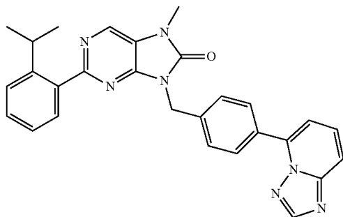
9-(4-([1,2,4]triazolo[1,5-a]pyridin-5-yl)benzyl)-2-(2-isopropylphenyl)-7-methyl-7,8-dihydro-8H-purin-8-one
