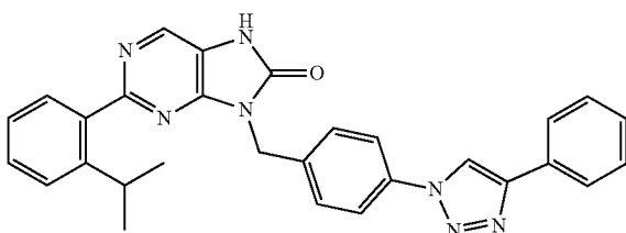
2-(2-isopropylphenyl)-9-(4-(4-phenyl-1H-1,2,3-triazol-1-yl)benzyl)-7,9-dihydro-8H-purin-8-one
