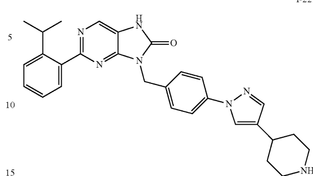
2-(2-isopropylphenyl)-9-(4-(4-(piperidine-4-yl)-1H-pyrazol-1-yl)benzyl)-7,9-dihydro-8H-purin-8-one
