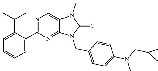
8-(4-((cyclopropylmethyl)(methyl)amino)benzyl)-2-(2-isopropylphenyl)-7-methyl-7,9-dihydro-8H-purin-8-one
