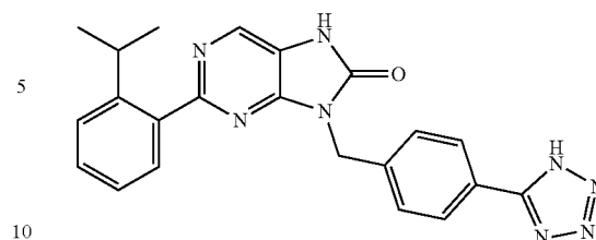
9-(4-(1H-tetrazol-5-yl)benzyl)-2-(2-isopropylphenyl)-7,9-dihydro-8H-purin-8-one
