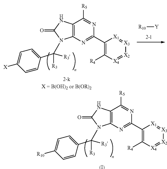
General Scheme 4
