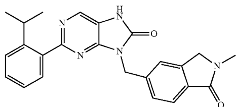
2-(2-isopropylphenyl)-8-((2-methyl-1-oxoisoxindolin-5-yl)methyl)-7,9-dihydro-8H-purin-8-one
