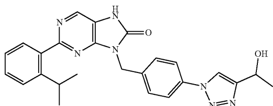
(R)-8-(4-(4-(1-hydroxyethyl)-1H-1,2,3-triazol-1-yl)benzyl)-2-(2-isopropylphenyl)-7,9-dihydro-8H-purin-8-one
