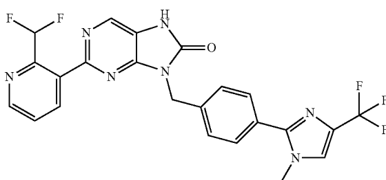
2-(2-difluoromethylpyridin-3-yl)-9-(4-(1-methyl-4-(trifluoromethyl)-1H-imidazol-2-yl)benzyl)-7,9-dihydro-8H-purin-8-one
