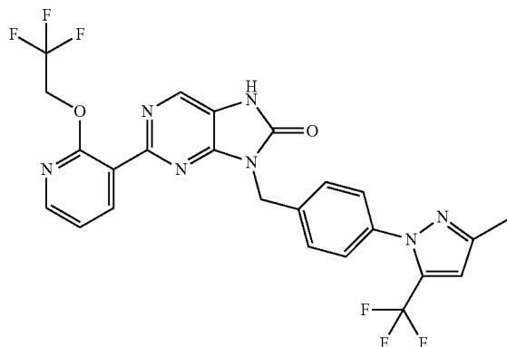
3-(4-(3-methyl-5-(trifluoromethyl)-1H-pyrazol-1-yl)benzyl)-2-(2-(2,2,2-trifluoroethoxy)pyridin-3-yl)-7,8-dihydro-8H-purin-8-one
