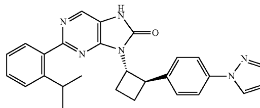
9-((1S,2R)-2-(4-(1H-pyrazol-1-yl)phenyl)cyclobutyl)-2-(2-isopropylphenyl)-7,9-dihydro-8H-purin-8-one
