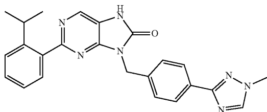
2-(2-isopropylphenyl)-9-(4-(1-methyl-1H-1,2,4-triazol-3-yl)benzyl)-7,8-dihydro-8H-purin-8-one
