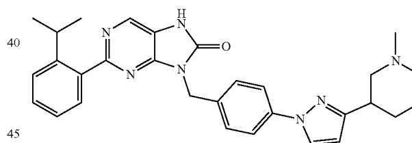
2-(2-isopropylphenyl)-9-(4-(3-(1-methylpiperidin-3-yl)-1H-pyrazol-1-yl)benzyl)-7,9-dihydro-8H-purin-8-one
