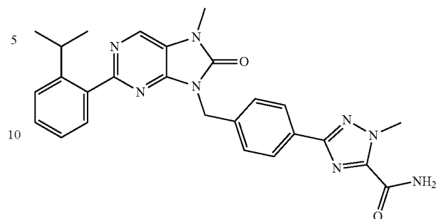
3-(4-((2-(2-isopropylphenyl)-7-methyl-8-oxo-7,8-dihydro-8H-purin-8-yl)methyl)phenyl)-1-methyl-1H-1,2,4-triazole-5-carboxamide
