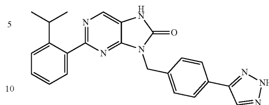
9-(4-(2H-1,2,3-triazol-4-yl)benzyl)-2-(2-isopropylphenyl)-7,9-dihydro-8H-purin-8-one
