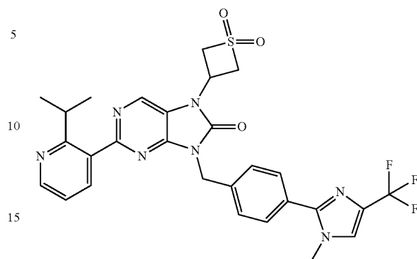
7-(1,1-dioxidothietan-3-yl)-2-(2-isopropylpyridin-3-yl)-8-(4-(1-methyl-4-(trifluoromethyl)-1H-imidazol-2-yl)benzyl)-7,9-dihydro-8H-purin-8-one
