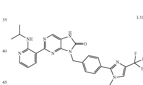
2-(2-isopropylamino)pyridin-3-yl)-8-(4-(1-methyl-4-(trifluoromethyl)-1H-imidazol-2-yl)benzyl)-7,9-dihydro-8H-purin-8-one
