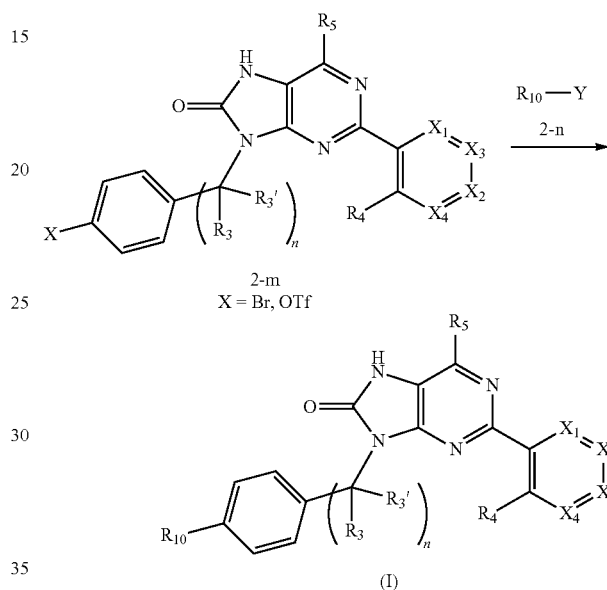
General Scheme 5
