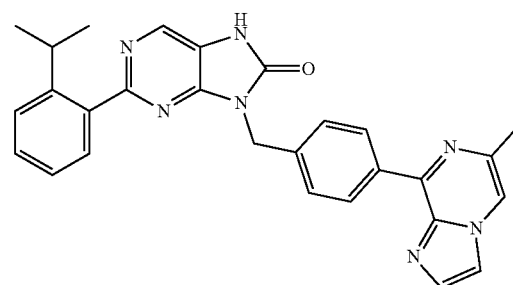
2-(2-isopropylphenyl)-8-(4-(6-methylimidazol[1,2-a]pyrazin-8-yl)benzyl)-7,9-dihydro-8H-purin-8-one
