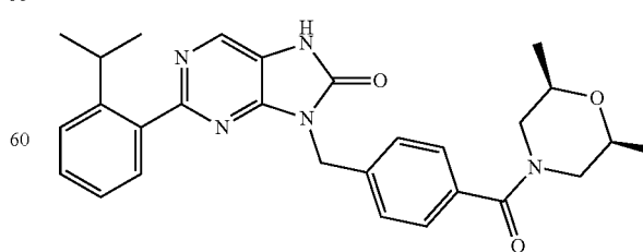
9-(4-((2R,6S), 2,5-dimethylmorpholine-4-carbonylbenzyl)-2-(2-isopropylphenyl)-7,8-dihydro-8H-purin-8-one
