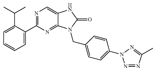
2-(2-isopropylphenyl)-8-(4-(5-methyl-2H-tetrazol-2-yl)benzyl)-7,9-dihydro-8H-purin-8-one
