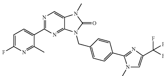
2-(6-fluoro-2-methylpyridin-3-yl)-7-methyl-9-(4-(1-methyl-4-(trifluoromethyl)-1H-imidazol-2-yl)benzyl)-7,8-dihydro-8H-purin-8-one
