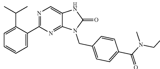
N-ethyl-4-((2-(2-isopropylphenyl)-8-oxo-7,8-dihydro 9H-purin-8-yl)methyl)-N-methylbenzamide
