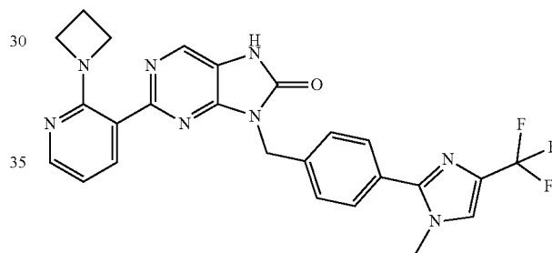
2-(2-(azetidin-1-yl)pyridin-3-yl)-9-(4-(1-methyl-4-(trifluoromethyl)-1H-imidazol-2-yl)benzyl)-7,9-dihydro-8H-purin-8-one
