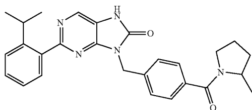
2-(2-isopropylphenyl)-8-(4-(2-methylpyrrolidine-1-carbonyl)benzyl)-7,8-dihydro-8H-purin-8-one
