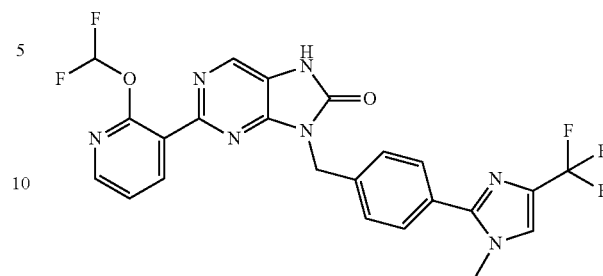
2-(2-(difluoromethoxy)pyridin-3-yl)-9-(4-(1-methyl-4-trifluoromethyl)-1H-imidazol-2-yl)benzyl)-7,9-dihydro-8H-purin-8-one
