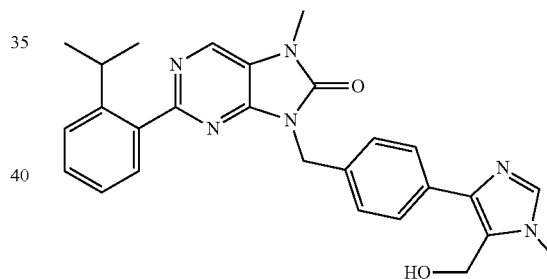
9-(4-(5-(hydroxymethyl)-1-methyl-1H-imidazol-4-yl)benzyl)-2-(2-isopropylphenyl)-7-methyl-7,9-dihydro-8H-purin-8-one
