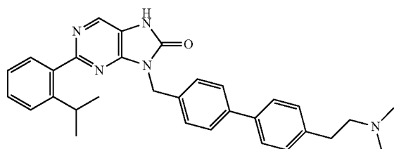
9-((4'-(2-(dimethylamino)ethyl)-(1,1'-biphenyl)-4-yl)methyl)-2-(2-isopropylphenyl)-7,9-dihydro-8H-purin-8-one
