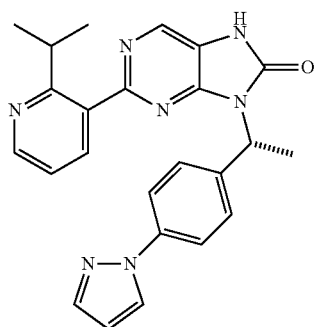
(R)-3-(1-(4-(1H-pyrazol-1-yl)phenyl)ethyl)-2-(2-isopropylpyridin-3-yl)-7,8-dihydro-8H-purin-8-one
