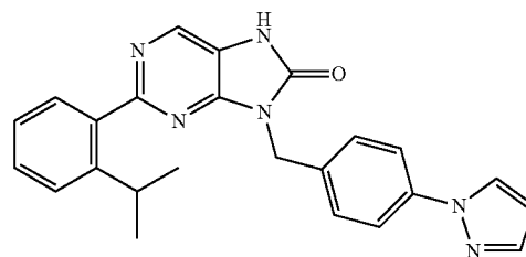
9-(4-(1H-pyrazol-1-yl)benzyl)-2-(2-isopropylphenyl)-7,9-dihydro-8H-purin-8-one
