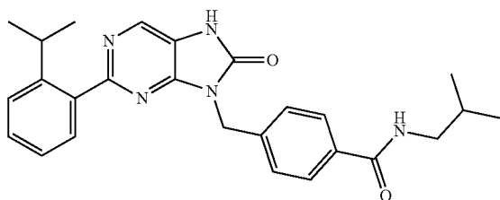
N-isopropyl-4-((2-(2-isopropylphenyl)-8-oxo-7,8-dihydro-8H-purin-8-yl)methyl)benzamide
