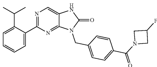
8-(4-(3-fluoroazetidine-1-carbonyl)benzyl)-2-(2-isopropylphenyl)-7,8-dihydro-8H-purin-8-one
