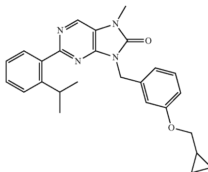
9-(3-(cyclobutoxy)benzyl)-2-(2-isopropylphenyl)-7,9-dihydro-8H-purin-8-one
