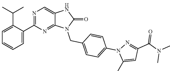
1-(4-((2-(2-isopropylphenyl)-8-oxo-7,8-dihydro-8H-purin-8-yl)methyl)phenyl)-N,N,5-trimethyl-1H-pyrazole-3-carboxamide
