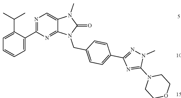
2-(2-isopropylphenyl)-7-methyl-3-(4-(5-methyl-5-morpholine-1H-1,2,4-triazol-3-yl)benzyl)-7,8-dihydro-8H-purin-8-one
