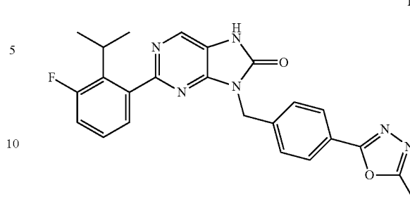
2-(3-fluoro-2-isopropylphenyl)-8-(4-(5-methyl-1,3,4-oxadiazol-2-yl)benzyl)-7,9-dihydro-8H-purin-8-one
