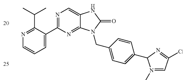
9-(4-(2-chloro-5-methyl-1H-pyrazol-1-yl)benzyl)-2-(2-isopropylpyridin-3-yl)-7,9-dihydro-8H-purin-8-one
