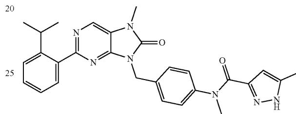
N-(4-((2-(2-isopropylphenyl)-7-methyl-8-oxo-7,8-dihydro-8H-purin-9-yl)methyl)phenyl)-N-5-dimethyl-1H-pyrazole-3-carboxamide
