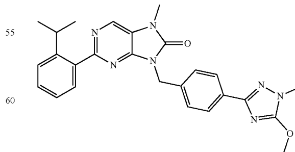
2-(2-isopropylphenyl)-9-(4-(5-methoxy-1-methyl-1H-1,2,4-triazol-3-yl)benzyl)-7-methyl-7,8-dihydro-8H-purin-8-one
