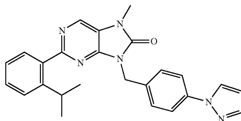
9-(4-(1H-pyrazol-1-yl)benzyl)-2-(2-isopropylphenyl)-7-methyl-7,8-dihydro-8H-purin-8-one
