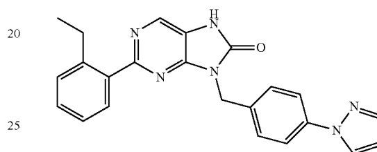
9-(4-(1H-pyrazol-1-yl)(benzyl)-2-(2-ethylphenyl)-7,9-dihydro-8H-purin-8-one
