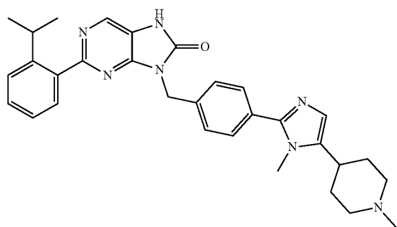
2-(2-isopropylphenyl)-9-(4-(1-methyl-5-(1-methylpiperidin-4-yl)-1H-imidazol-2-yl)benzyl)-7,9-dihydro-8H-purin-8-one
