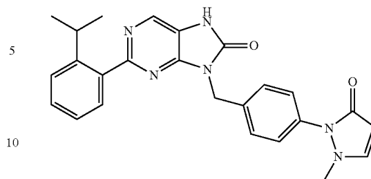
2-(2-isopropylphenyl)-6-(4-(2-methyl-5-oxo-2,5-dihydro-1H-pyrazol-1-yl)benzyl)-7,9-dihydro-8H-purin-8-one
