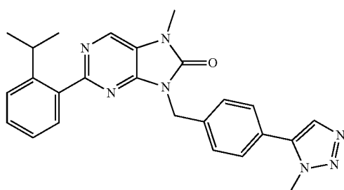
2-(2-isopropylphenyl)-7-methyl-8-(4-(1-methyl-1H-1,2,3-triazol-5-yl)benzyl)-7,9-dihydro-8H-purin-8-one
