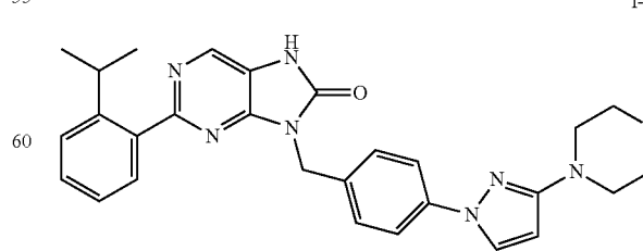
2-(2-isopropylphenyl)-8-(4-(3-morpholine-1H-pyrazol-1-yl)benzyl)-7,9-dihydro-8H-purin-8-one
