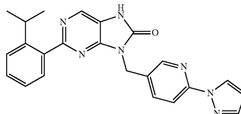
9-((8-(1H-pyrazol-1-yl)pyridin-3-yl)methyl)-2-(2-isopropylphenyl)-7,9-dihydro-8H-purin-8-one
