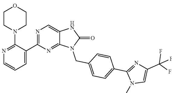
9-(4-(1-methyl-4-(trifluoromethyl)-1H-imidazol-2-yl)benzyl)-2-(2-morpholinopyridin-3-yl)-7,9-dihydro-8H-purin-8-one
