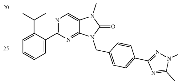
8-(4-(1,5-dimethyl-1H-1,2,4-triazol-3-yl)benzyl)-2-(2-isopropylphenyl)-7-methyl-7,8-dihydro-8H-purin-8-one
