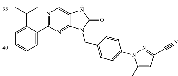
1-(4-((2-(2-isopropylphenyl)-8-oxo-7,8-dihydro-8H-purin-8-yl)methyl)phenyl)-5-methyl-1H-pyrazol-8-carbonitrile
