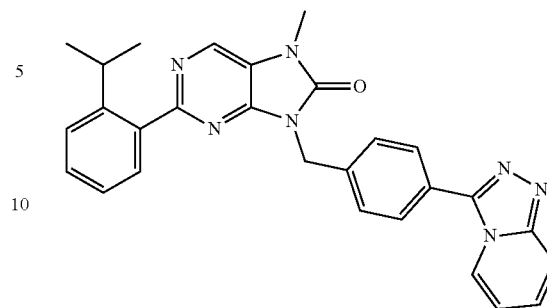
9-(4-([1,2,4]triazolo[4,3-a]pyridin-3-yl)benzyl)-2-(2-isopropylphenyl)-7-methyl-7,8-dihydro-8H-purin-8-one
