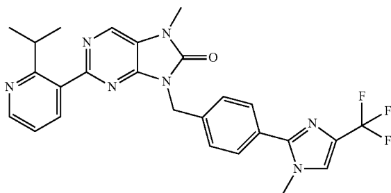
2-(2-isopropylpyridin-3-yl)-7-methyl-9-(4-(1-methyl-4-trifluoromethyl-1H-imidazol-2-yl)-benzyl)-7,9-dihydro-8H-purin-8-one
