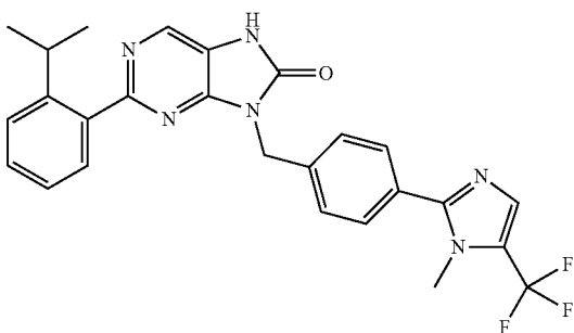
2-(2-isopropylphenyl)-9-(4-(1-methyl)-5-(trifluoromethyl)-1H-imidazol-2-yl)benzyl-7,9-dihydro-8H-purin-8-one
