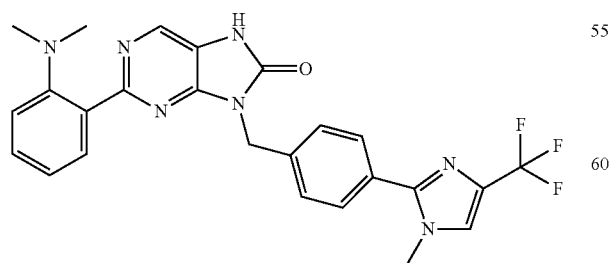
2-(2-(dimethylaminophenyl)-8-(4-(t-methyl-4-(trifluoromethyl)-1H-imidazol-2-yl)benzyl)-7,9-dihydro-8H-purin-8-one
