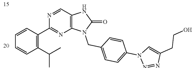
9-(4-(4-(2-hydroxyethyl)-1H-1,2,3-triazol-1-yl)benzyl)-2-(2-isopropylphenyl)-7,9-dihydro-8H-purin-8-one
