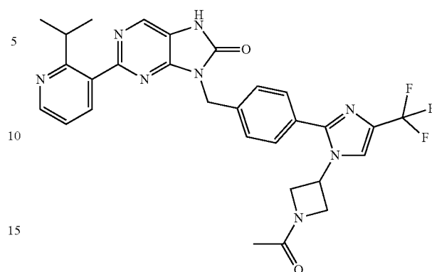
9-(4-(1-(1-acetylazetidin-3-yl)-4-(trifluoromethyl)-1H-imidazol- 2-yl)benzyl)-2-(2-isopropylpyridin-3-yl)-7,9-dihydro-8H-purin-8-one
