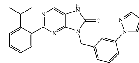
9-(3-(1H-pyrazol-1-yl)benzyl)-2-(2-isopropylphenyl)-7,9-dihydro-8H-purin-8-one
