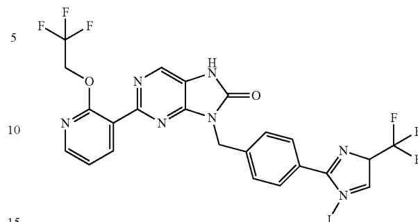
9-(4-(1-methyl-4-(trifluoromethyl)-1H-imidazol-2-yl)benzyl)-2-(2,2,2-trifluoroethoxy)pyridin-3-yl)-7,9-dihydro-8H-purin-8-one
