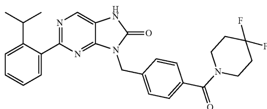
9-(4-(4,4-difluoropiperidine-1-carbonyl)benzyl)-2-(2-isopropylphenyl)-7,8-dihydro-8H-purin-8-one
