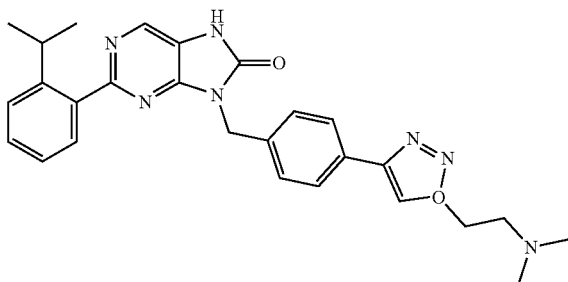
9-(4-(1-(2-(dimethylamino)ethyl)-1H-1,2,3-triazol-4-yl)benzyl)-2-(2-isopropylphenyl)-7,9-dihydro-8H-purin-8-one
