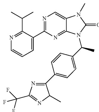
(S)-2-(2-isopropylpyridin-3-yl)-7-methyl-9-(1-(4-(1-methyl-4-(trifluoromethyl)-1H-imidazol-2-yl)phenyl)ethyl)-7,9-dihydro-8H-purin-8-one
