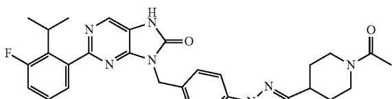
8-(4-(3-(1-acetylpiperidin-4-yl)-1H-pyrazol-1-yl)benzyl)-2-(3-fluoro-2-isopropylphenyl)-7,8-dihydro-8H-purin-8-one
