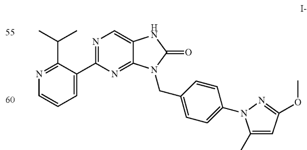
2-(2-isopropylpyridin-3-yl)-9-(4-(3-methoxy-5-methyl-1H-pyrazol-1-yl)benzyl)-7,9-dihydro-8H-purin-8-one
