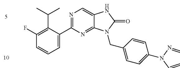
9-(4-(1H-pyrazol-1-yl)benzyl)-2-(3-fluoro-2-isopropylphenyl)-7,9-dihydro-8H-purin-8-one
