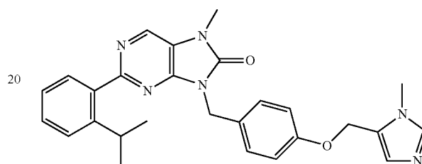
2-(2-isopropylphenyl)-7-methyl-9-(4-((1-methyl-1H-imidazol-5-yl) methoxy)benzyl)-7,9-dihydro-8H-purin-8-one
