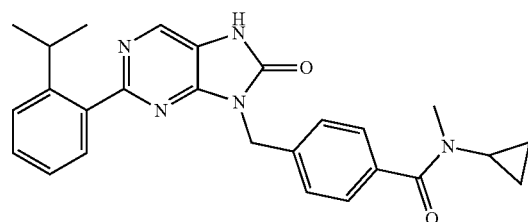
N-cyclopropyl-4-((2-(2-isopropylphenyl)-8-oxo-7,8-dihydro-8H-purin-8-yl)methyl)-N-methylbenzamide
