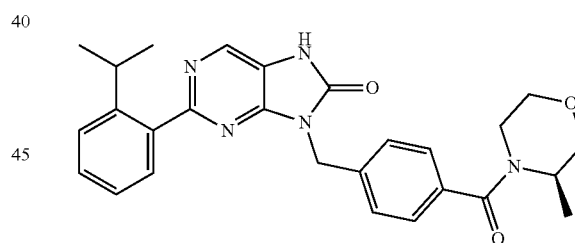
(R)-2-(2-isopropylphenyl)-8-(4-(3-methylmorpholine-4-carbonyl)benzyl)-7,8-dihydro-8H-purin-8-one
