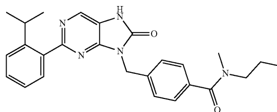
4-((2-(2-isopropylphenyl)-8-oxo-7,8-dihydro 9H-purin-8-yl)methyl)-N-methyl-N-propylbenzamide
