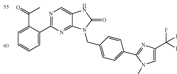
2-(2-acetylphenyl)-8-(4-(1-methyl-4-(trifluoromethyl)-1H-imidazol-2-yl)benzyl)-7,8-dihydro-8H-purin-8-one
