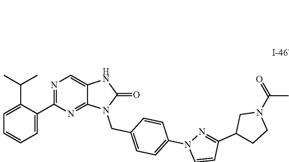
8-(4-(3-(1-acetylpyrrolidin-3-yl)-1H-pyrazol-1-yl)benzyl)-2-(2-isopropylphenyl)-7,8-dihydro-8H-purin-8-one
