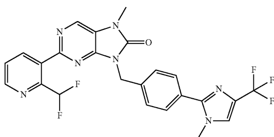
2-(2-(difluoromethyl)pyridin-3-yl)-7-methyl-9-(4-(1-methyl-4-(trifluoromethyl)-1H-imidazol-2-yl)-benzyl)-7,9-dihydro-8H-purin-8-one
