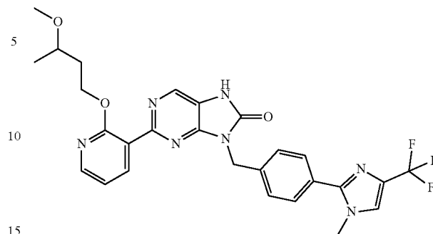
2-(2-(3-methoxybutoxy)pyridin-3-yl)-8-(4-(1-methyl-4-(trifluoromethyl)-1H-imidazol-2-yl)benzyl)-7,9-dihydro-8H-purin-8-one
