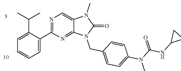
3-isopropyl-1-(4-((2-(2-isopropylphenyl)-7-methyl-8-oxo-7,5-dihydro-8H-purin-9-yl)methoxyethyl)-1-methyl
