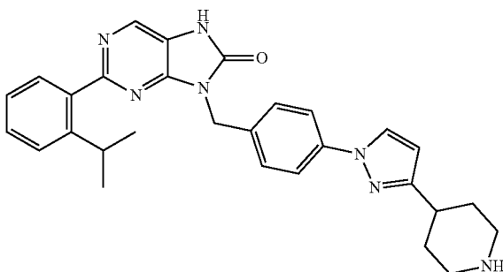
2-(2-isopropylphenyl)-9-(4-(3-(piperidin-4-yl)-1H-pyrazol-1-yl)benzyl)-7,9-dihydro-8H-purin-8-one
