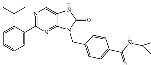
N-cyclopropyl-4-((2-(2-isopropylphenyl)-8-oxo-7,8-dihydro-9H-purin-8-yl)methyl)benzamide
