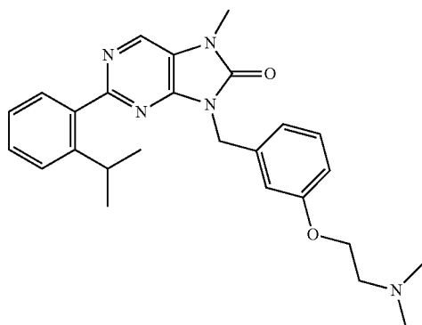
9-(3-(2-dimethylamino)ethoxy)benzyl-2-(2-isopropylphenyl)-7-methyl-7,9-dihydro-8H-purin-8-one
