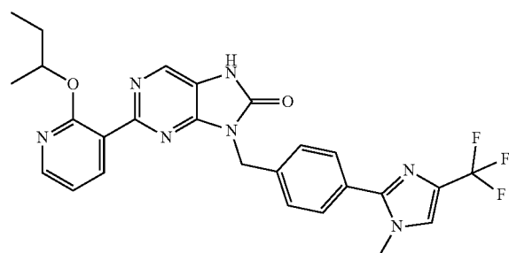
2-(2-(2-azobutoxy)pyridin-3-yl)-9-(4-(1-methyl-4-(trifluoromethyl)-1H-imidazol-2-yl)benzyl)-7,9-dihydro-8H-purin-8-one
