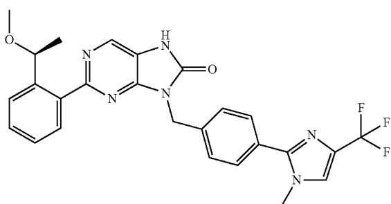
(S)-2-(2-(1-methoxyethyl)-8-(4-(1-methyl-4-(trifluoromethyl)-1H-imidazol-2-yl)benzyl)-7,9-dihydro-8H-purin-8-one
