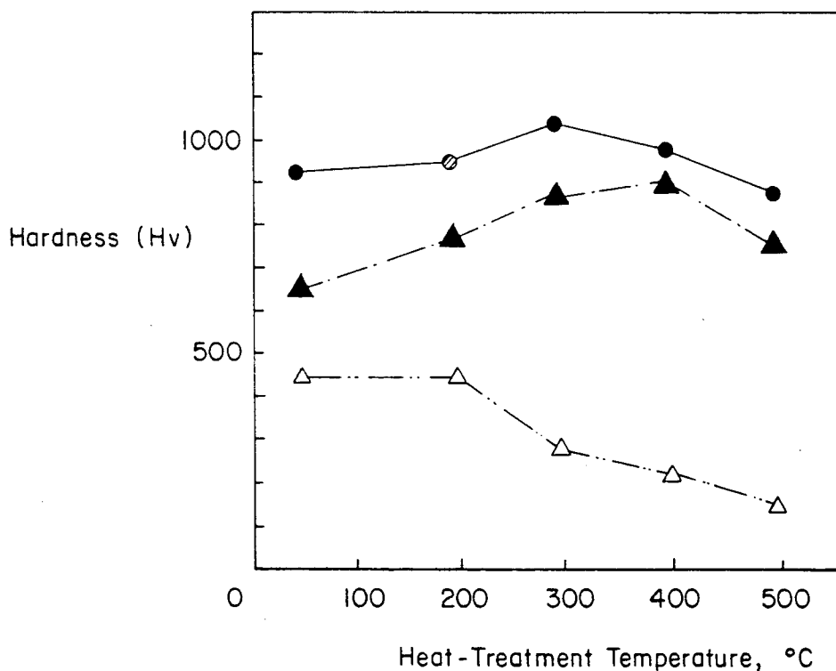
Hardness (Hv) with One Hour Heat-Treatment
