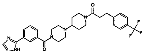
Compound 60
