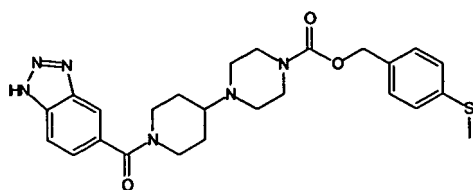
Compound 149
