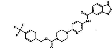
Compound 110
