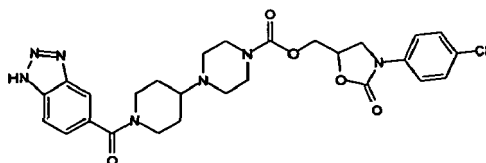
Compound 175
