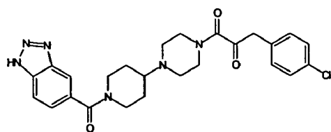
Compound 123
