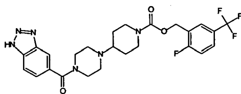
Compound 74
