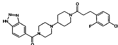
Compound 61
