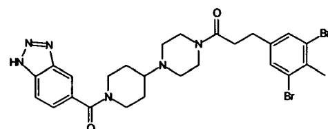
Compound 130
