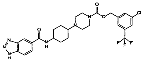
Compound 187
