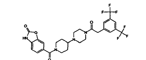
Compound 142
