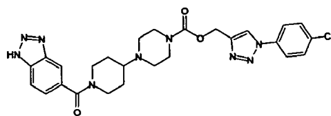
Compound 131
