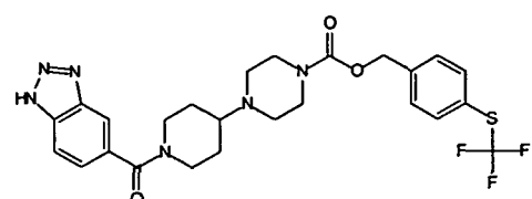
Compound 37
