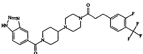
Compound 105
