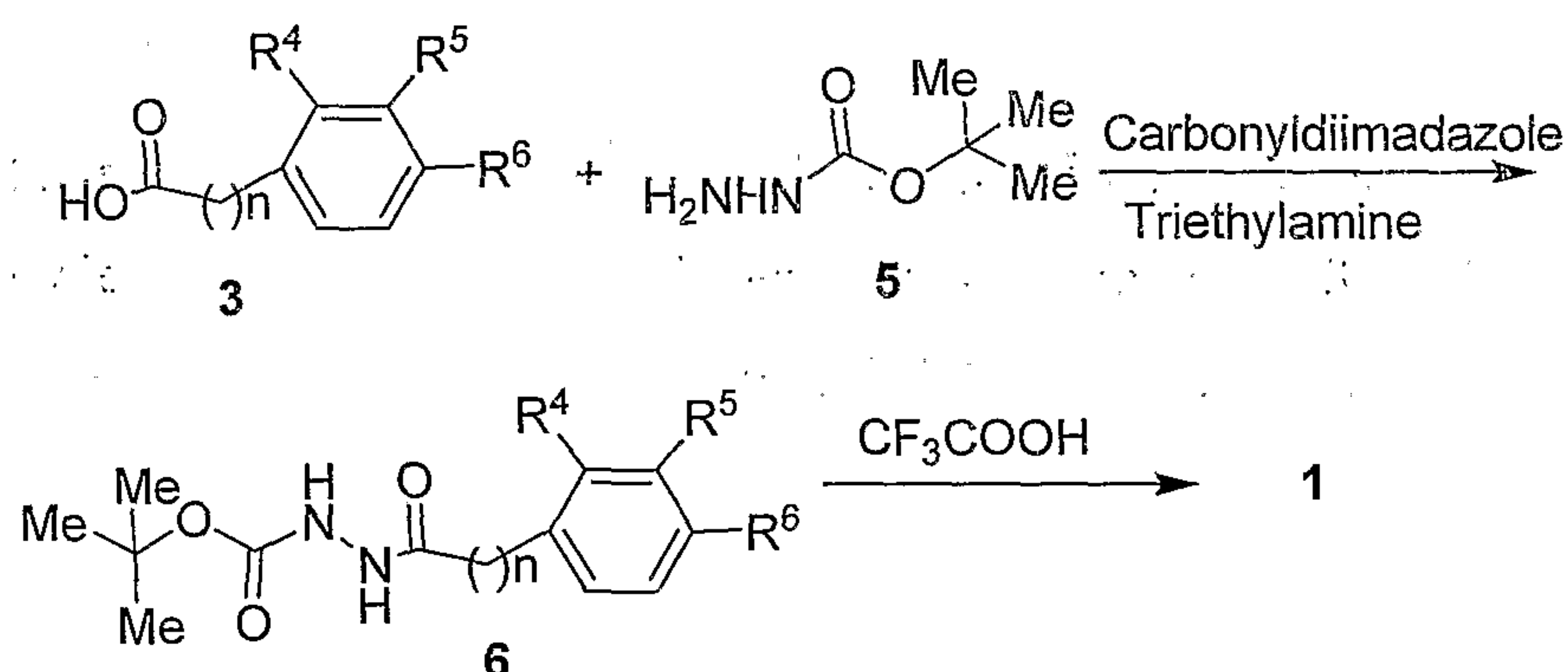
Scheme 5
