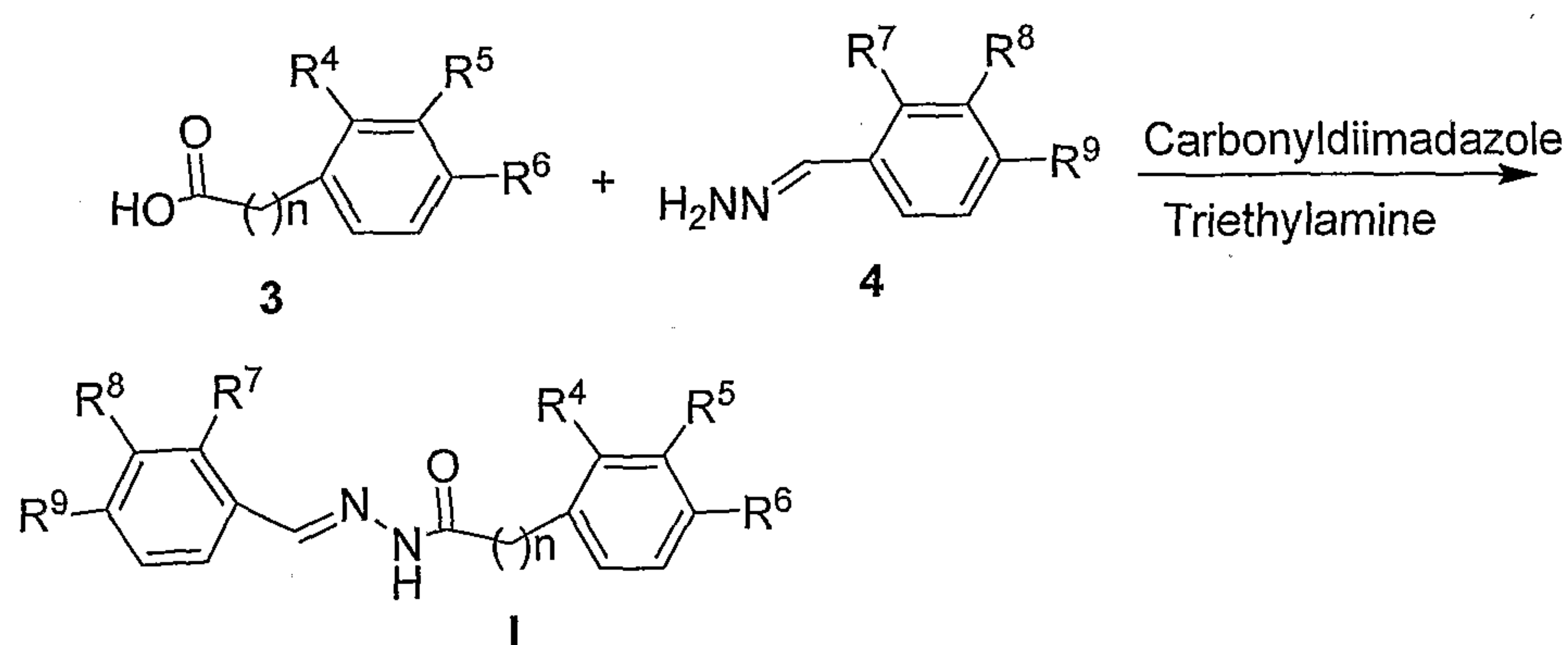
Scheme 4
