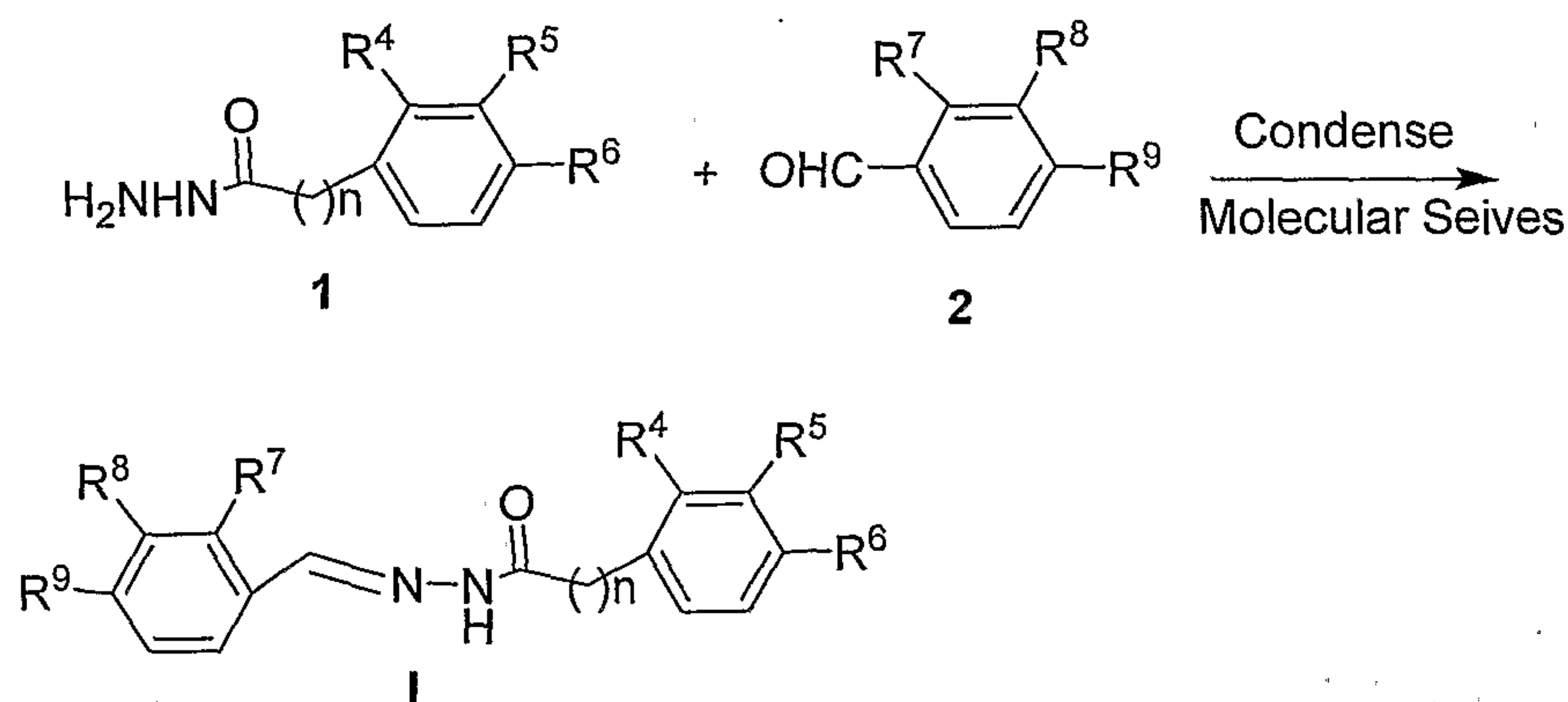
Scheme 3
