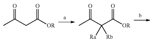
Scheme 42
