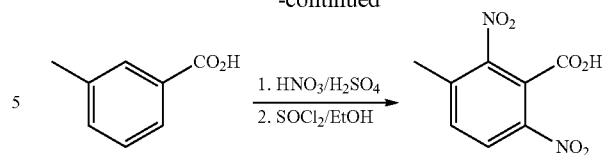
3-Methyl-2,6-dinitrobenzoic acid
