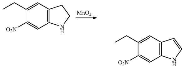
5-Ethyl-6-nitro-1H-indole
