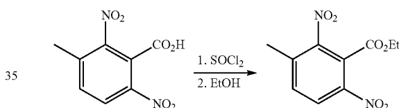
Ethyl 3-methyl-2,6-dinitrobenzoate
