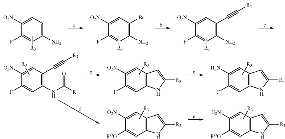
Scheme 18
