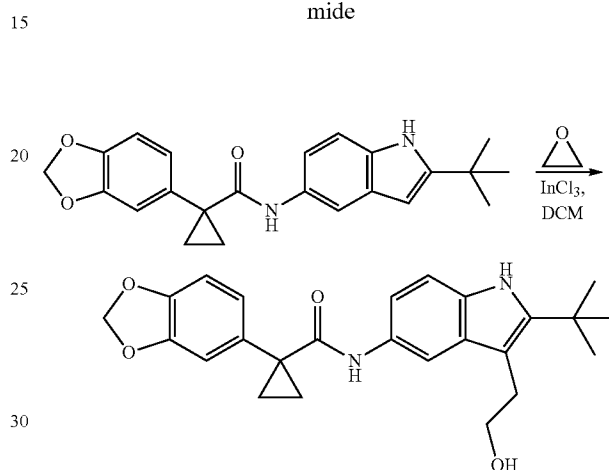
1-(Benzo[d][1,3]dioxol-5-yl)-N-(2-tert-butyl-3-(2-hydroxyethyl)-1H-indol-5-yl)cyclopropanecarboxamide
