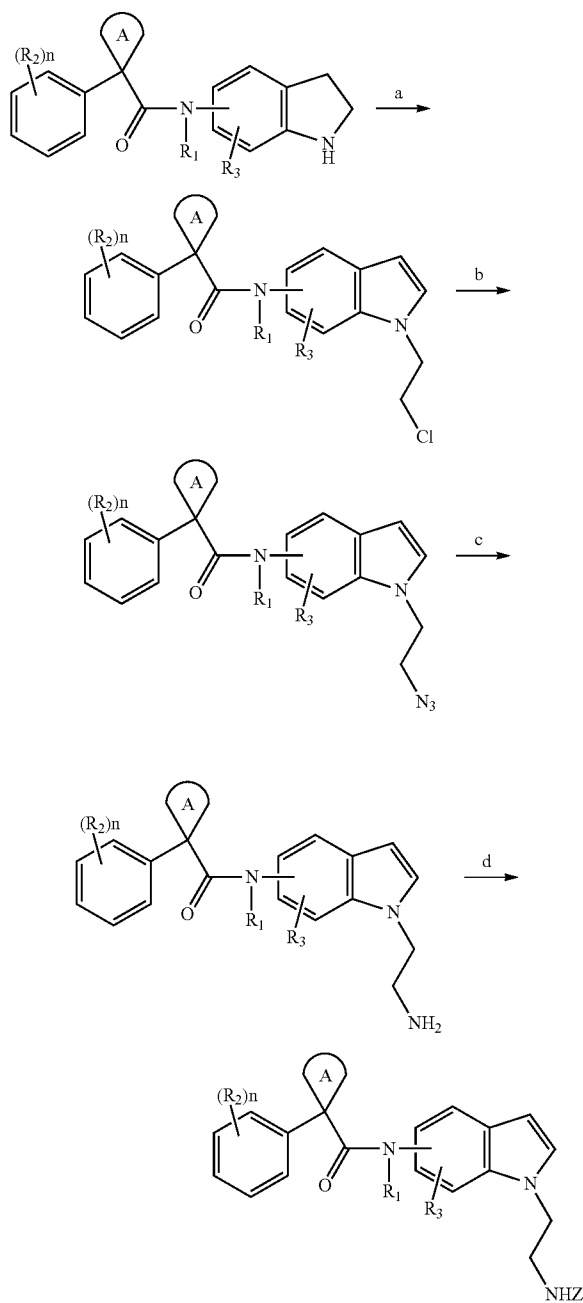
Scheme 41
