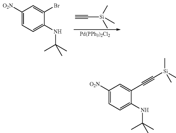
tert-Butyl-(4-nitro-2-trimethylsilanylethynyl-phenyl)-amine
