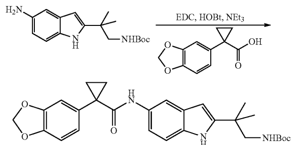
tert-Butyl 2-(5-(1-(benzo[d][1,3]dioxol-5-yl)cyclopropanecarboxamido)-1H-indol-2-yl)-2-methylpropylcarbamate
