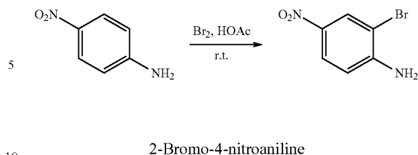
2-Bromo-4-nitroaniline
