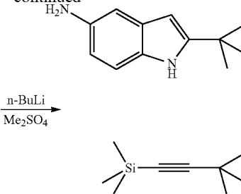
Trimethyl-(1-methyl-cyclopropylethynyl)-silane
