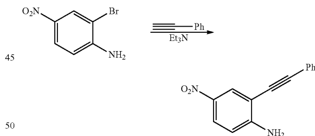
4-Nitro-2-(phenylethynyl)aniline
