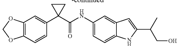
1-(Benzo[d][1,3]dioxol-5-yl)-N-(2-(1-hydroxypropan-2-yl)-1H-indol-5-yl)cyclopropanecarboxamide
