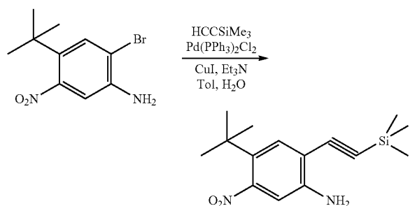
4-tert-Butyl-5-nitro-2-trimethylsilanylethynyl-phenylamine
