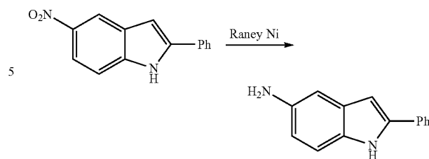
2-Phenyl-1H-indol-5-amine
