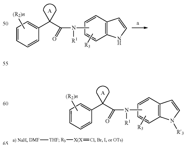
Scheme 36
