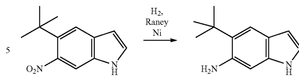
5-tert-Butyl-1H-indol-6-ylamine
