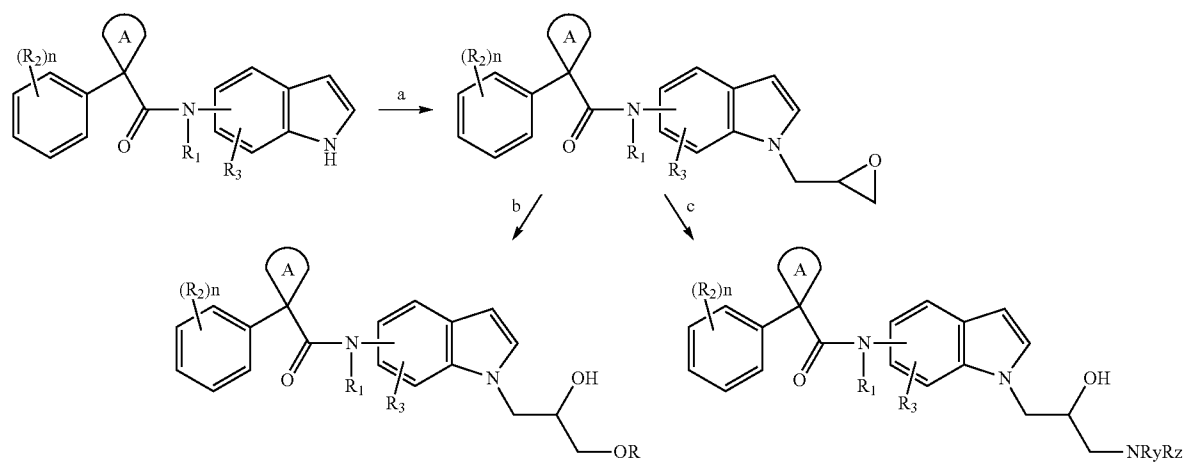
Scheme 39
