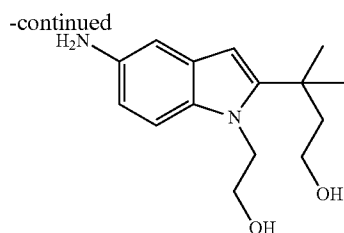
3-[5-Amino-1-(2-hydroxy-ethyl)-1H-indol-2-yl]-3-methyl-butan-1-ol
