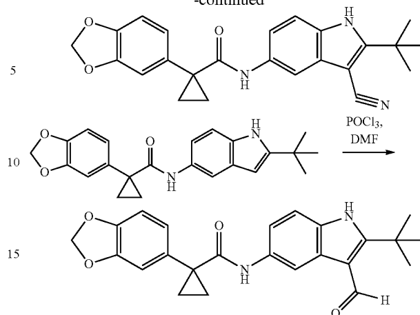
1-(Benzo[d][1,3]dioxol-5-yl)-N-(2-tert-butyl-3-formyl-1H-indol-5-yl)cyclopropane-carboxamide
