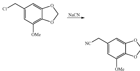
2-(7-Methoxybenzo[d][1,3]dioxol-5-yl)acetonitrile
