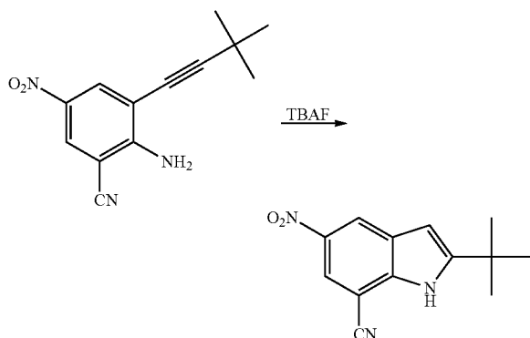
2-tert-Butyl-5-nitro-1H-indole-7-carbonitrile
