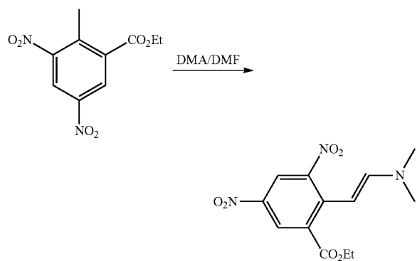
(E)-Ethyl 2-(2-(dimethylamino)vinyl)-3,5-dinitrobenzoate
