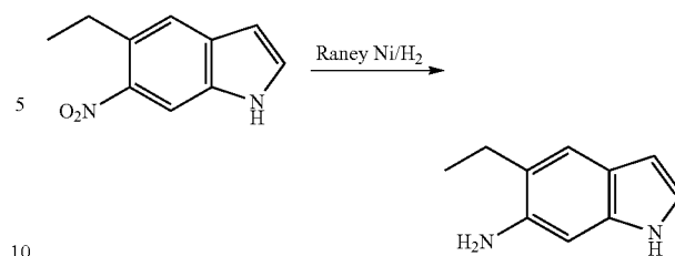
5-Ethyl-1H-indol-6-amine
