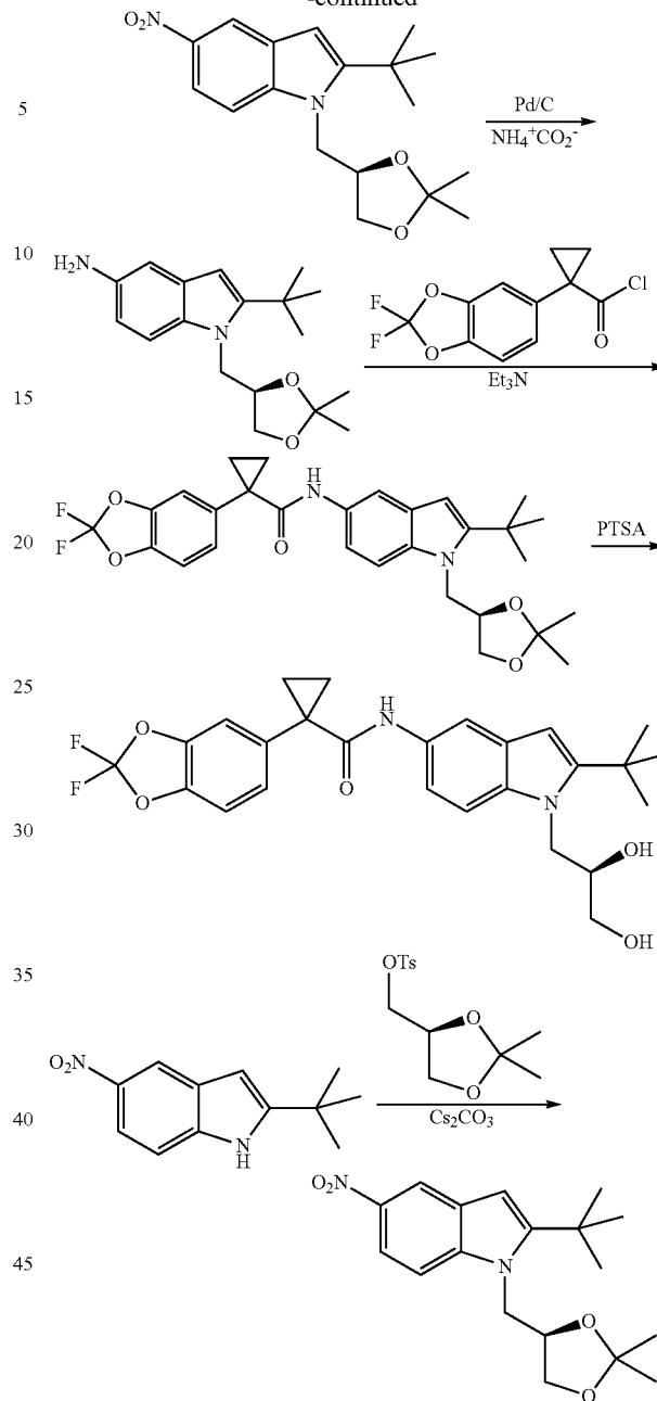
(R)-2-tert-Butyl-1-((2,2-dimethyl-1,3-dioxolan-4-yl)methyl)-5-nitro-1H-indole
