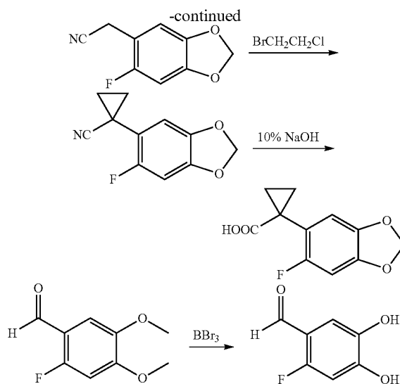
2-Fluoro-4,5-dihydroxy-benzaldehyde
