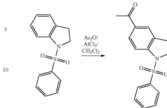
1-(1-(Phenylsulfonyl)indolin-5-yl)ethanone
