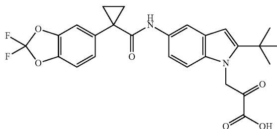
3-(2-tert-Butyl-5-(1-(2,2-difluorobenzo[d][1,3]dioxol-5-yl)cyclopropanecarboxamido)-1H-indol-1-yl)-2-oxopropanoic acid
