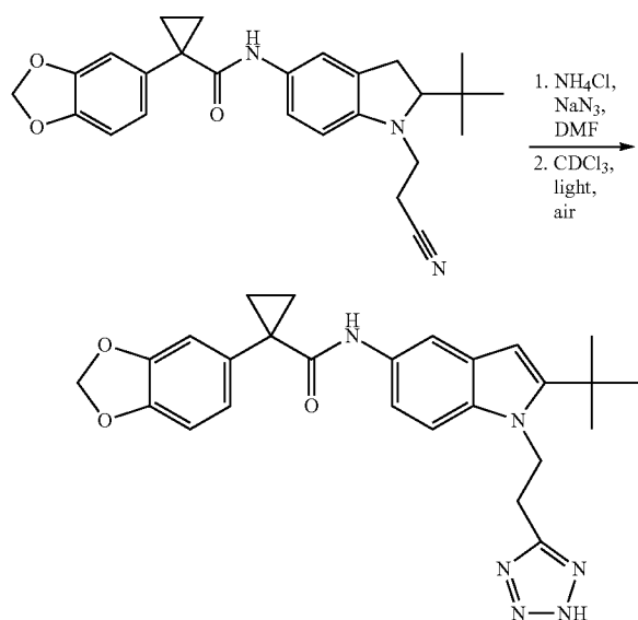
N-(1-(2-(2H-Tetrazol-5-yl)ethyl)-2-tert-butyl-1H-indol-5-yl)-1-(benzo[d][1,3]dioxol-5-yl)cyclopropanecarboxamide
