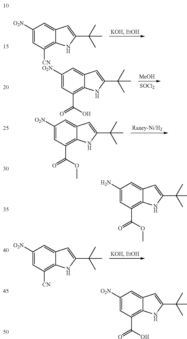
Methyl 5-amino-2-tert-butyl-1H-indole-7-carboxylate
