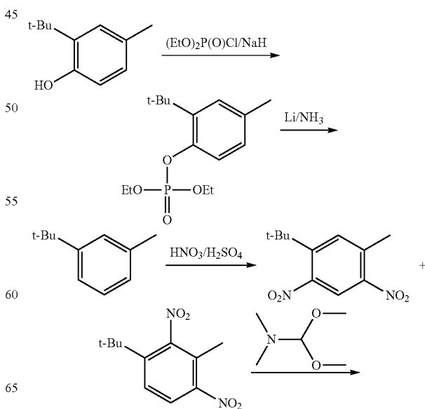
5-tert-Butyl-1H-indol-6-amine
