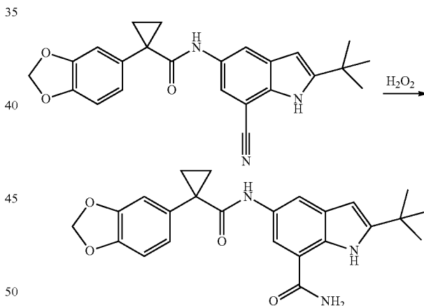
5-(1-(Benzo[d][1,3]dioxol-5-yl)cyclopropanecarboxamido)-2-tert-butyl-1H-indole-7-carboxamide
