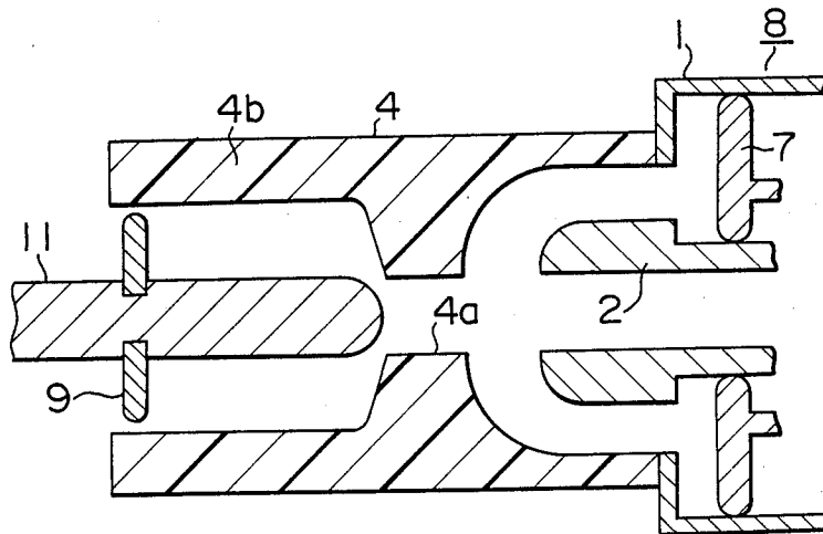
FIG. 10 PRIOR ART
