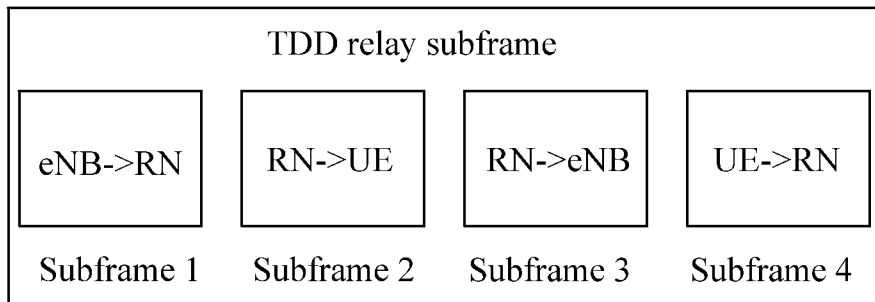
FIG. 1 (Prior Art)
