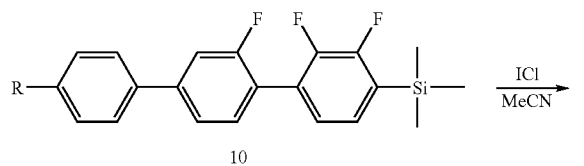
Scheme 3 Synthesis of the terphenyl (11) by iodo-desilylation
