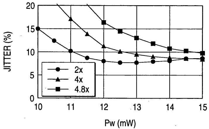
RECORDING POWER DEPENDENCY OF EDGE-TO-CLOCK JITTER
