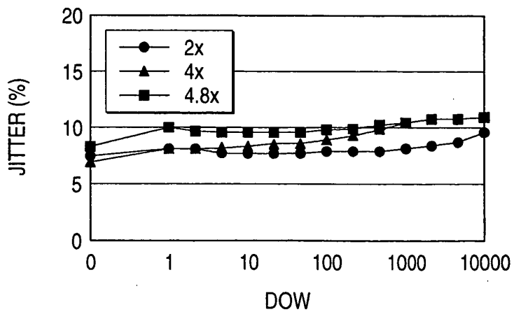
OVERWRITE CYCLE DEPENDENCY OF EDGE-TO-CLOCK JITTER
