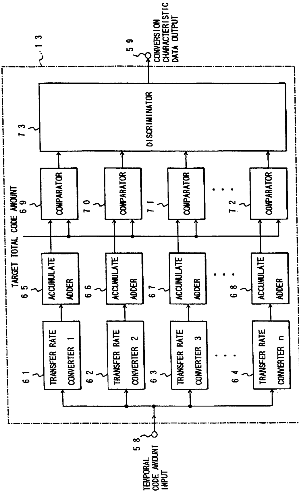
FIG. 2 PRIOR ART
