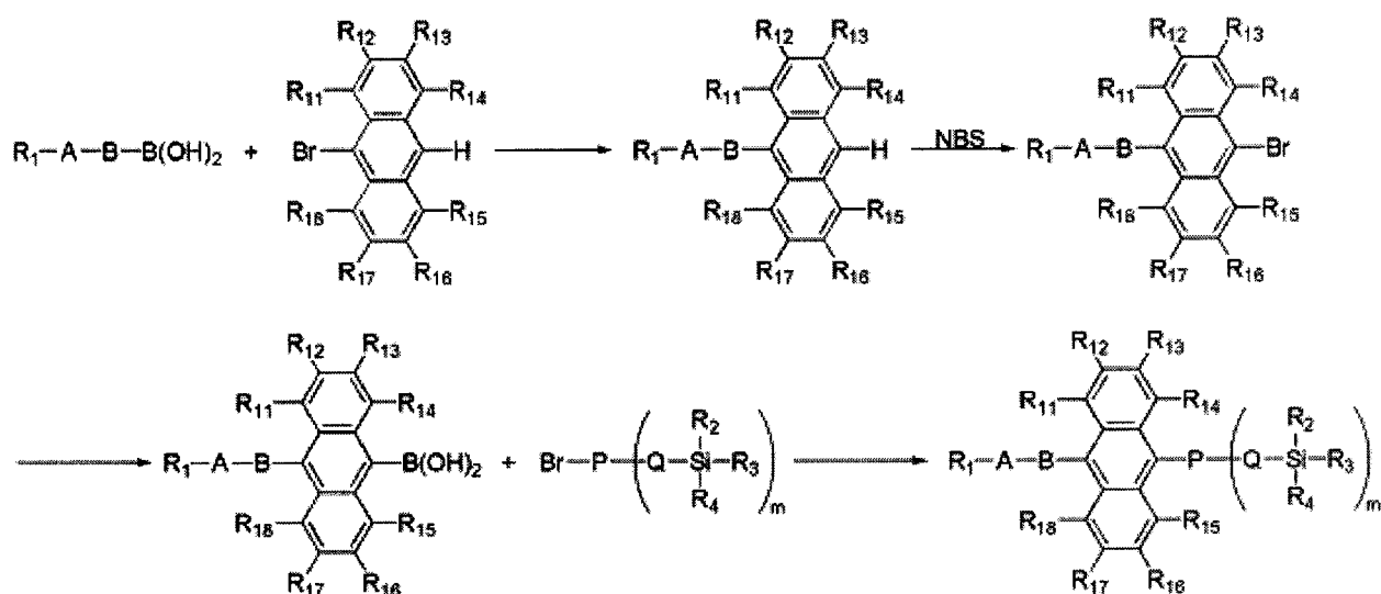
[Reaction Scheme 1]
