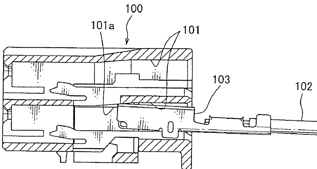
FIG. 9 PRIOR ART
