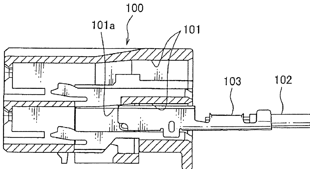
FIG. 8 PRIOR ART
