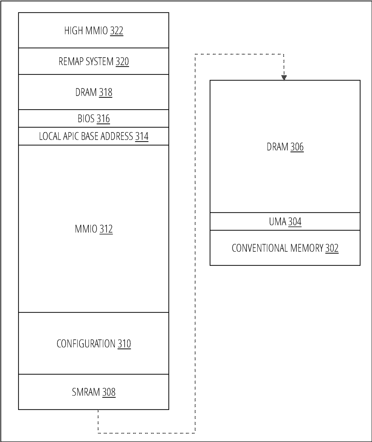
MEMORY MAP 210
