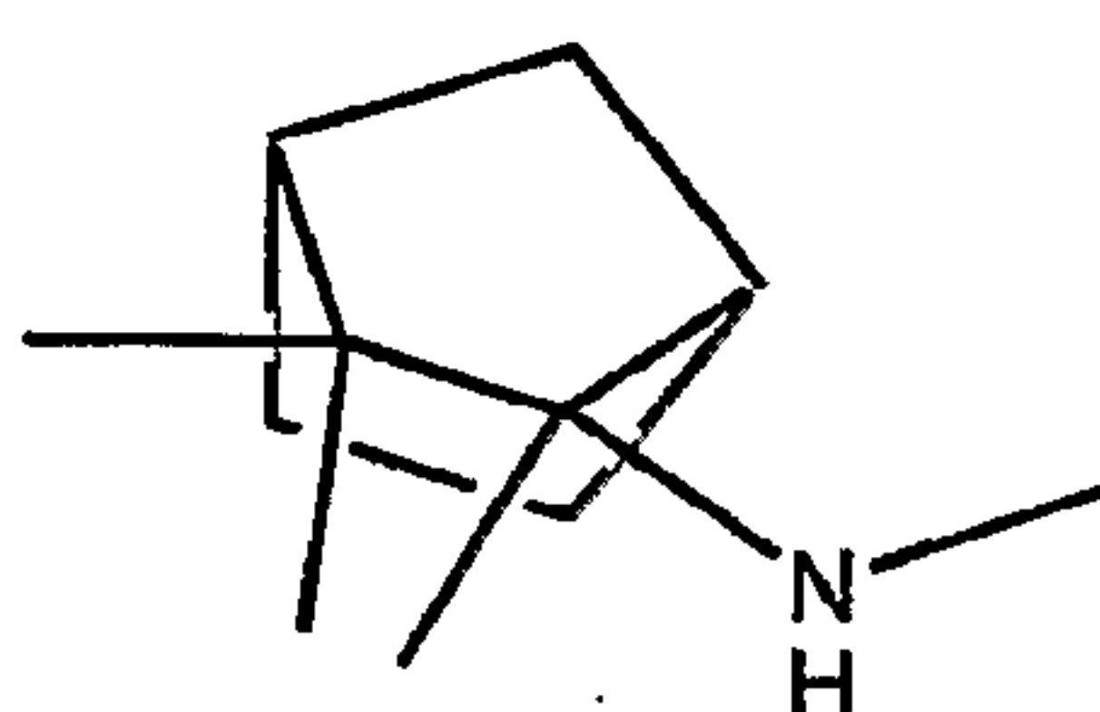
N-2,3,3-tetramethylbicyclo[2.2.1]heptan-2-amine
