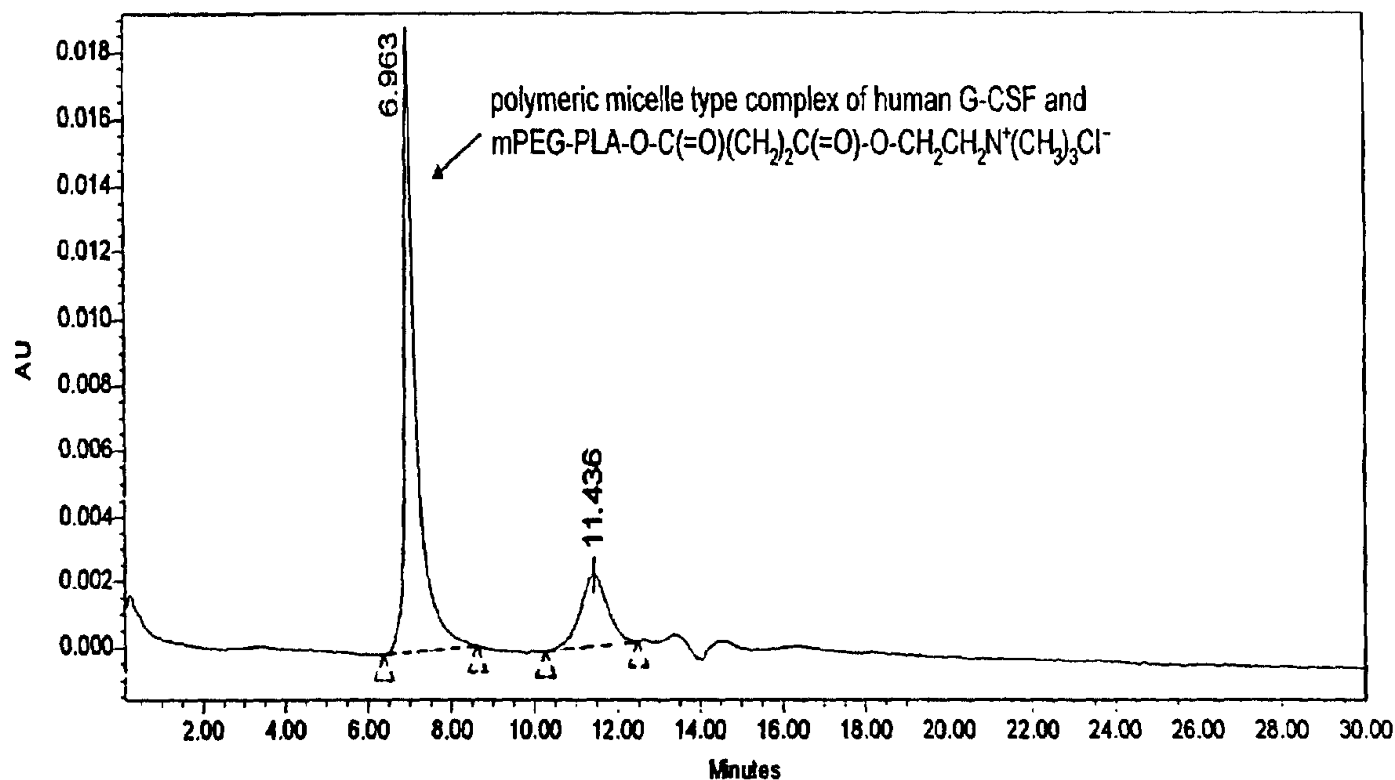
Auto-Scaled Chromatogram
