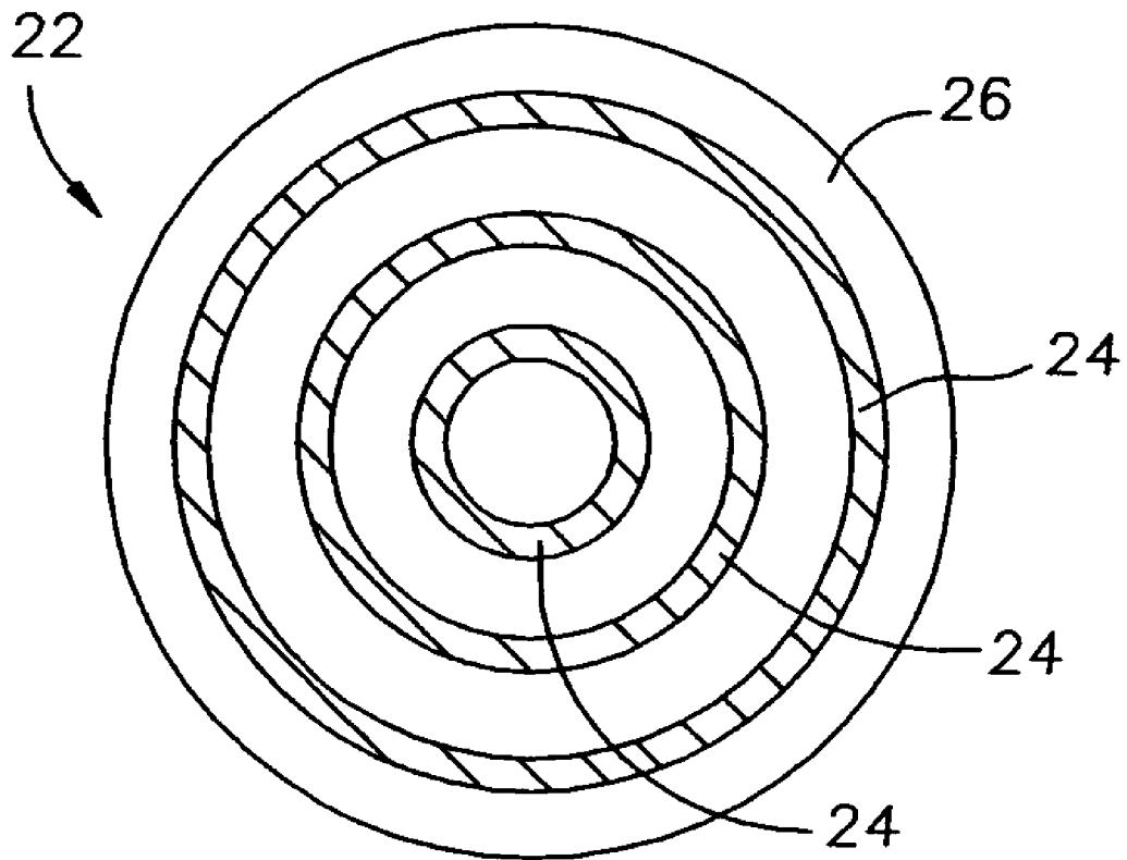
FIG. 4 (PRIOR ART)
