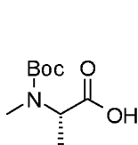
Boc-N-Methyl alanine
