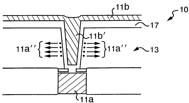
FIG. 1C (PRIOR ART)
