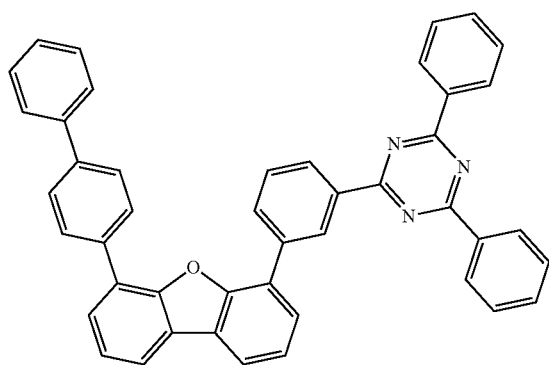
Compound C73
