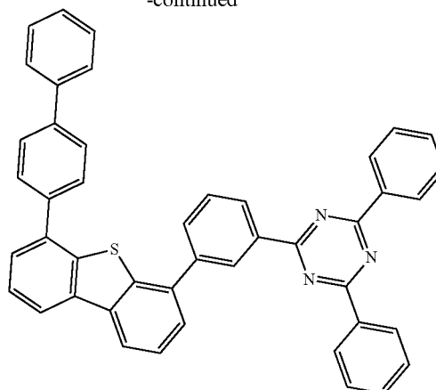
Compound C74
