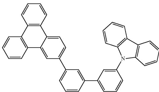
Compound E28
