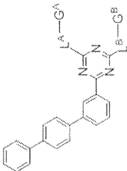
Formula III
