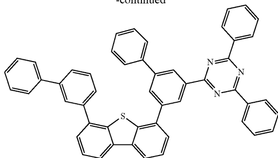
Compound A17
