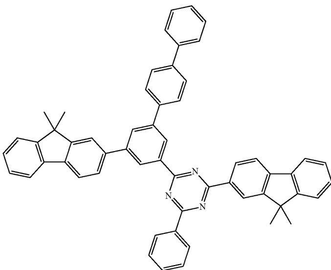
Compound B6
