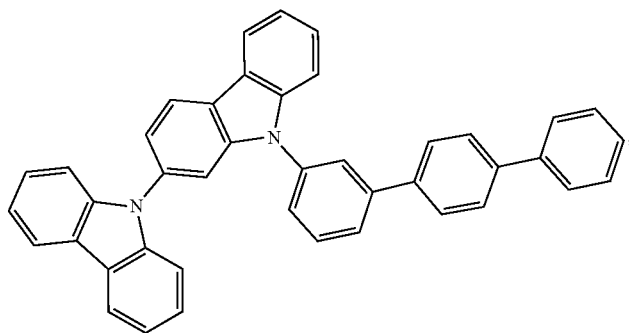
Compound G7
