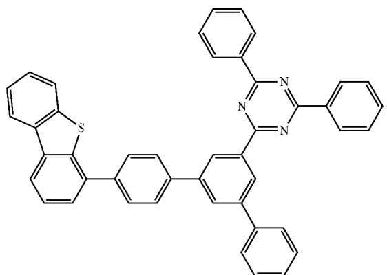
Compound A113
