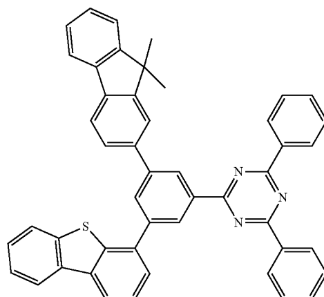
Compound A116
