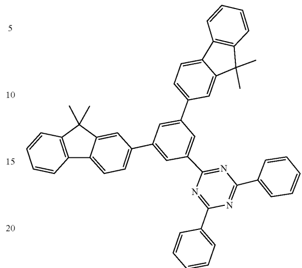
Compound B7
