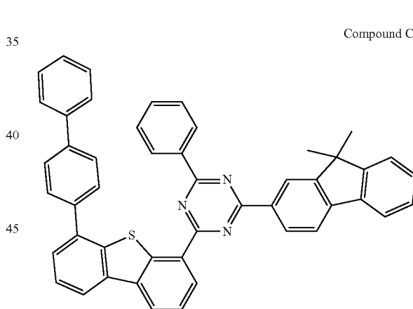
Compound C173
