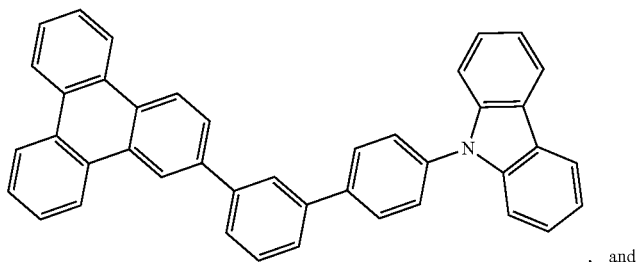
Compound E29
