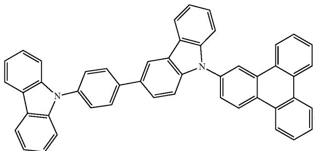
Compound G12
