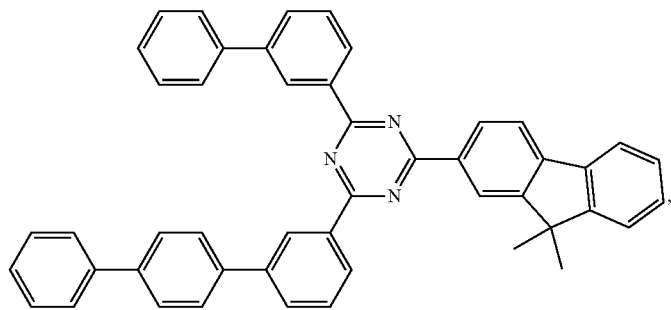
Compound F5
