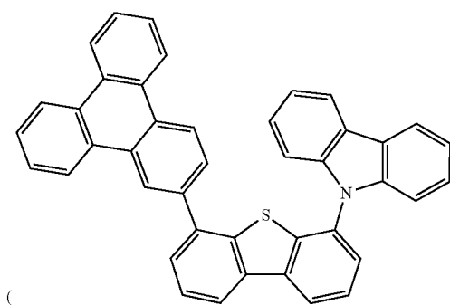
Compound E26
