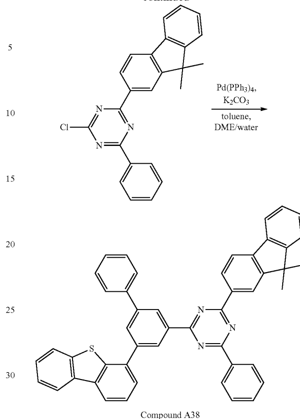
Compound A38
