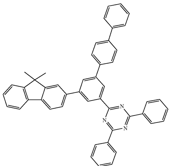
Compound B3
