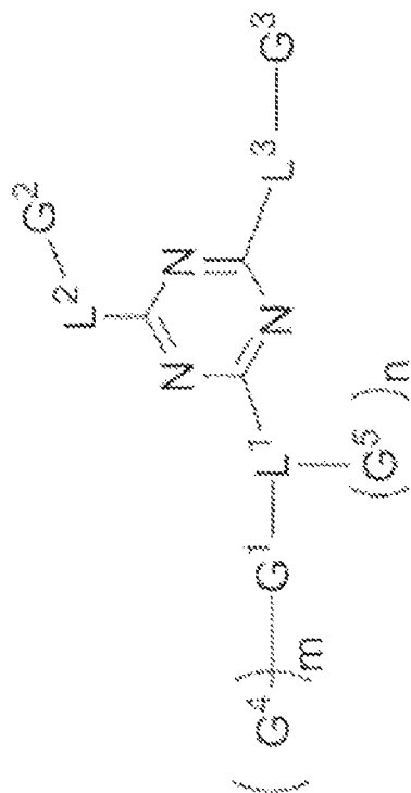
Formula I
