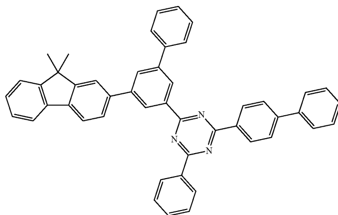
Compound B4
