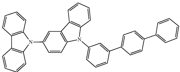
Compound G6
