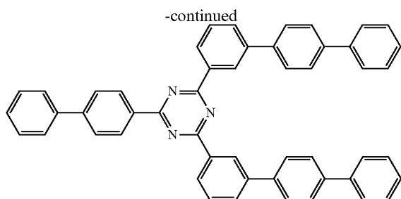
Compound F3
