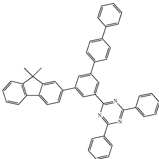
Compound B3
