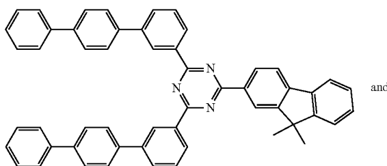
Compound F13
