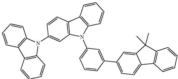
Compound G24
