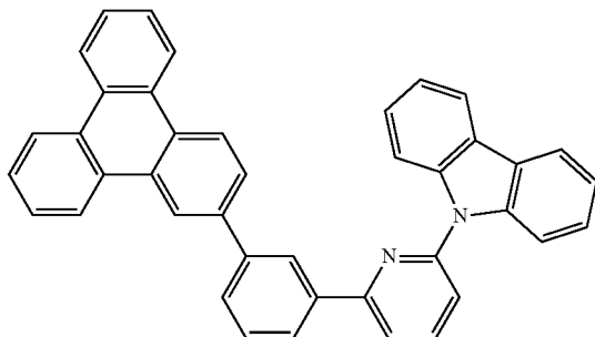
Compound E30
