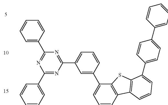
Compound C74
