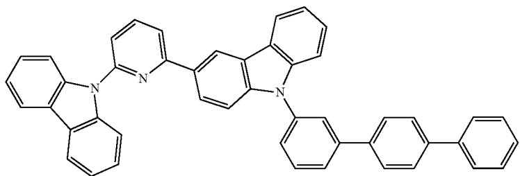
Compound G3
