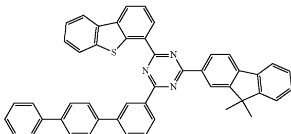
Compound F13
