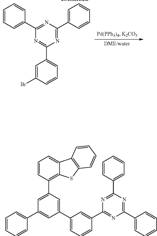
Compound A110
