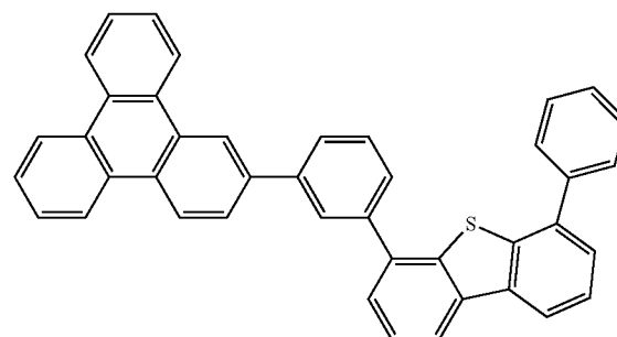
Compound E8
