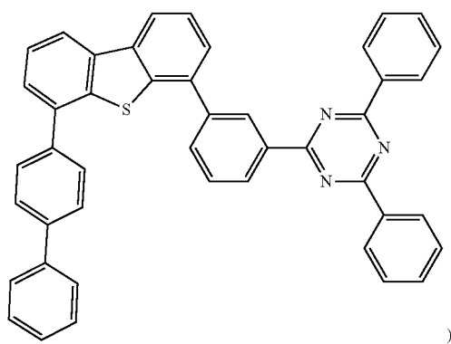
Compound E26
