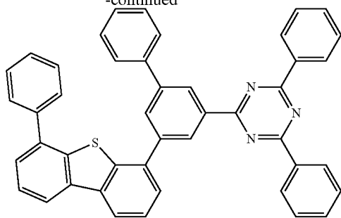
Compound A11
