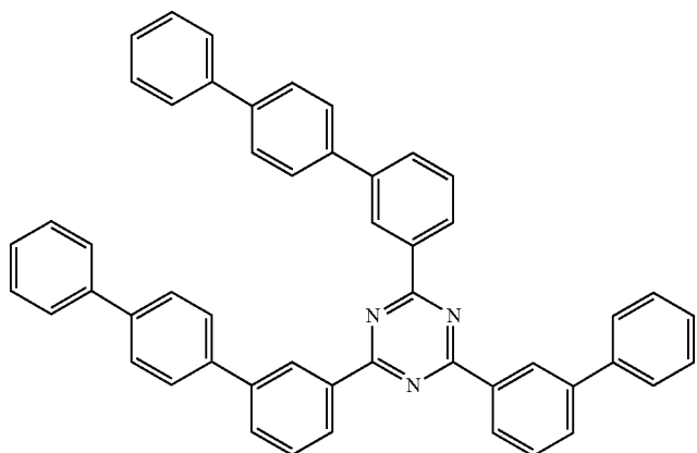
Compound F2
