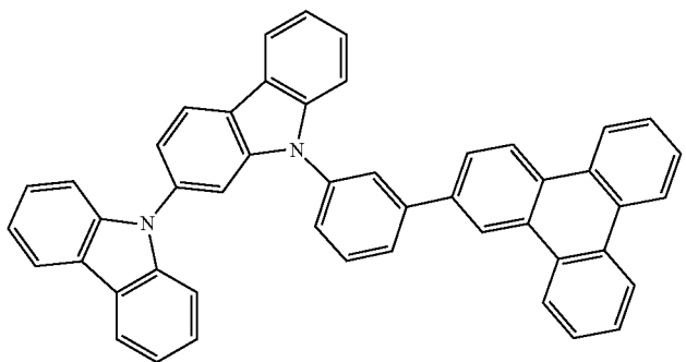
Compound G16
