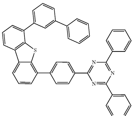
Compound C110
