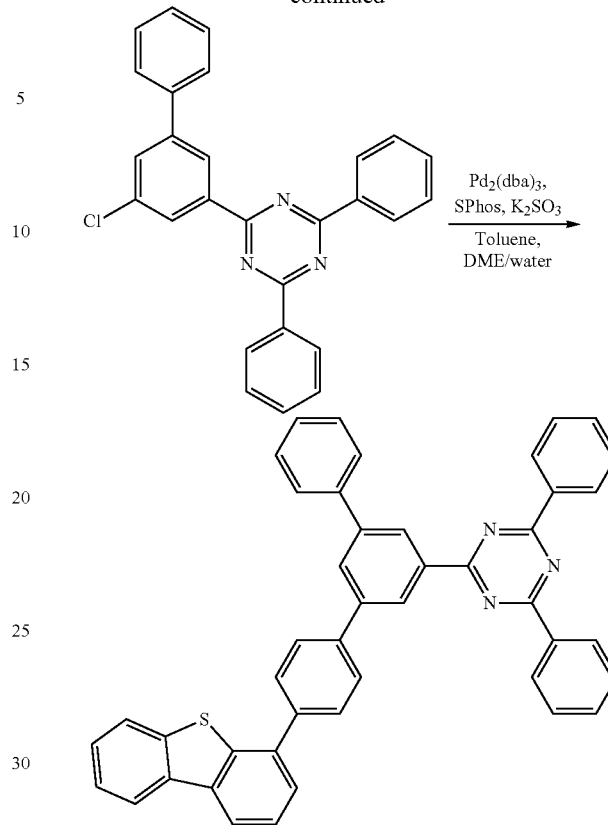
Compound A113
