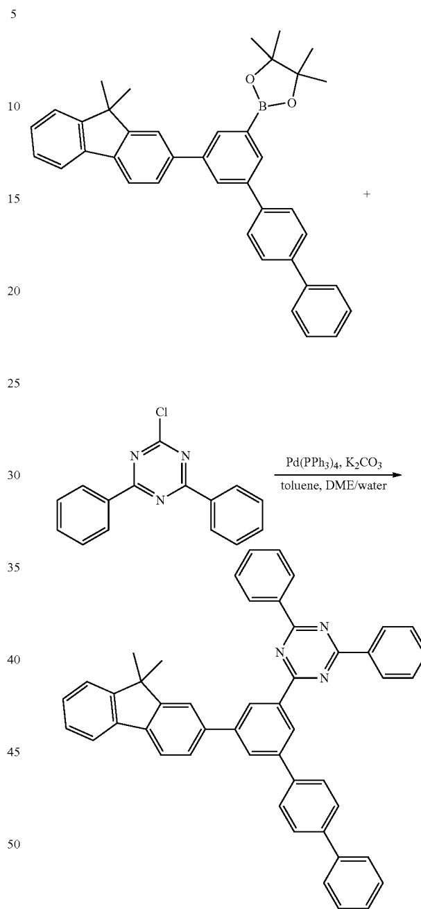
Compound B3
