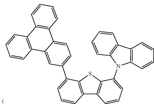
Compound C74
