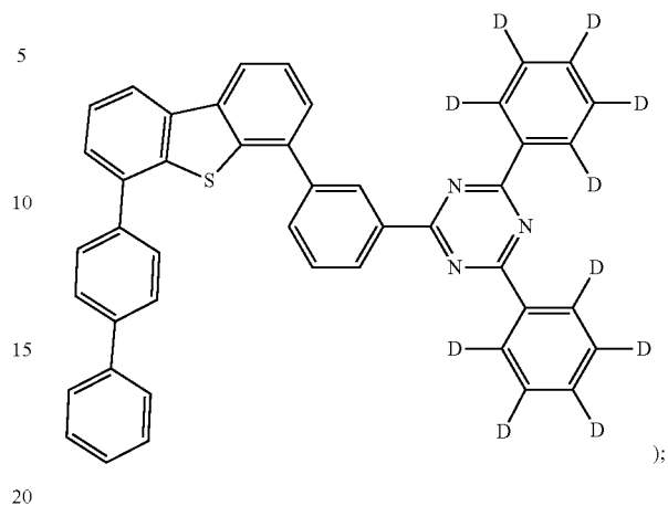
Compound C248
