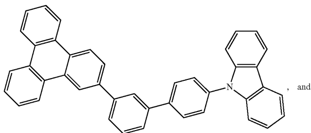
Compound E29
