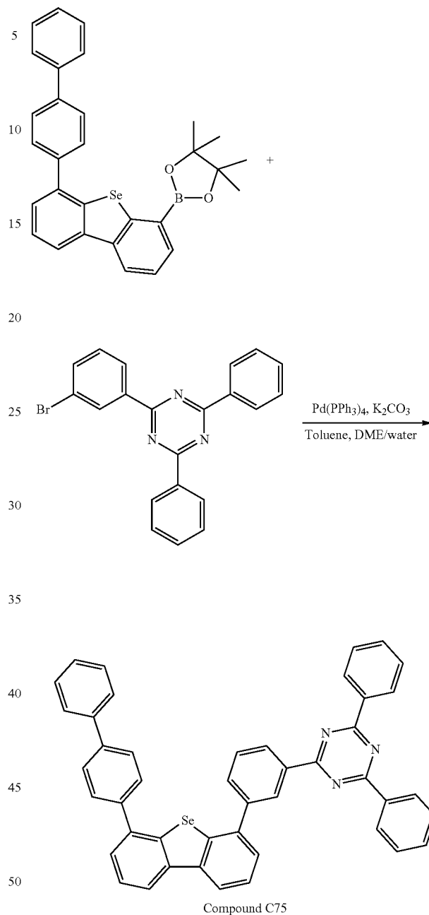
Compound C75
