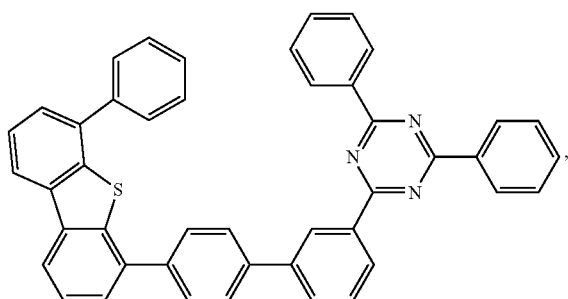
Compound C71
