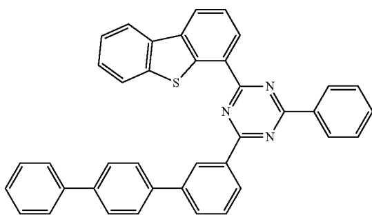
Compound F7
