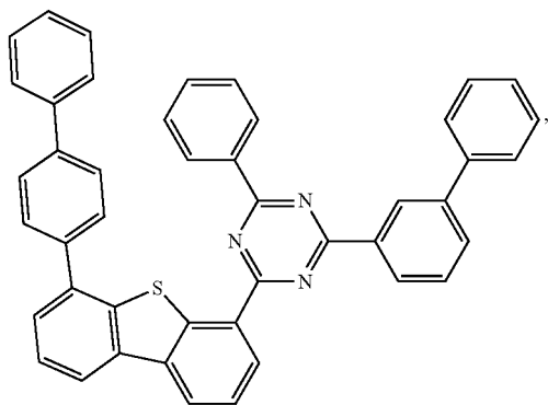
Compound C83
