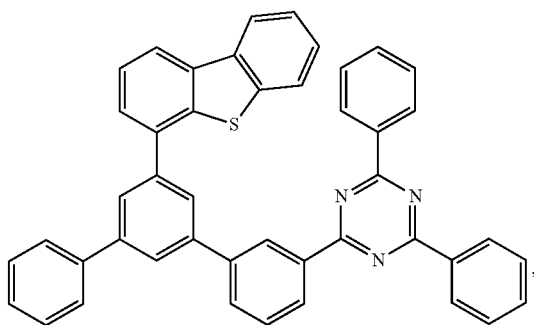
Compound A110
