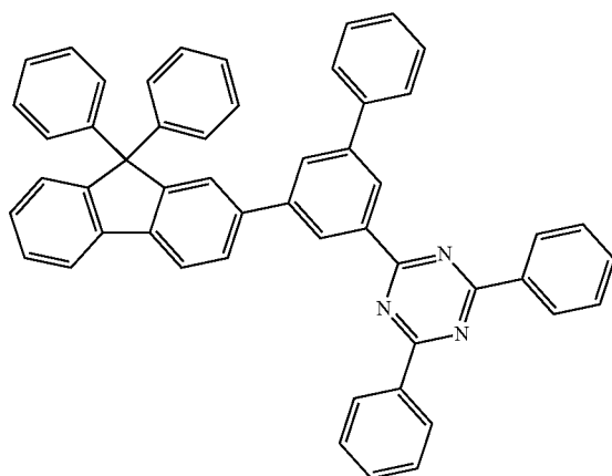
Compound B4
