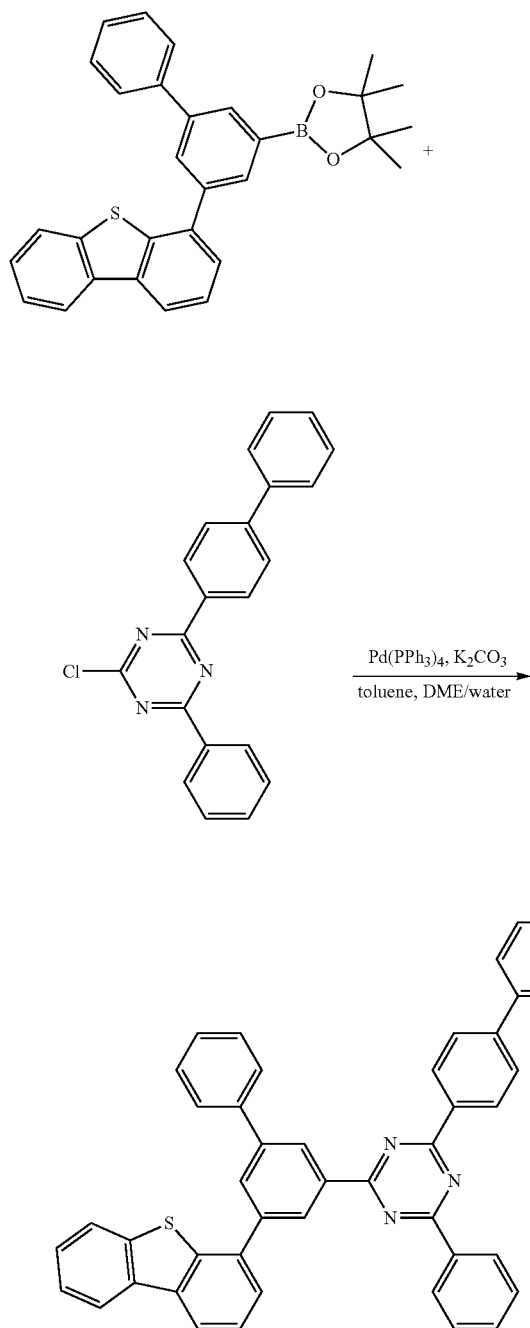
Compound A32
