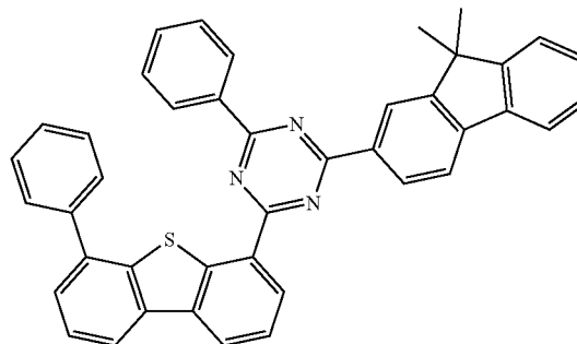
Compound C119
