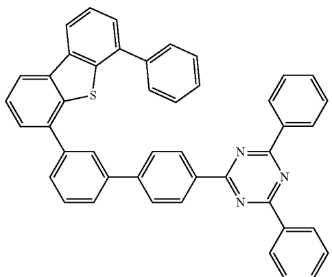
Compound C56
