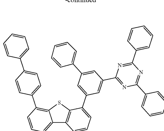
Compound A14
