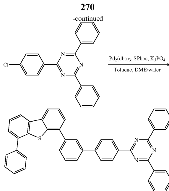
Compound C47
