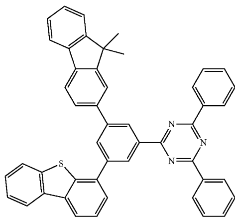
Compound A116
