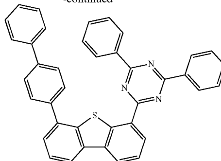
Compound C65
