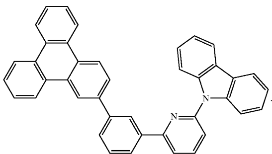
Compound E30
