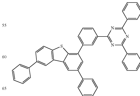
Compound C173
