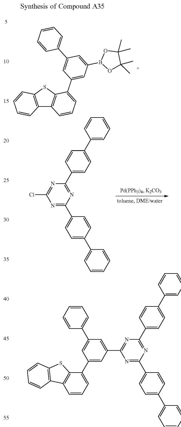
Compound A35
