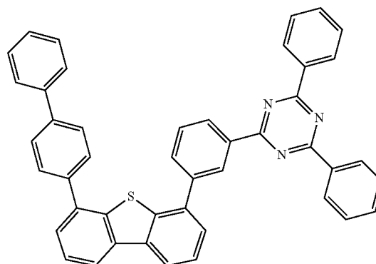
Compound C74
