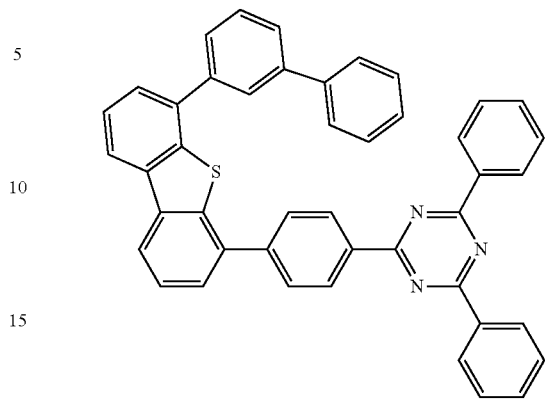
Compound C119
