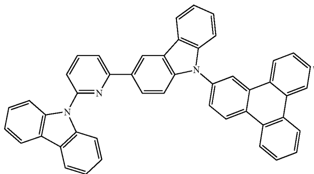
Compound G10
