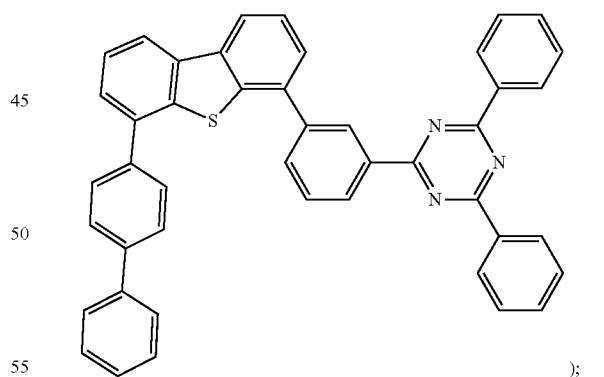
Compound E29
