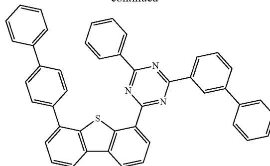
Compound C71
