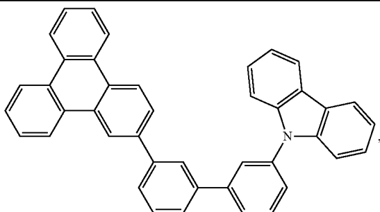
Compound E28
