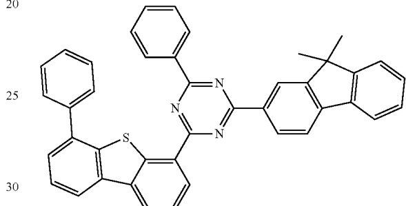
Compound C134
