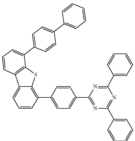
Compound C83
