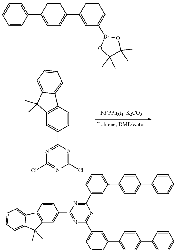
Compound F4
