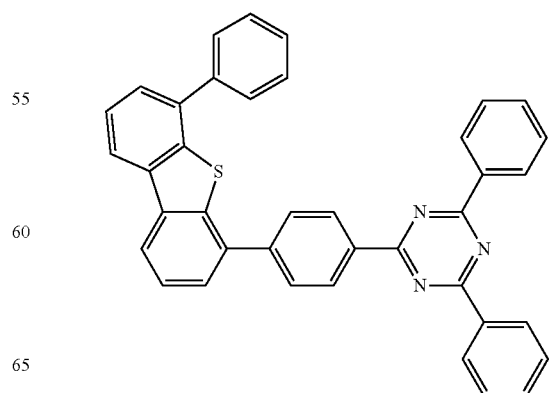
Compound C29
