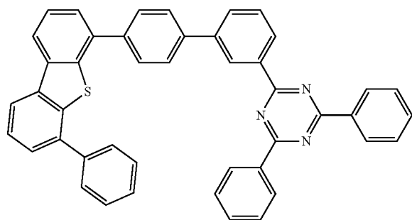
Compound C56
