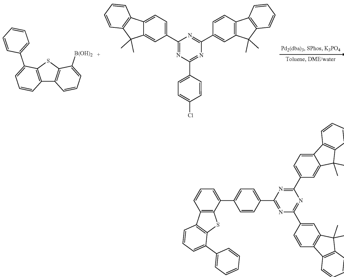
Compound C131
