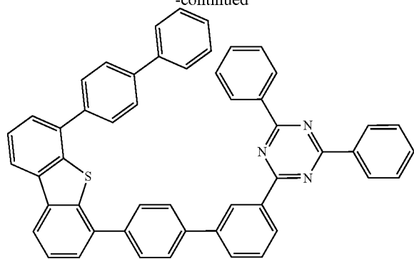
Compound C251
