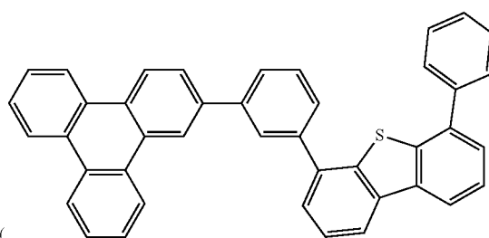
Compound E8
