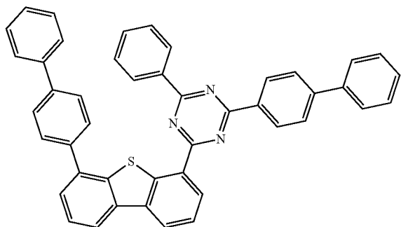
Compound C68
