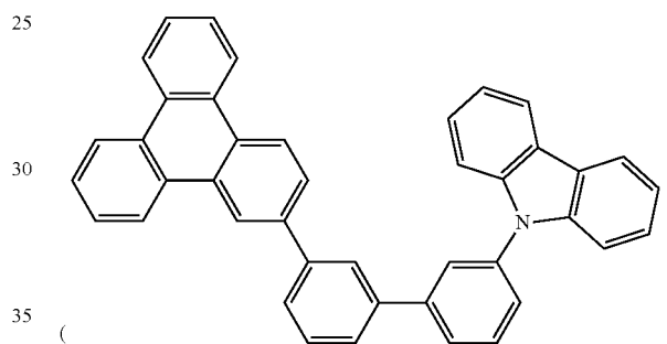
Compound E28
