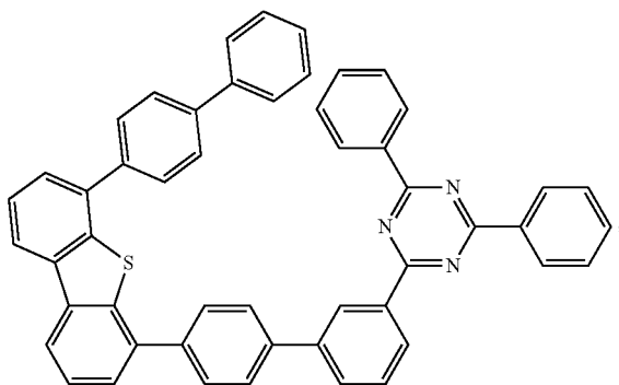
Compound F4
