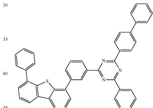
Compound C23
