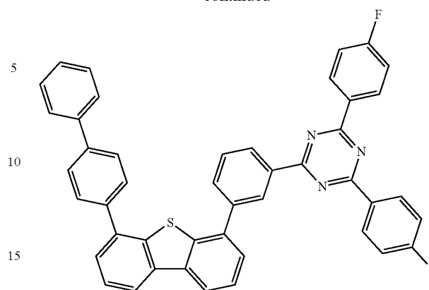
Compound C254
