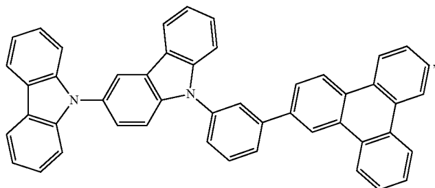
Compound G15
