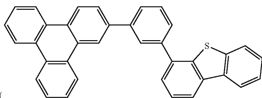
Compound E5
