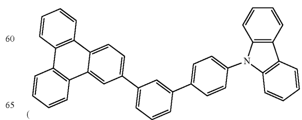
Compound E29
