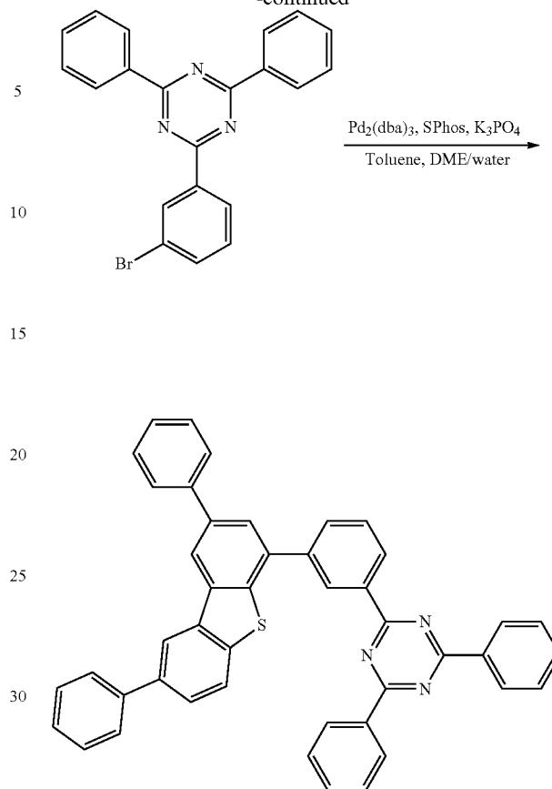
Compound 173
