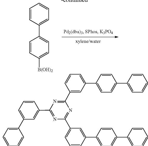
Compound F2
