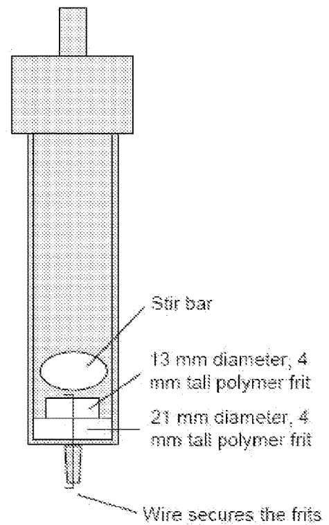
Reaction Tube
