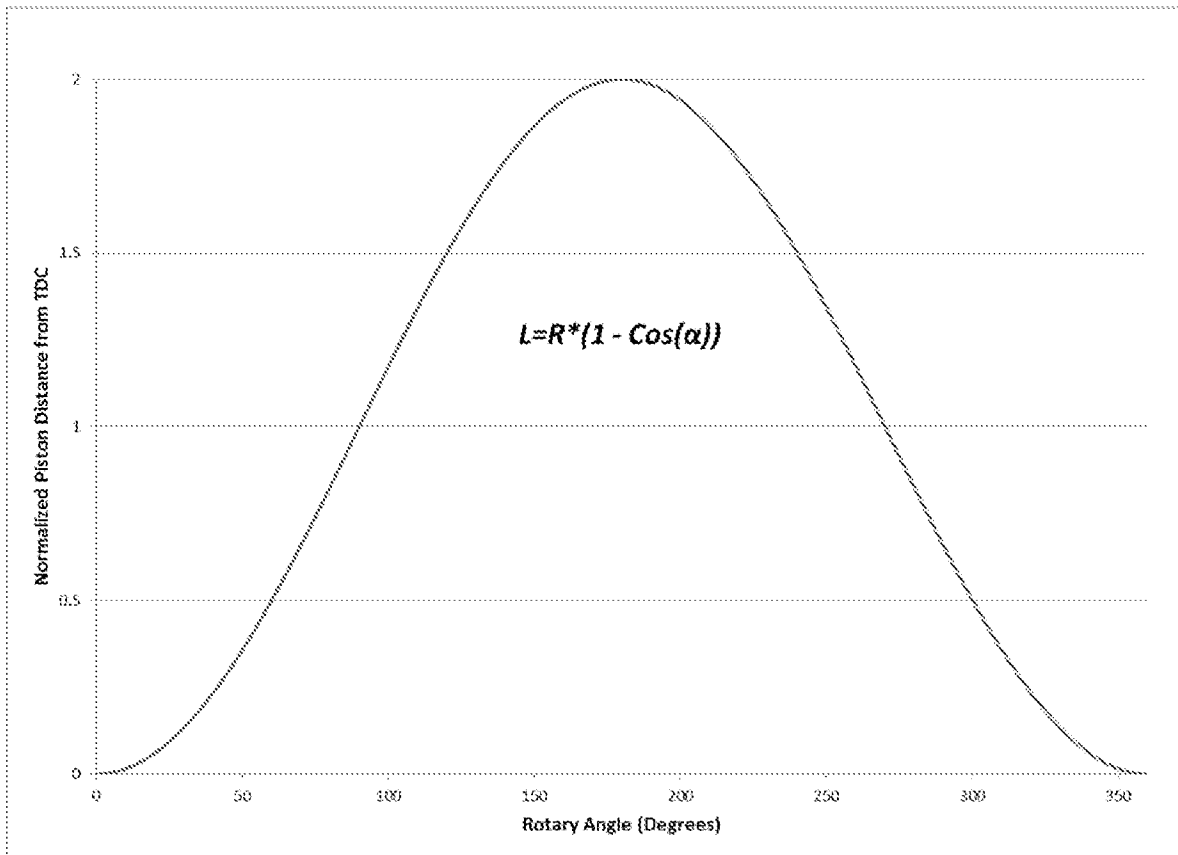
LPEG Piston Position vs Resolver Angle
