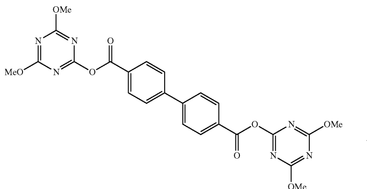
DCPT
