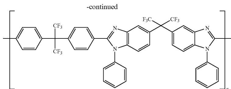
PBI(HPBT-PhTA)
