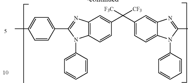
PBI(TPBT-PhTA)
