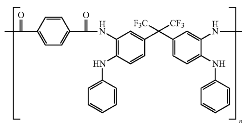
PA(TPBT-PhTA)
