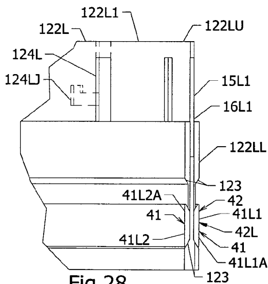
Fig.28 DETAIL M
