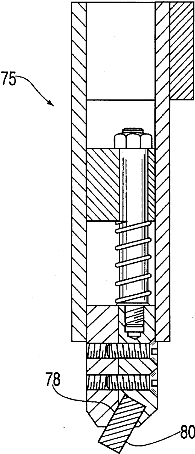
FIG. 2 (PRIOR ART)
