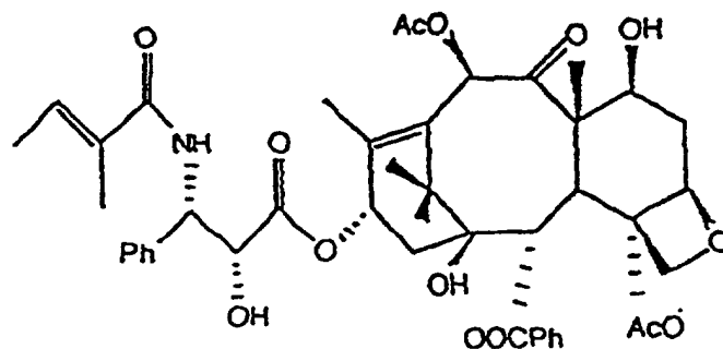
(b) Cephalomannine
