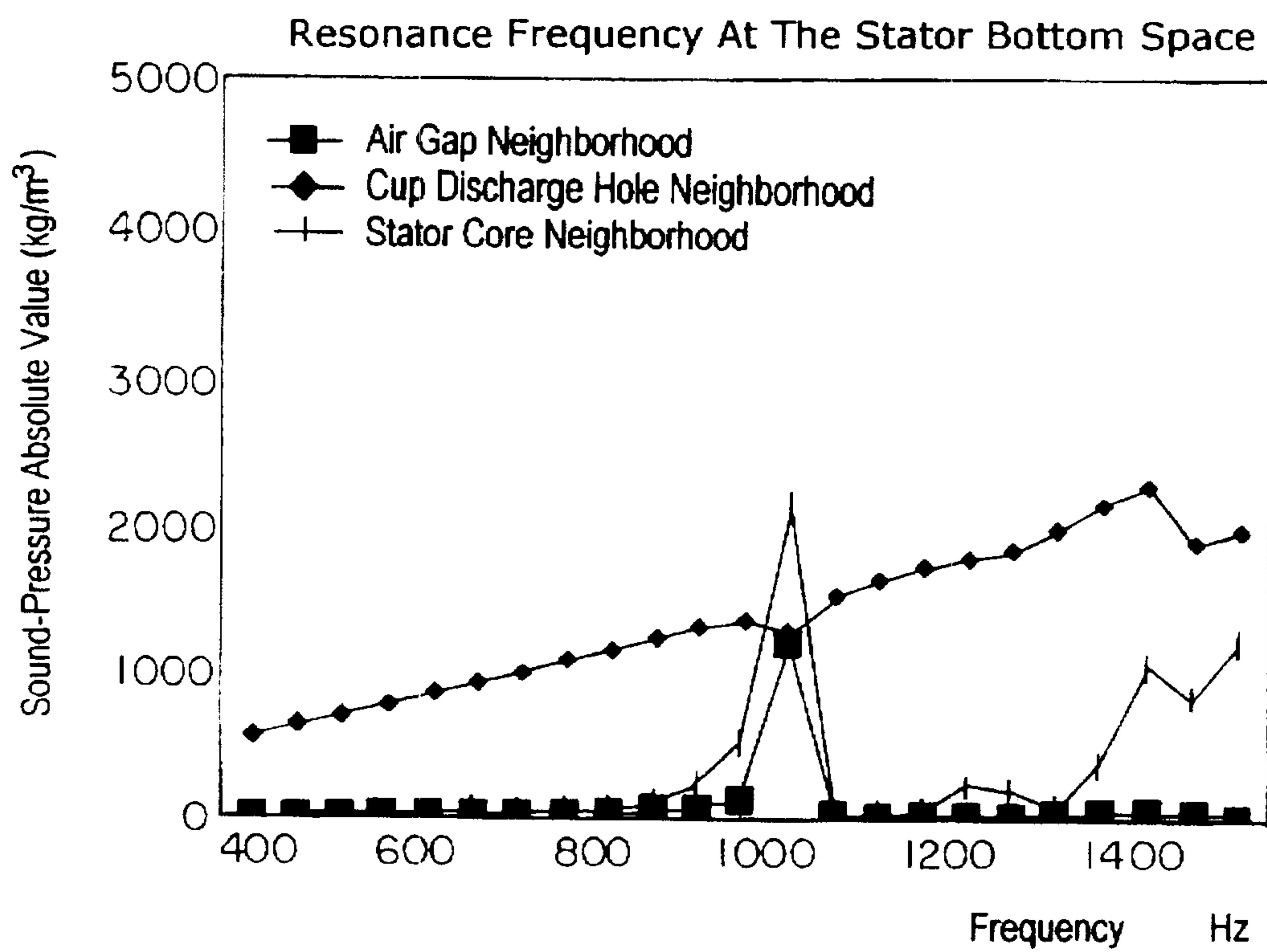
Fig. 10 Prior Art
