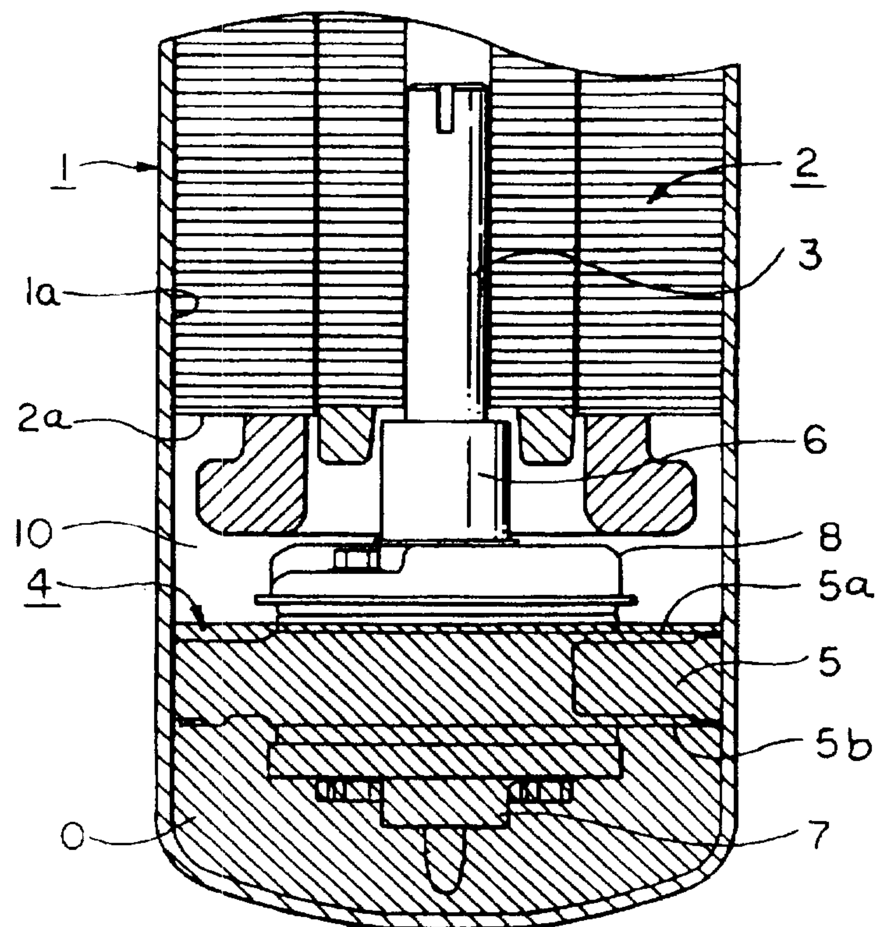
Fig. 6 Prior Art
