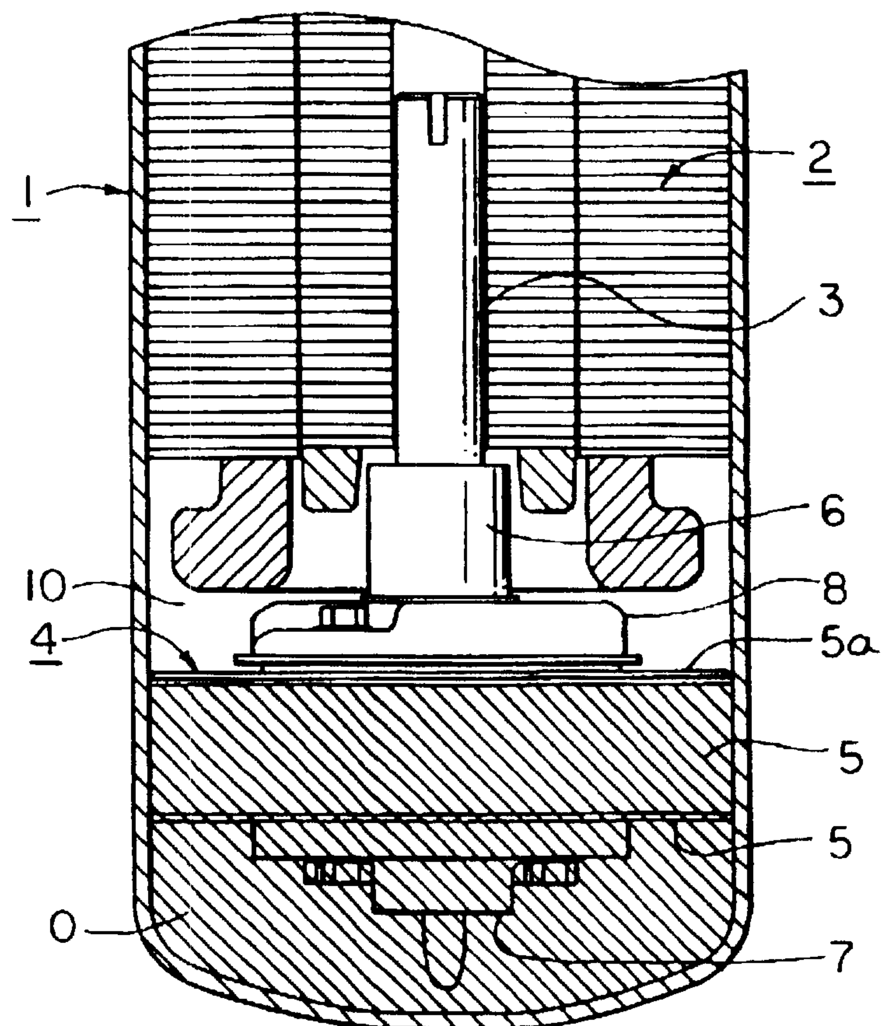
Fig. 8 Prior Art
