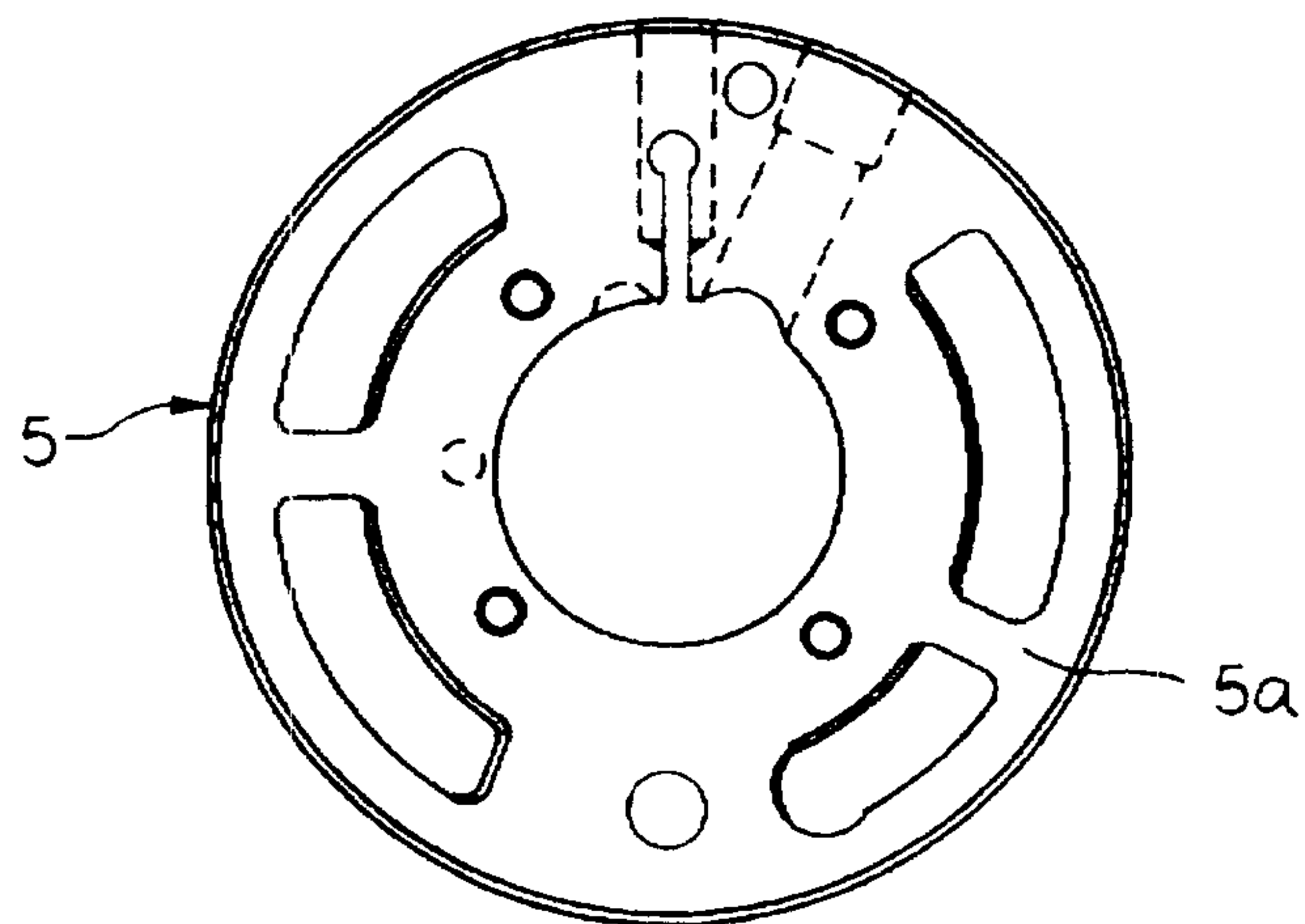
Fig. 9 Prior Art
