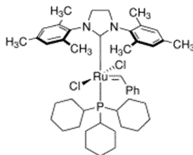
2 nd Gen. Grubbs Catalyst 1,3-Bis-(2,4,6-trimethylphenyl)-2-(imidazolidinylidene)(dichlorophenylmethylene)(tricyclohexylphosphine)ruthenium
