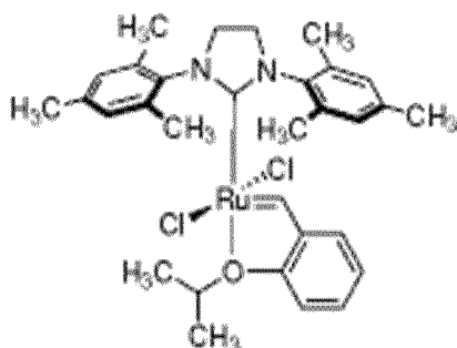
2 nd Gen. Hoveyda-Grubbs Catalyst (1,3-Bis-(2,4,6-trimethylphenyl)-2-imidazolidinylidene)dichloro(o-isopropoxyphenylmethylene)ruthenium
