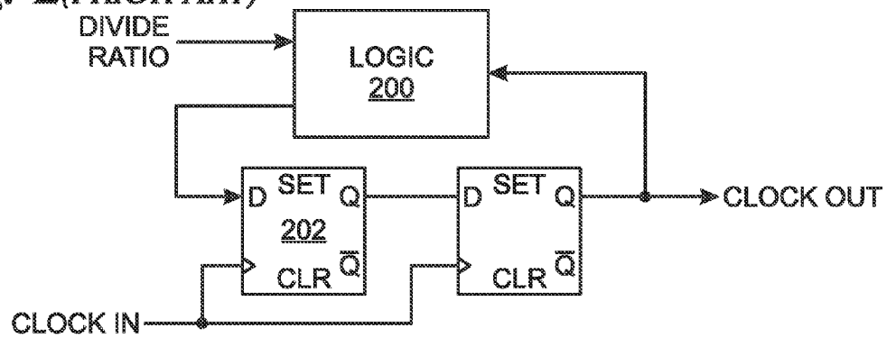
Fig. 2(PRIOR ART)
