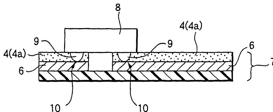
FIG.1E BORDING PROCESS
