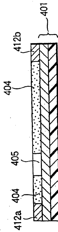
FIG.8B ETCHING MASK PRINTING PROCESS
