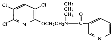
N-(n-propyl), N-(3-pyridylcarbonyl)ethanolamine 3,5,6-trichloropyridylether
