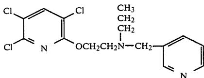
N-(n-propyl), N-(3-picoly)ethanolamine 3,5,6-trichloropyridylether
