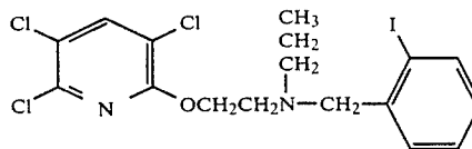
N-(n-propyl), N-(2-iodobenzoyl)ethanolamine 3,5,6-trichloropyridylether
