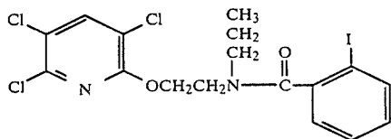
N-(n-propyl), N-(2-iodobenzoyl) ethanolamine 3,5,6-trichloropyridylether
