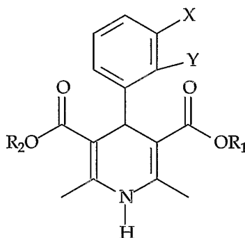
Formula VIII
