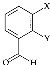
Formula II
