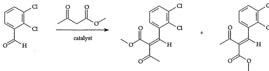
Scheme 4
