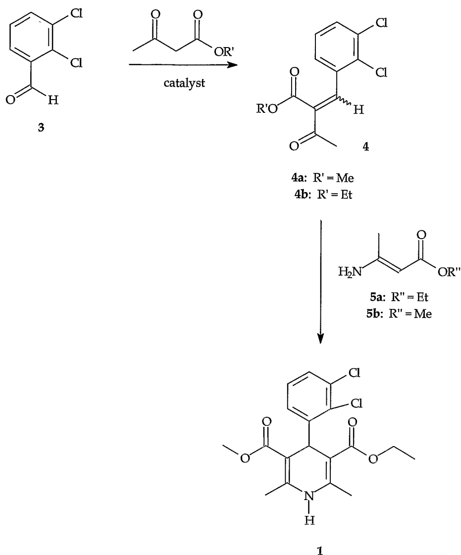
Scheme 1
