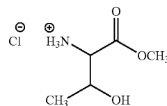
L-threonine methyl ester, hydrochloride
