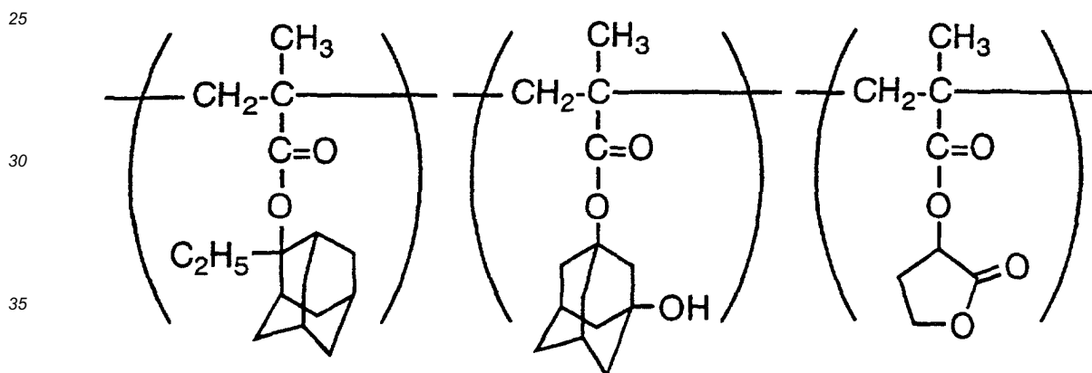
Synthesis Example 3 for Resin (Synthesis of resin A3)
