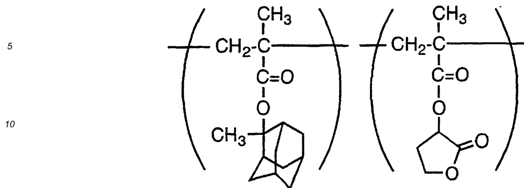
Synthesis Example 2 for Resin (Synthesis of resin A2)
