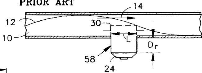
FIG. 4 PRIOR ART
