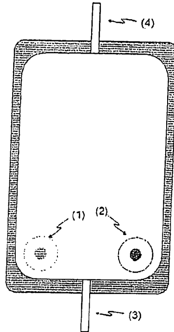
Figure 5b. Reservoir design 5b.
