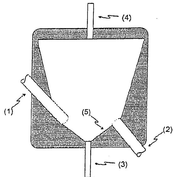
Figure 7. Reservoir design 7. Placement of (2) is arbitrary.
