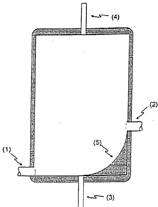
Figure 6. Reservoir design 6.
