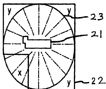
PRIOR ART FIG. 1c
