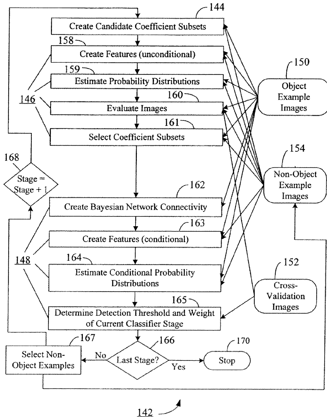
System for building Bayesian Network based classifier
