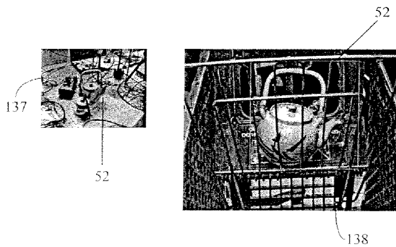
FIG. 32 Teapot Detection
