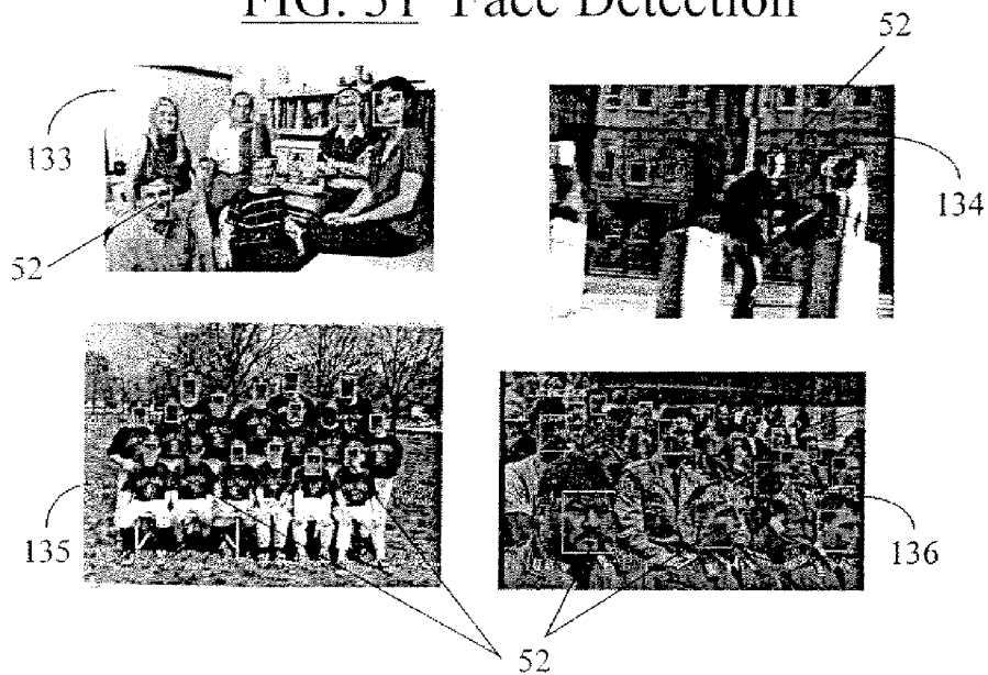
FIG. 31 Face Detection
