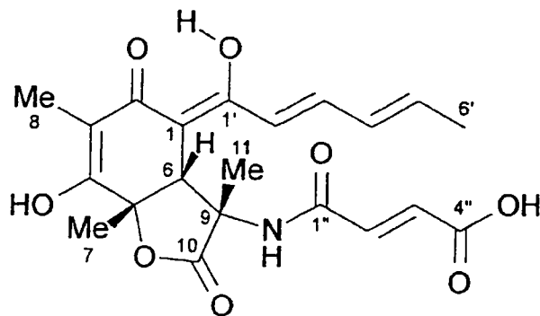
Sorbicillacton A
