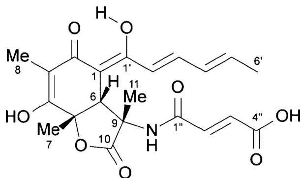
Sorbicillacton A
