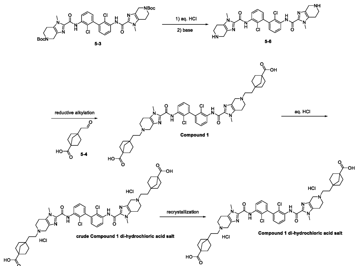
Scheme 8
