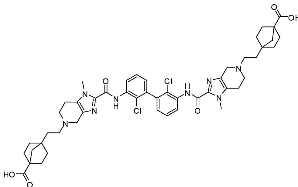
Compound 1
