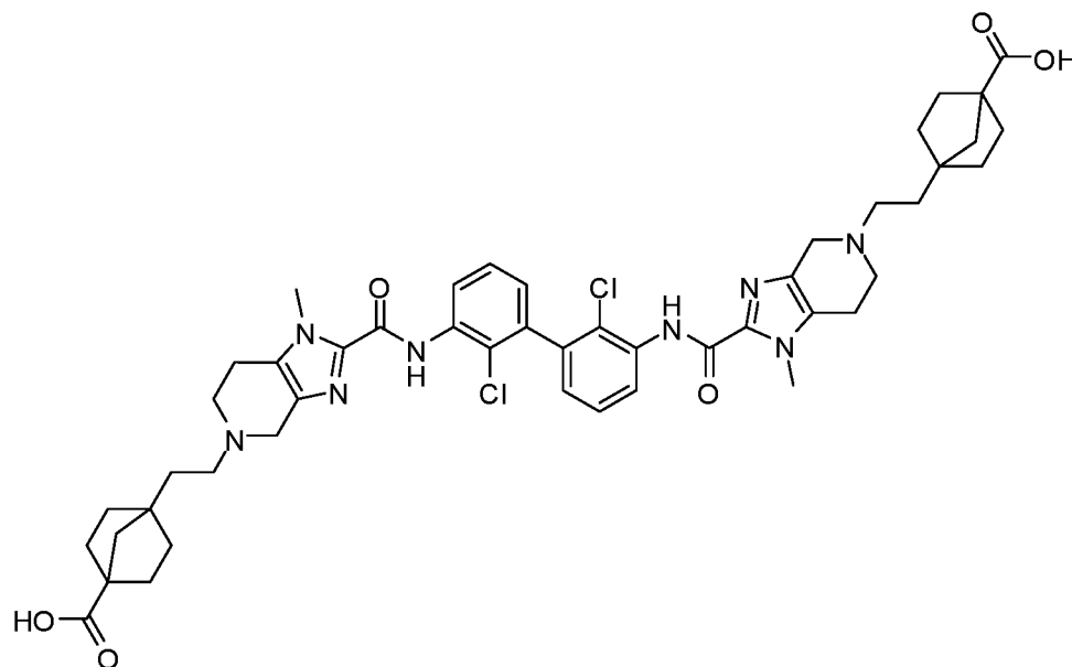
(Compound 1)
