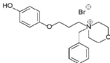
Compound 53A
