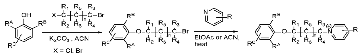
Scheme C:
