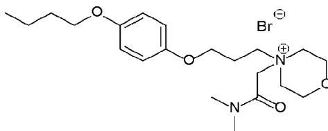
Compound 54A
