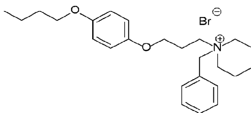
Compound 38A
