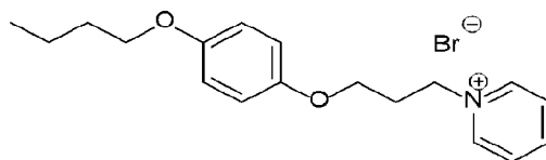
Compound 44A
