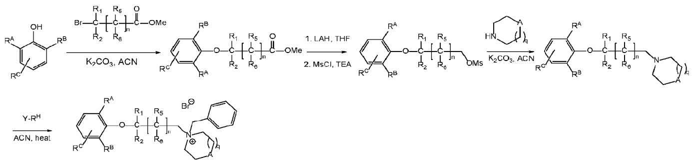
Scheme D:
