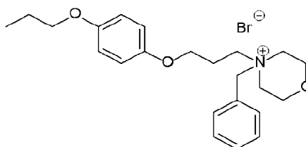
Compound 47A
