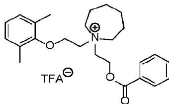
Compound 35A
