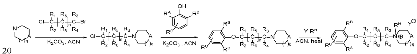
Scheme B:
