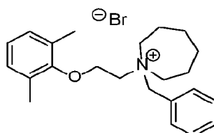
Compound 1A
