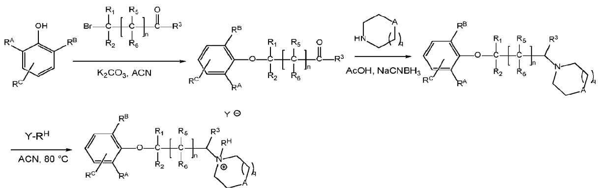
Scheme E:
