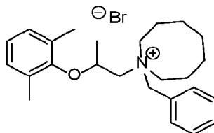
Compound 34A
