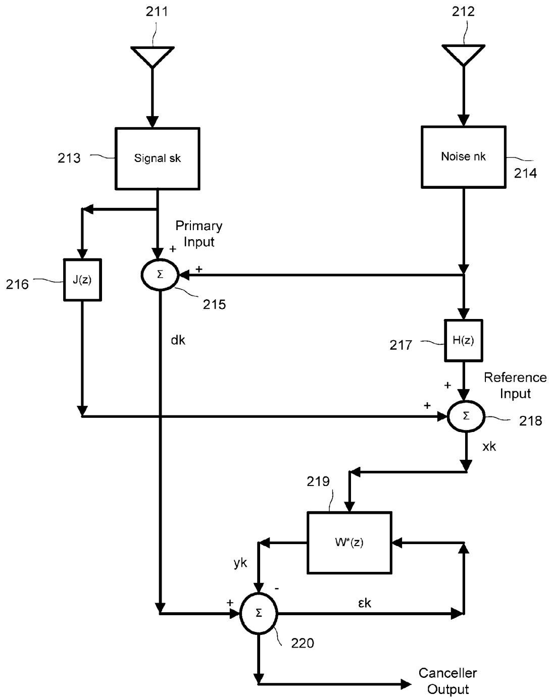
FIG. 2 PRIOR ART
