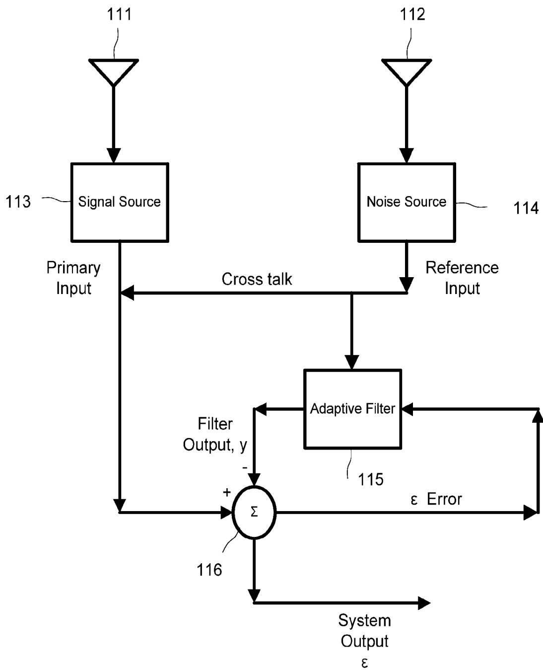
FIG. 1 PRIOR ART
