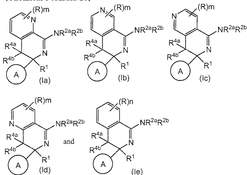
[Chemical Formula 23]
