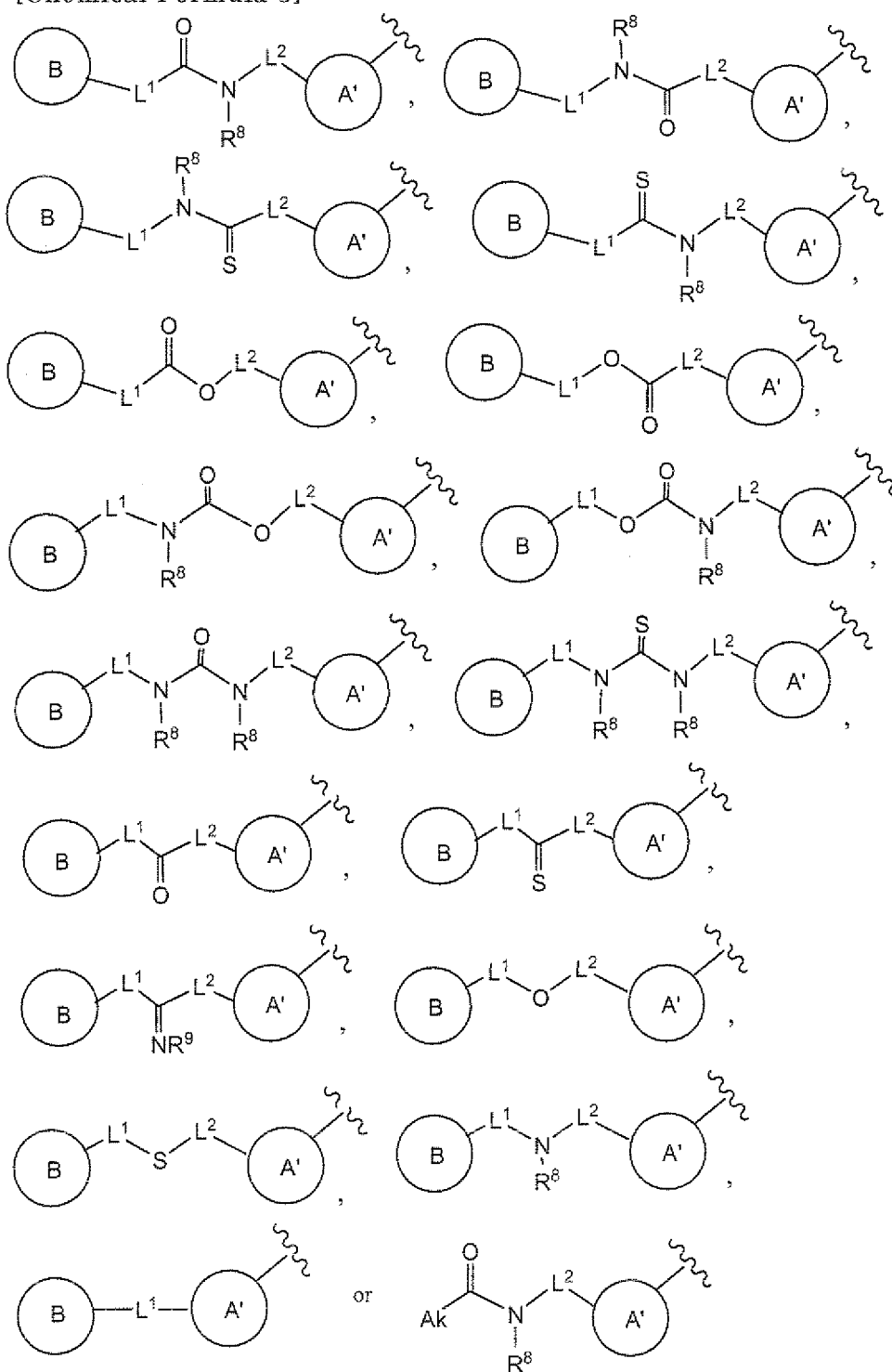
[Chemical Formula 3]
