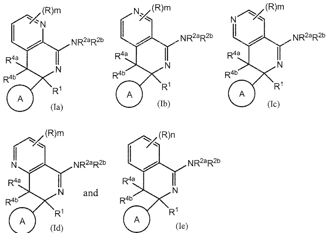
[Chemical Formula 14]
