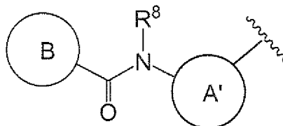
[Chemical Formula 32]
