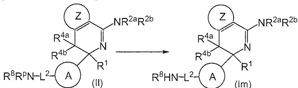
[Chemical Formula 20]
