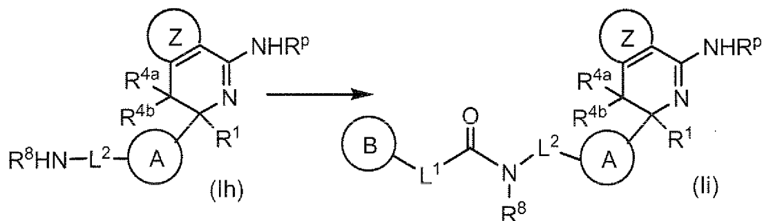
[Chemical Formula 18]
