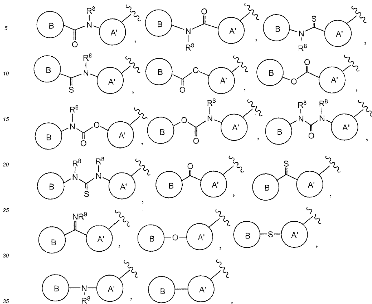
[Chemical Formula 8]
