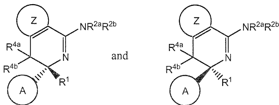
[Chemical Formula 12]
