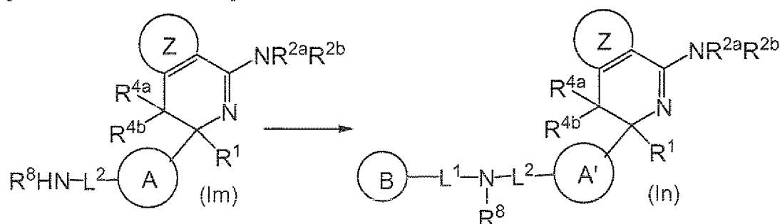
[Chemical Formula 21]
