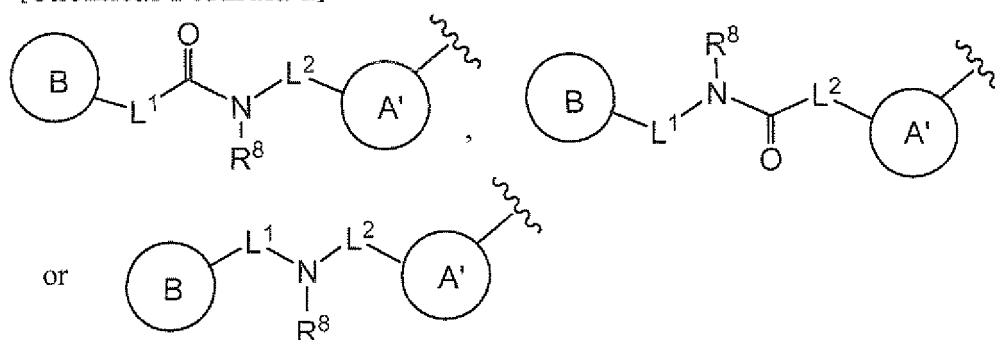
[Chemical Formula 2]
