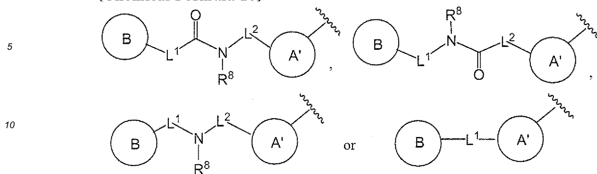
[Chemical Formula 25]
