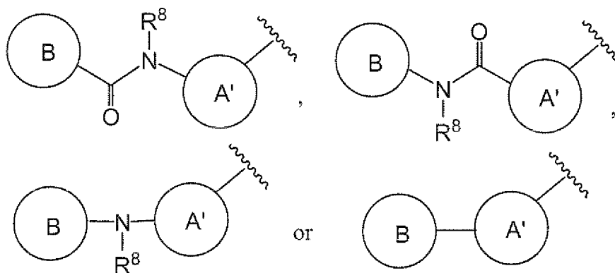
[Chemical Formula 31]
