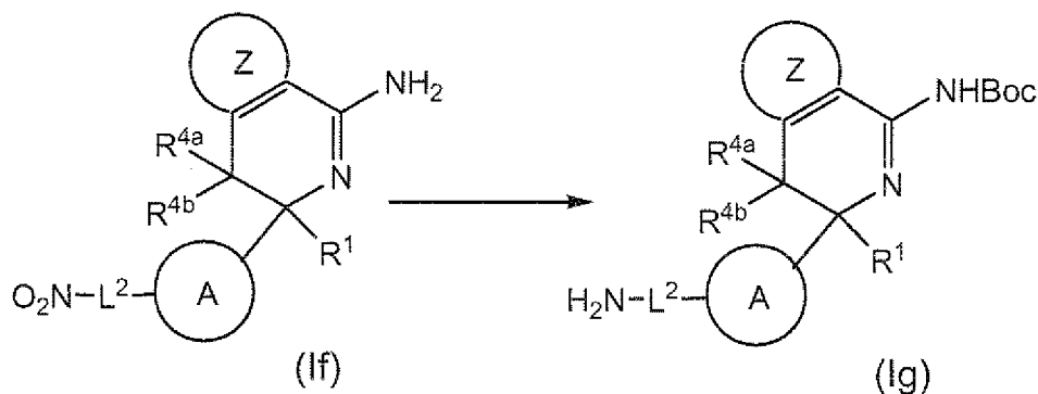
[Chemical Formula 17]
