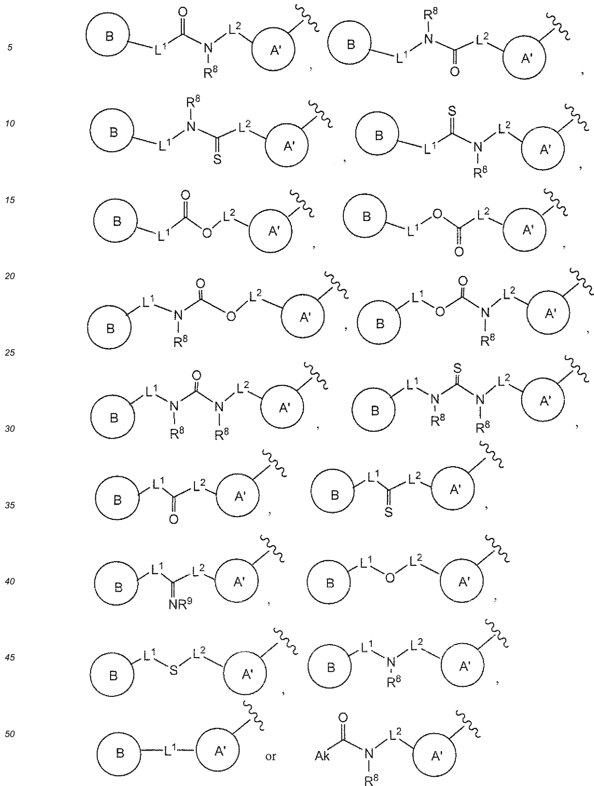
[Chemical Formula 24]
