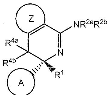
[Chemical Formula 13]
