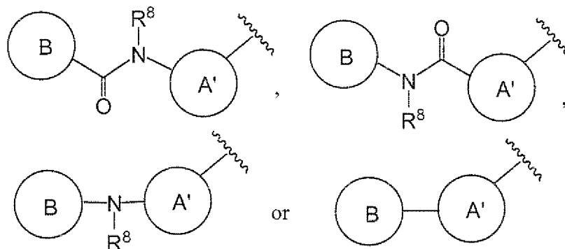
[Chemical Formula 30]
