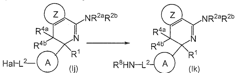
[Chemical Formula 19]
