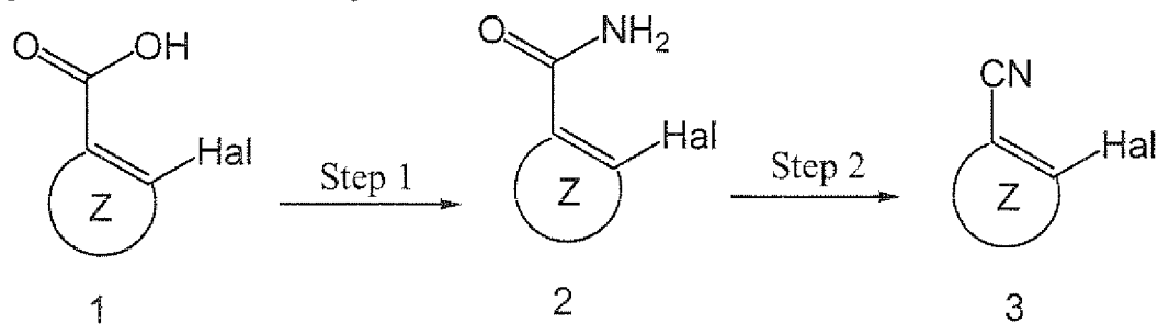
[Chemical Formula 15]
