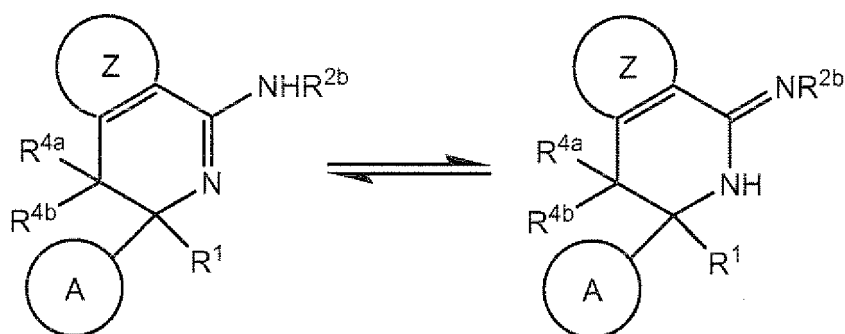
[Chemical Formula 11]
