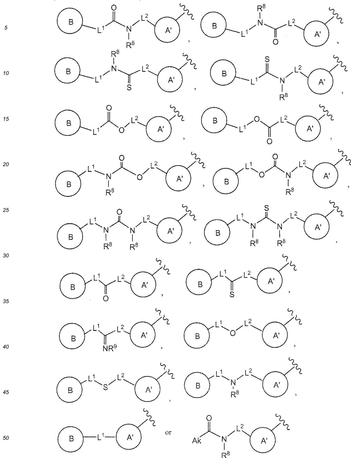
[Chemical Formula 6]
