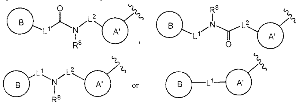
[Chemical Formula 28]
