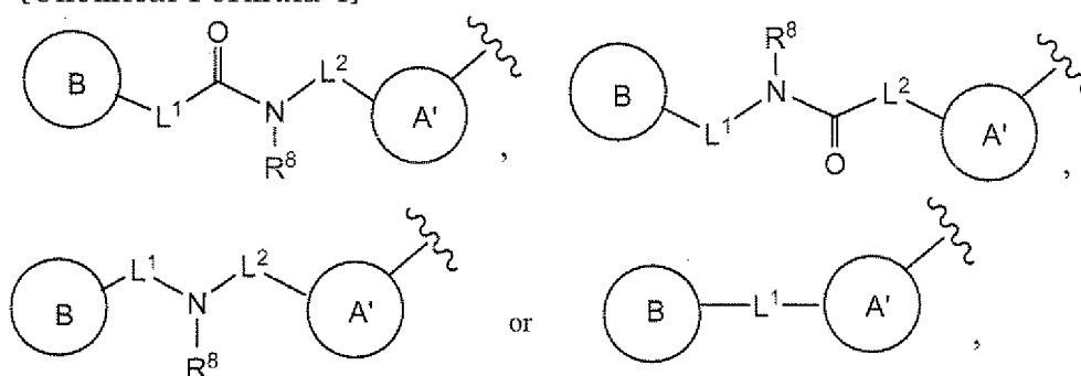
[Chemical Formula 4]
