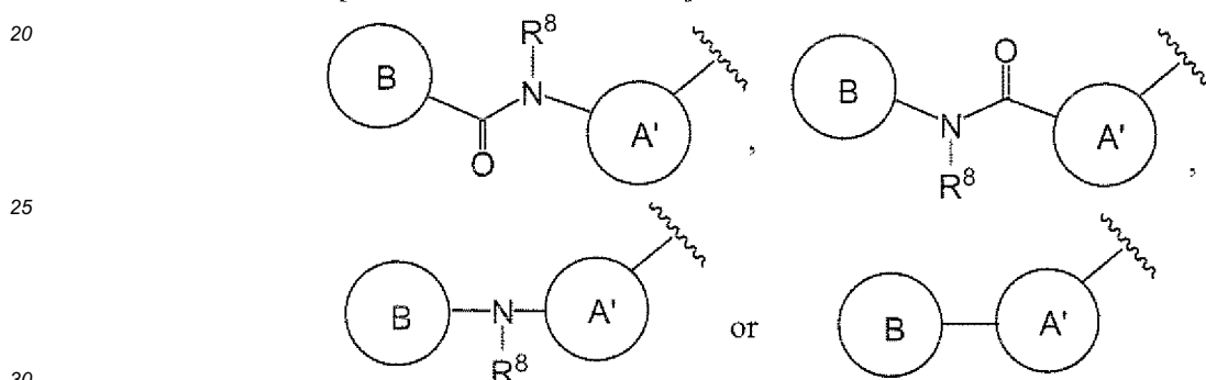
[Chemical Formula 26]
