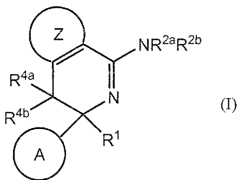
[Chemical Formula 1]
