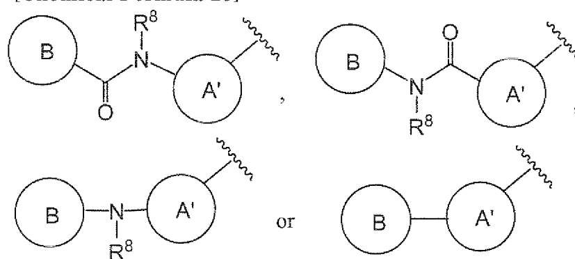
[Chemical Formula 29]
