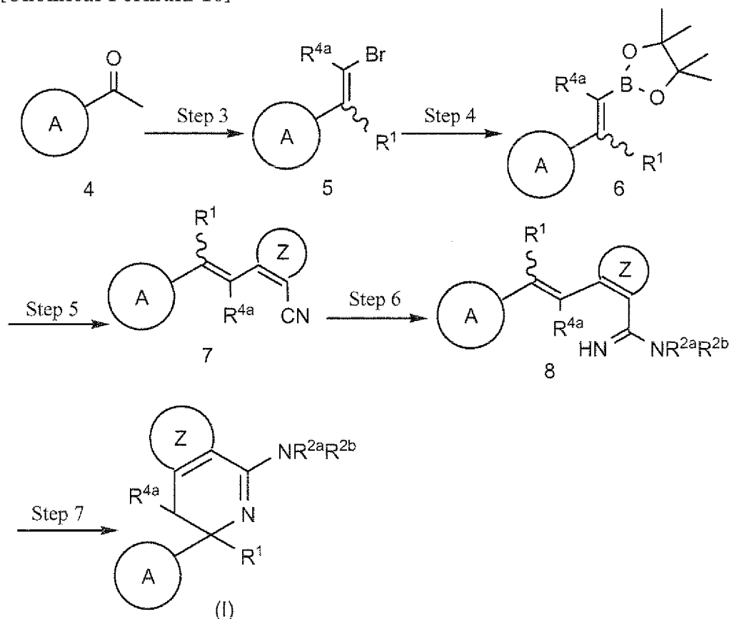
[Chemical Formula 16]
