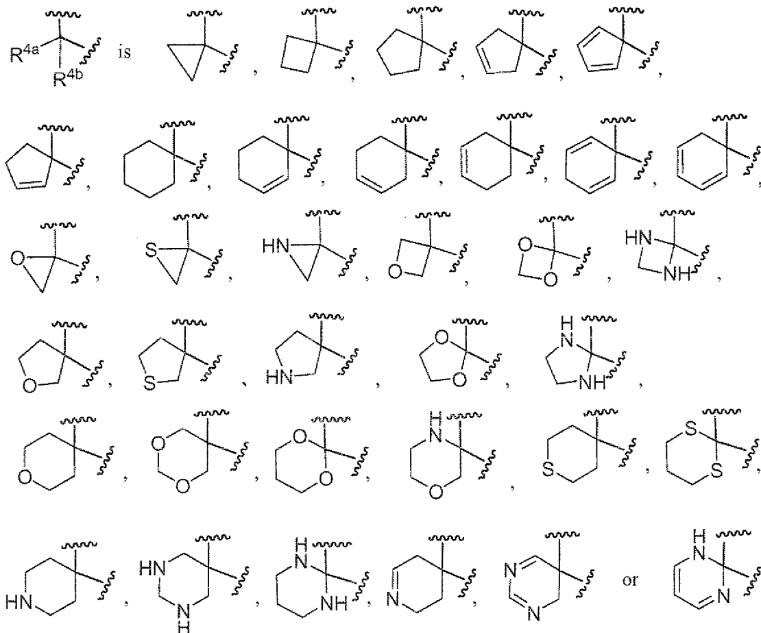
[Chemical Formula 10]
