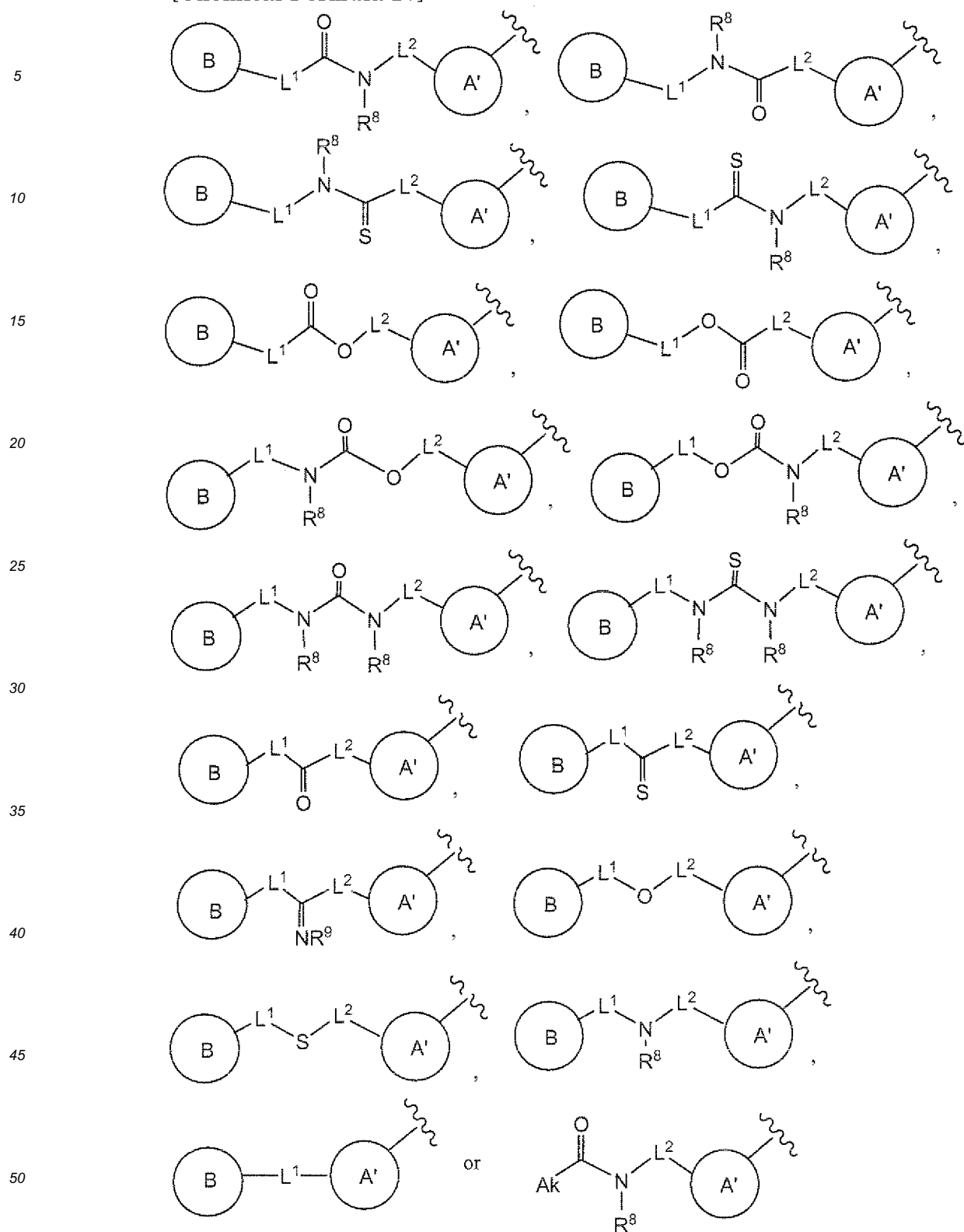
[Chemical Formula 27]
