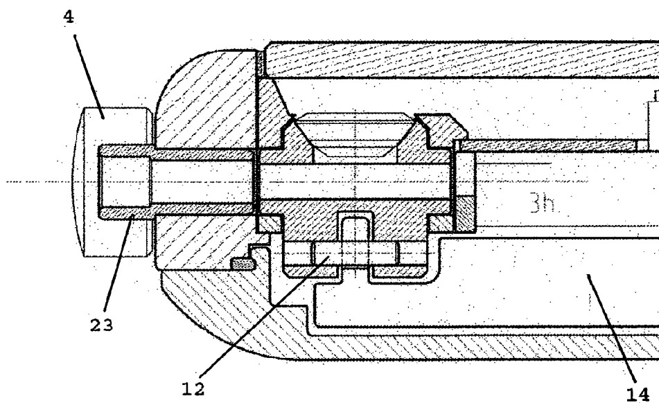
Fig 8 Section D-D
