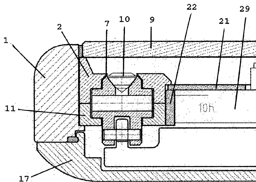
Fig 7 Section C-C
