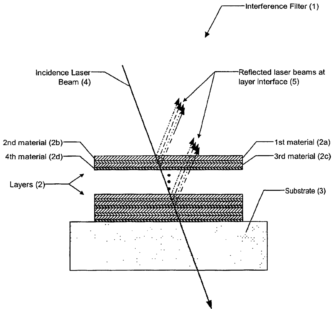
FIG. 1 (background art)
