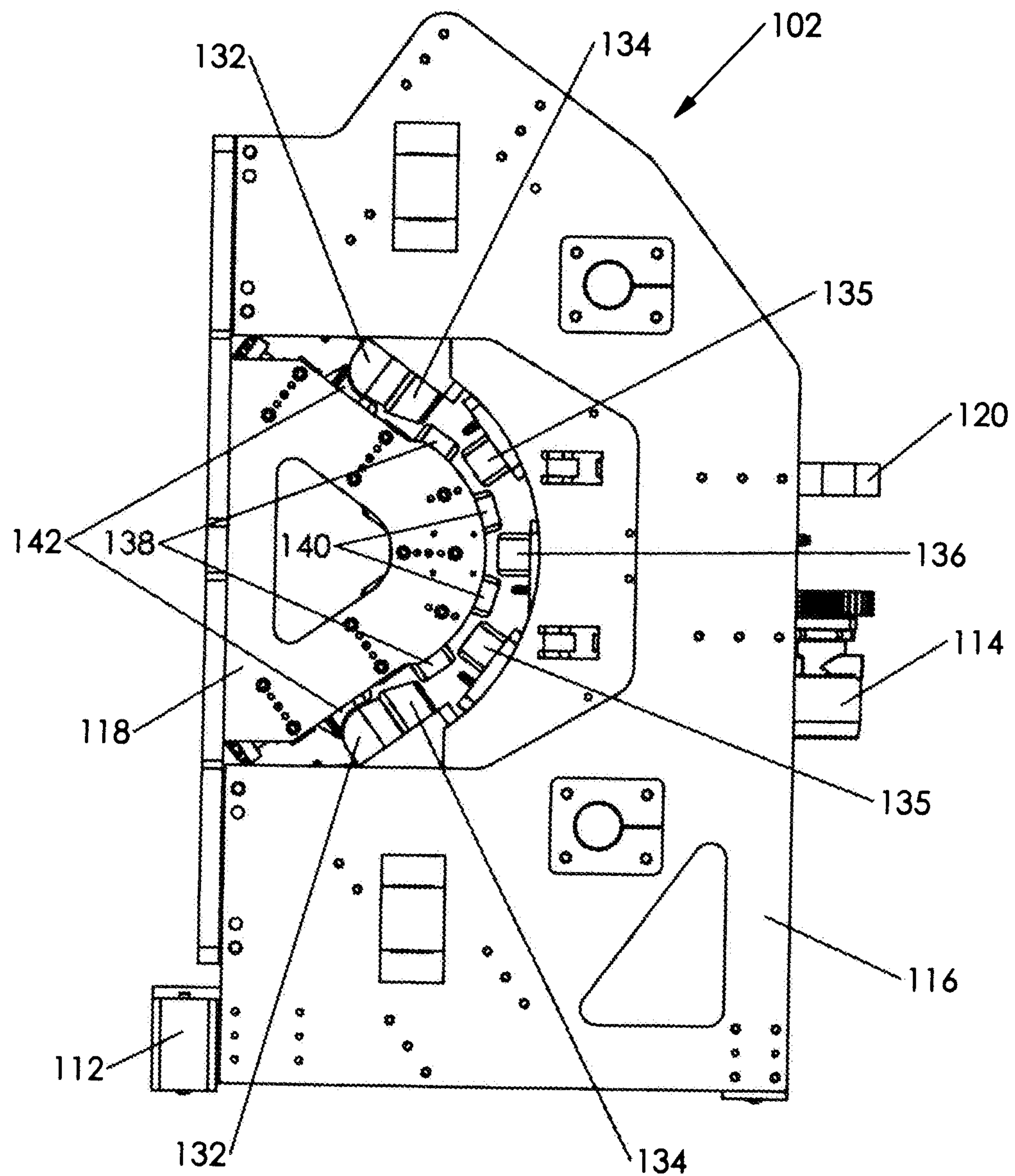
FIG. 10 (Side View)
