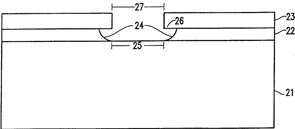
FIG. 2C PRIOR ART
