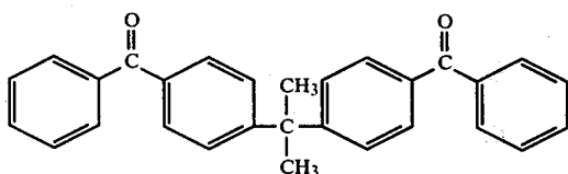
4,4'-isopropylidenedibenzophenone
