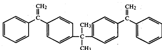
2,2-Bis[4-(1-phenylethenyl)phenyl]propane
