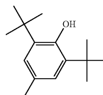
2,6-bis(1,1-dimethylethyl)-4-methylphenol (BHT)
