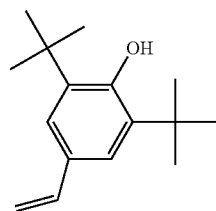
2,6-di-tert-butyl-4-vinylphenol
