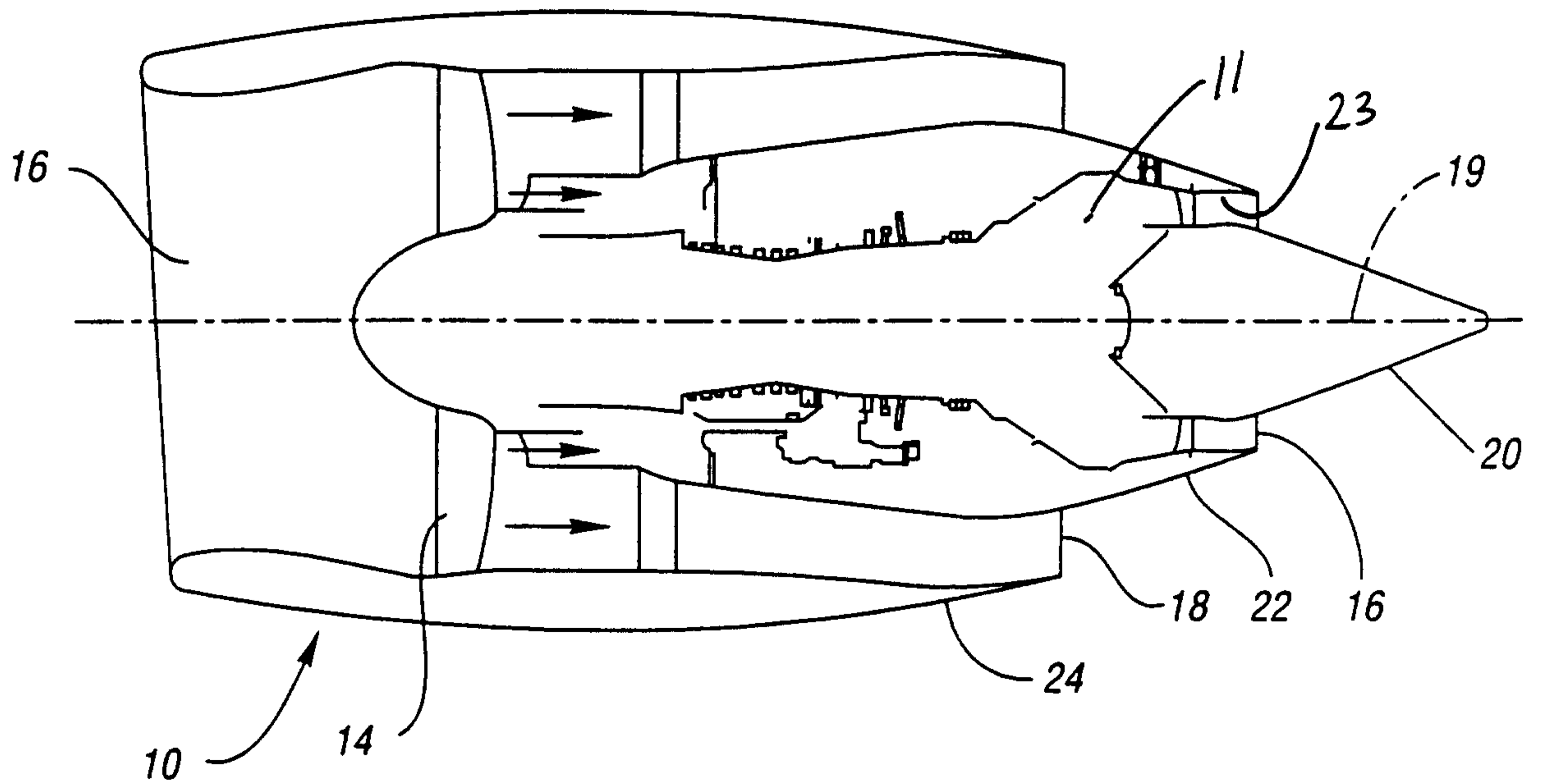
Fig. 2 (PRIOR ART)
