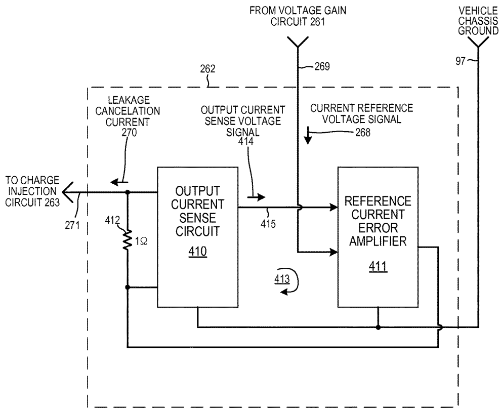
CURRENT CONTROLLED FEEDBACK CIRCUIT FIG. 25
