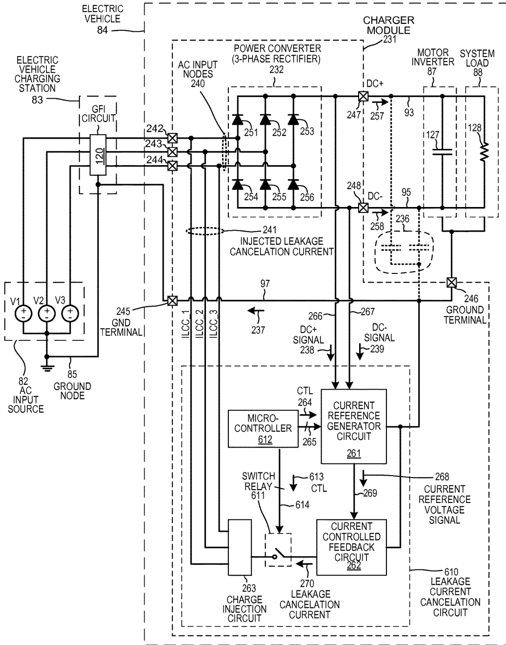
CHARGER MODULE (ANOTHER EMBODIMENT) FIG. 33
