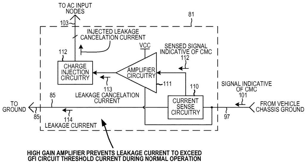
LEAKAGE CURRENT CANCELATION CIRCUIT FIG. 8
