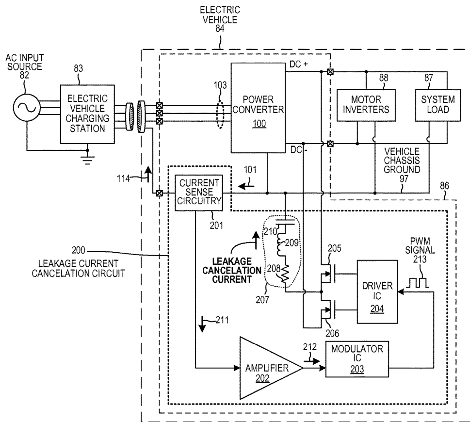
LEAKAGE CURRENT CANCELATION CIRCUIT (ANOTHER EMBODIMENT)
