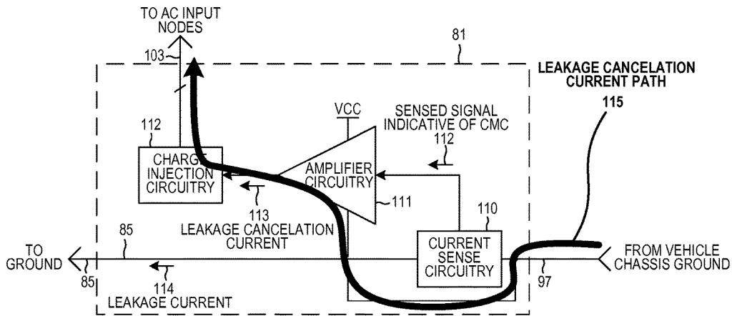
LEAKAGE CURRENT CANCELATION CIRCUIT FIG. 8
