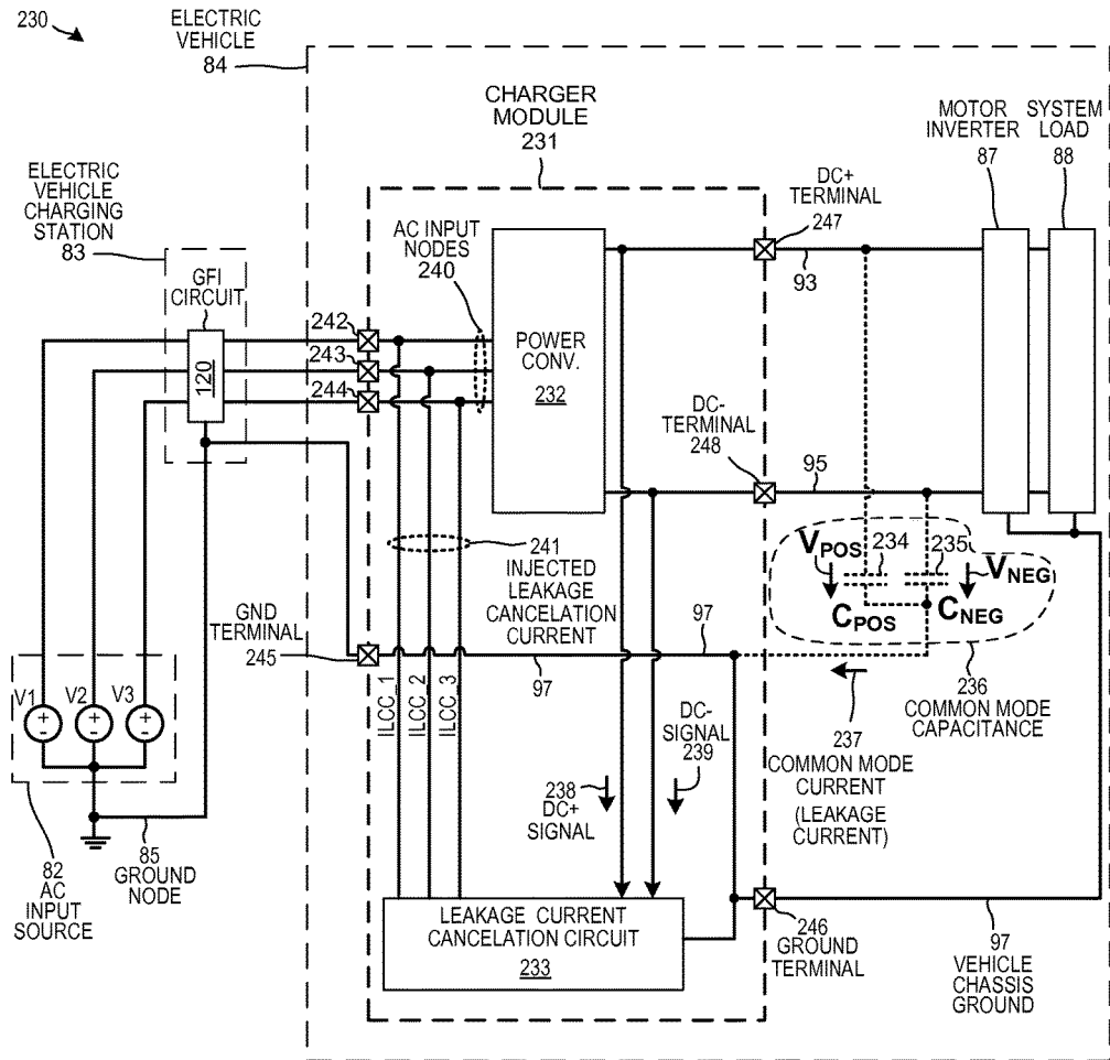
LEAKAGE CURRENT CANCELATION CIRCUIT (ANOTHER EMBODIMENT)
