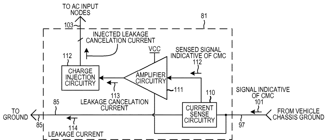
LEAKAGE CURRENT CANCELATION CIRCUIT
